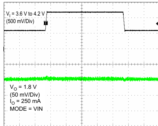
Figure 34. Line Transient (Forced PWM Mode)
