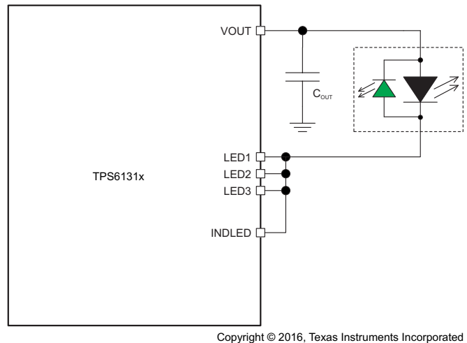
Figure 29. Configuration 2
