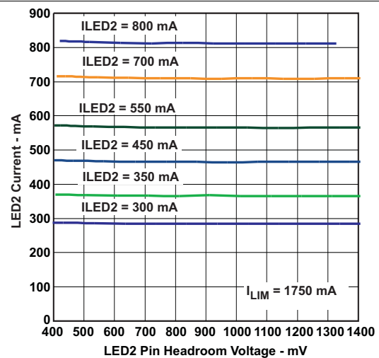
Figure 6. LED2 Current vs LED2 Pin Headroom Voltage
