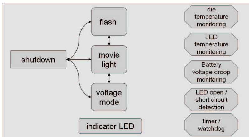
Figure 25. TPS6131x States
