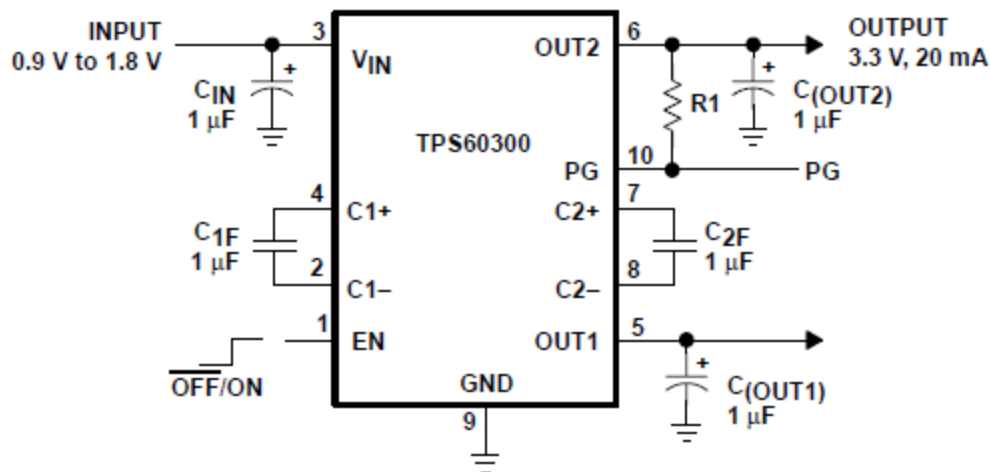
Figure 3. Typical Operating Circuit
