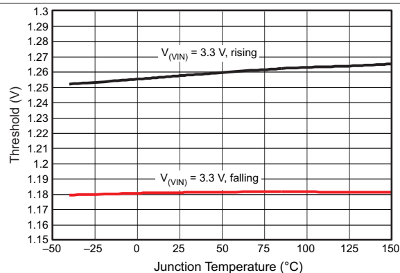
Figure 9. EN Pin Voltage vs Temperature
