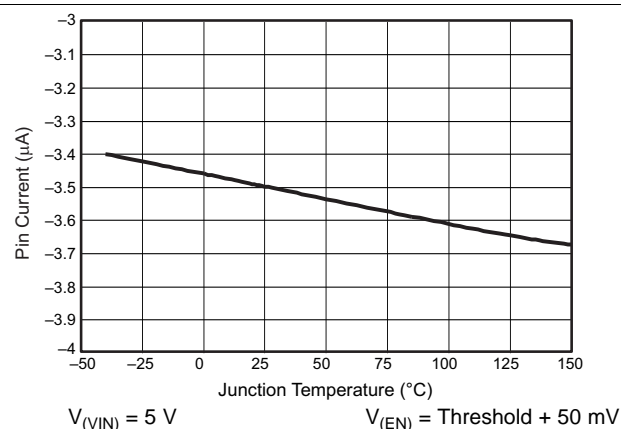
Figure 10. EN Pin Current vs Temperature
