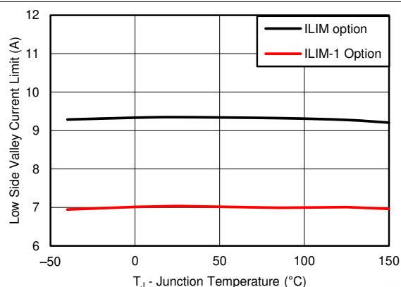
Figure 6-10. Valley Current Limit vs Temperature
