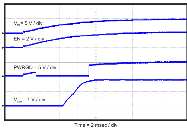
Figure 8-5. Power Up Relative To VIN
