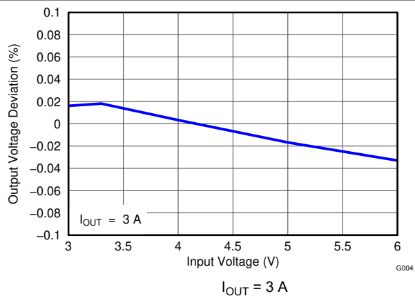
Figure 8-13. Output Voltage Regulation vs Input Voltage
