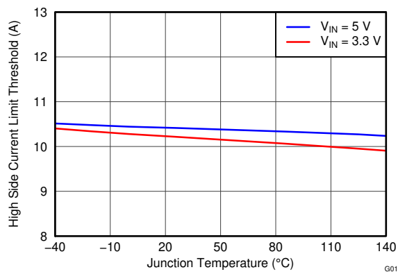
Figure 6-17. High-Side FET Current Limit vs Temperature
