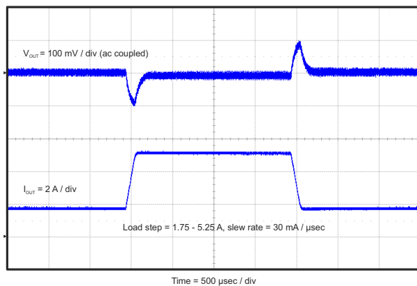
Figure 8-4. Transient Response, 3.5 A Step
