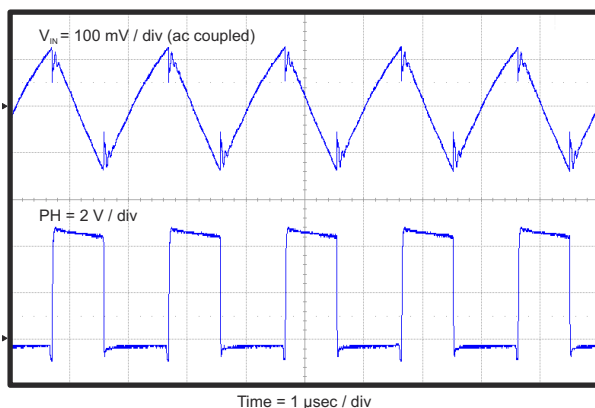
Figure 8-10. Input Ripple, I_{OUT} = 7\text{ A}
