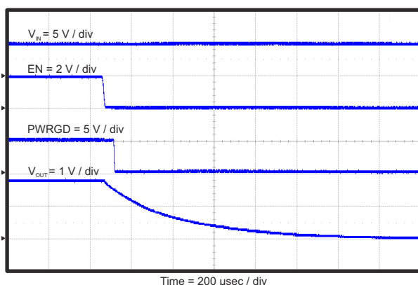
Figure 8-8. Power Down Relative To EN
