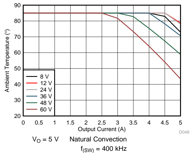
Figure 48. 5-V Outputs
