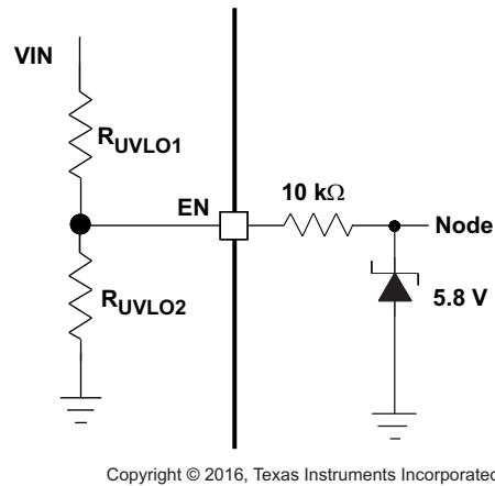
Figure 23. Low Input Voltages Applications
