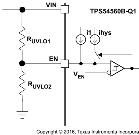
Figure 22. Adjustable Undervoltage Lockout (UVLO)
