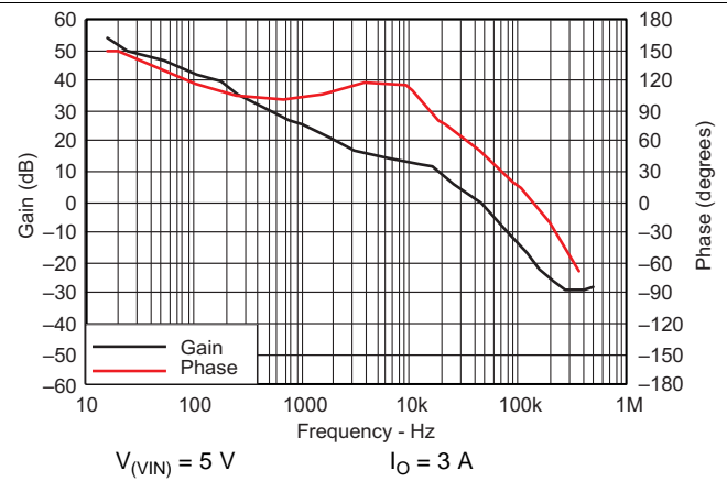
Figure 46. Closed-Loop Response
