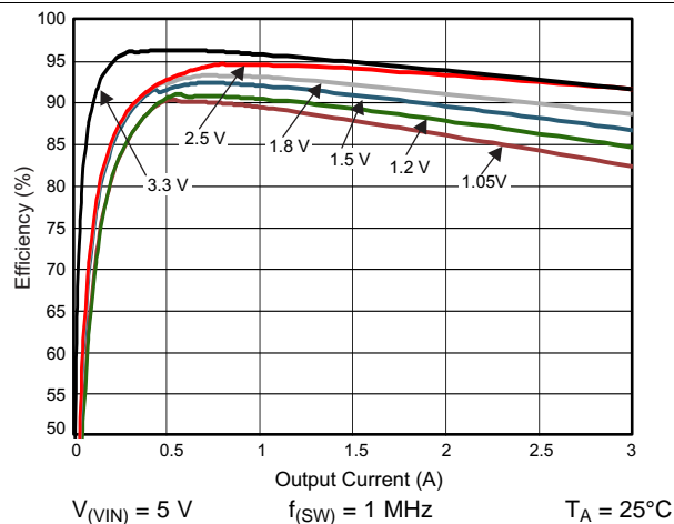
Figure 38. Efficiency vs Load Current
