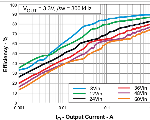
Figure 50. Light Load Efficiency
