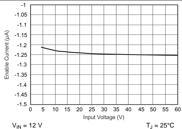
Figure 11. Enable-Pin Pullup Current vs Input Voltage
