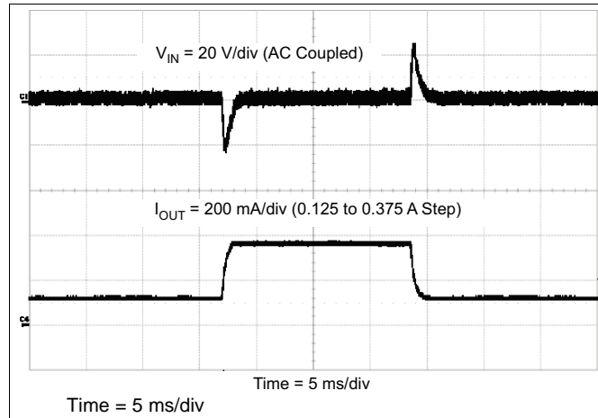
Figure 51. Load Transient
