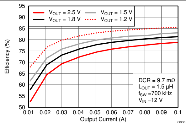
Figure 8-7. Light-Load Efficiency vs. Output Current
