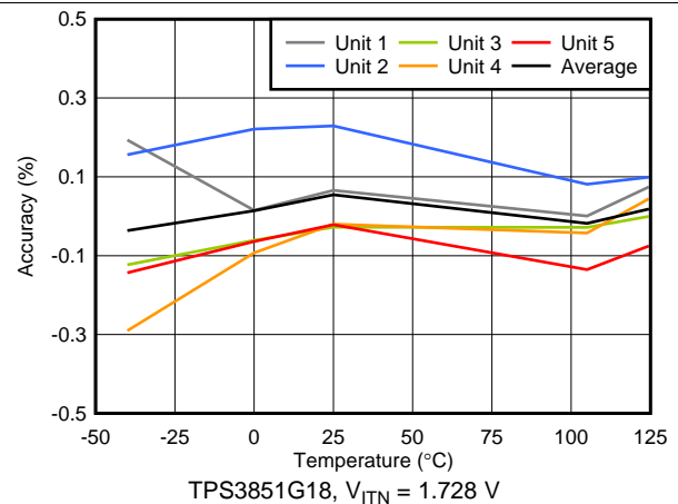
Figure 6. V_{ITN} + V_{HYS} Accuracy vs Temperature
