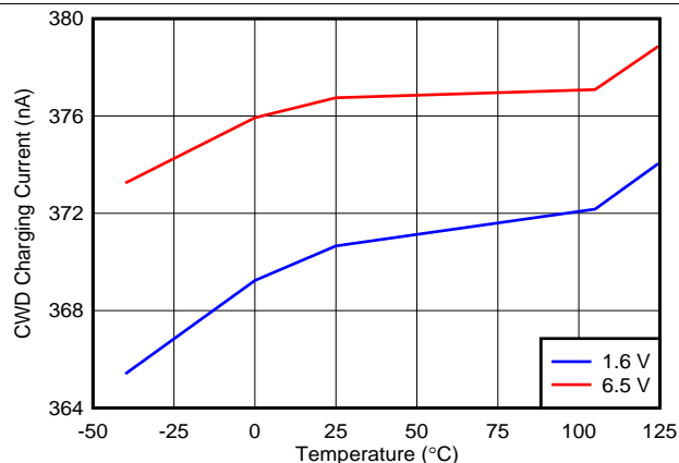
Figure 10. CWD Charging Current vs Temperature
