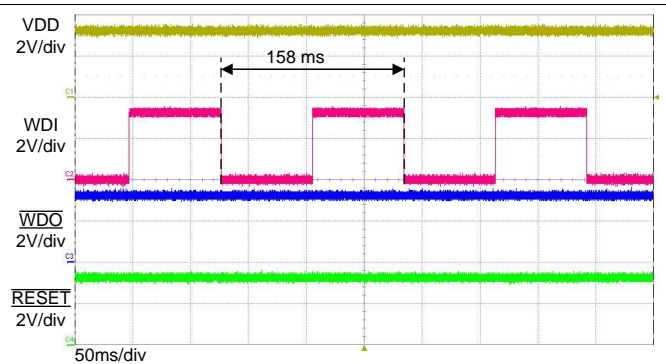
Figure 41. Typical WDI Signal
