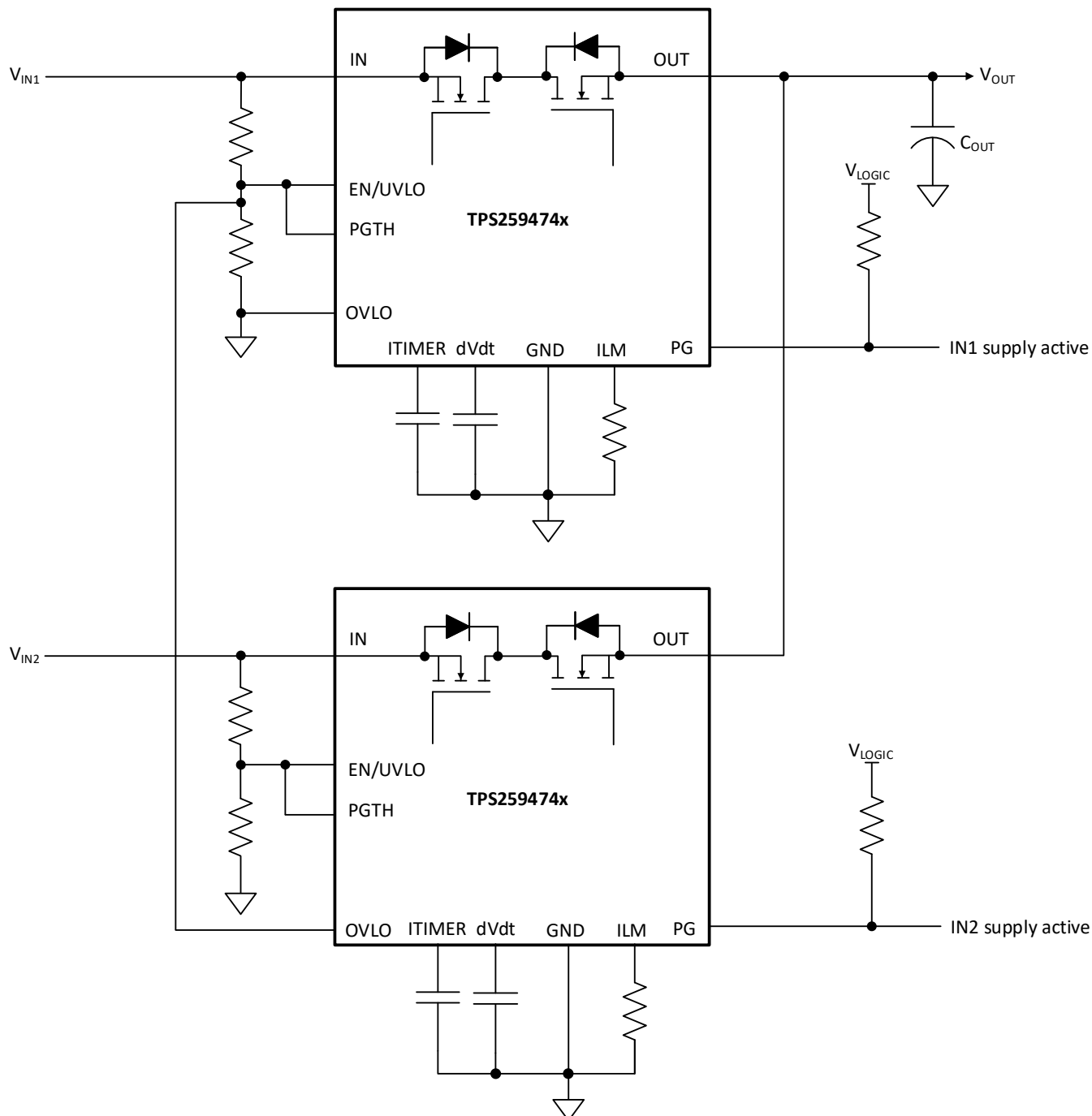
Figure 9-15. Priority power MUXing with 2 x TPS25947x
