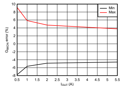
Figure 7-16. Analog Current Monitor Gain Accuracy
