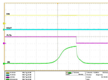
Figure 7-53. Output Short-Circuit During Steady State
