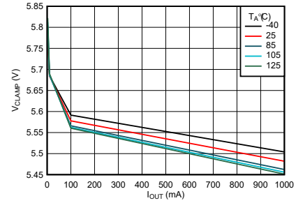
Figure 7-27. OVC Clamping Voltage (OVCSEL = Open) vs Load Current
