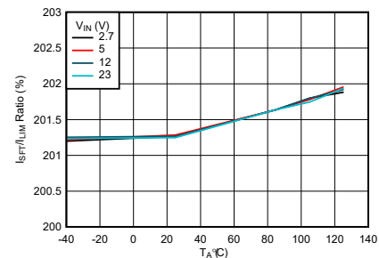
Figure 7-17. Scalable Fast-Trip Threshold:Current Limit Threshold ( I_{LIM} ) Ratio vs Temperature
