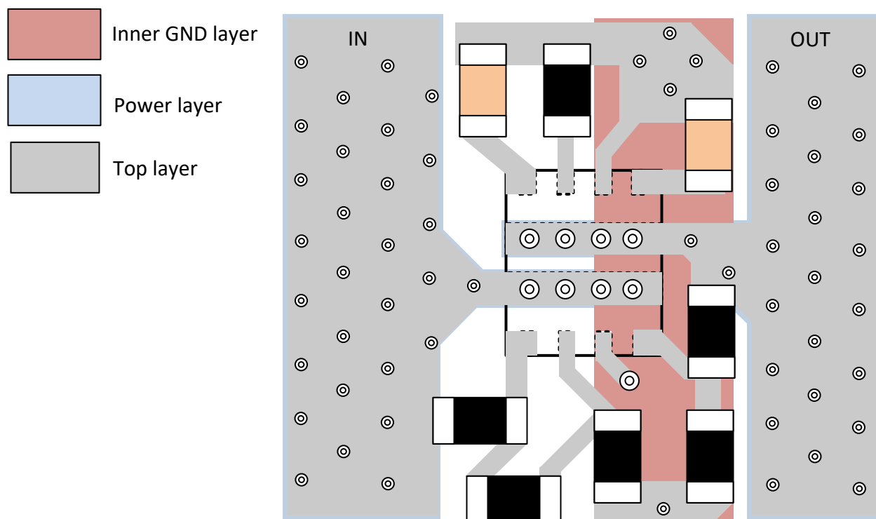
Figure 11-1. Layout Example - Single TPS25947x with PGTH Referred to OUT
