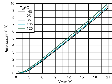
Figure 7-23. Reverse Leakage Current During OFF-State
