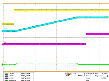
Figure 7-38. Start Up with Enable
