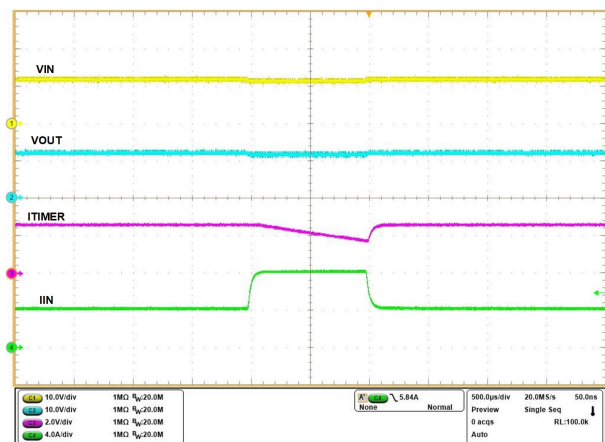
Figure 9-5. Transient Overload
