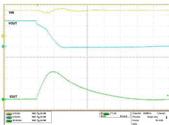
Figure 7-52. Circuit Breaker Response - TPS259474x
