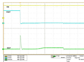
Figure 7-51. Transient Overcurrent Blanking Timer Response - TPS259474x
