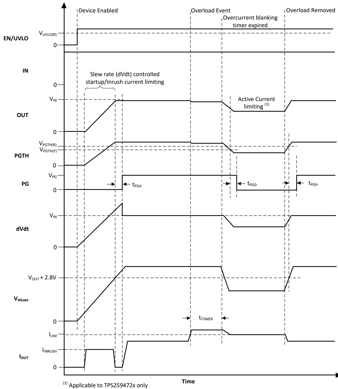
Figure 8-17. TPS259472x/74x PG Timing Diagram
