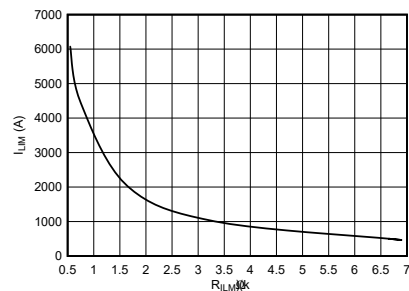
Figure 7-14. Overcurrent Threshold vs ILM resistor
