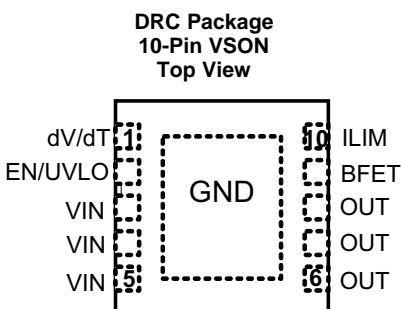
Pin Functions
