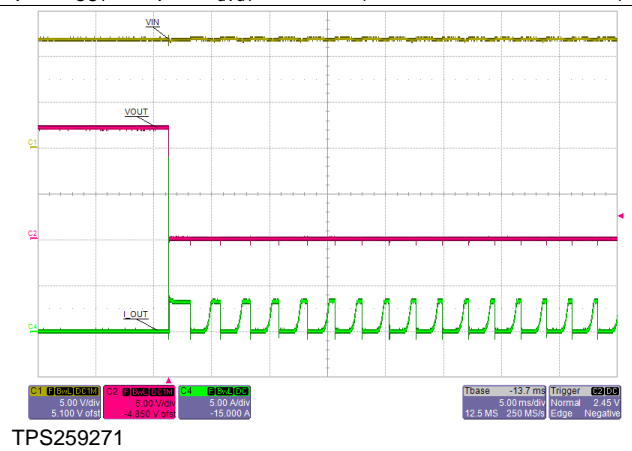
Figure 32. Transient: Thermal Fault Auto-Retry
