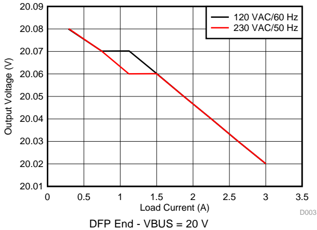
Figure 48. Load Regulation
