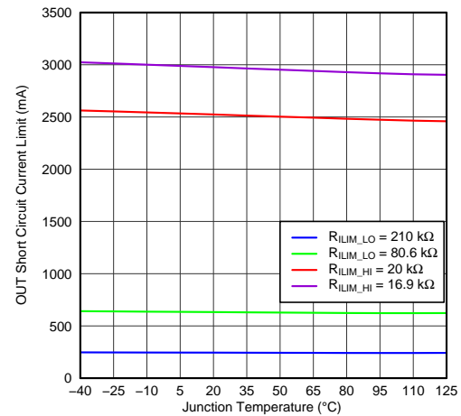
Figure 4. OUT Short-Circuit Current Limit vs Temperature
