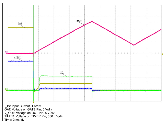
Figure 31. Current Limit During Output Load Short Circuit Condition (Overview)
