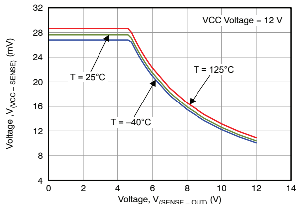
Figure 7. Voltage Across R_{SENSE} in Inrush Power Limiting vs V_{DS} of Pass MOSFET
