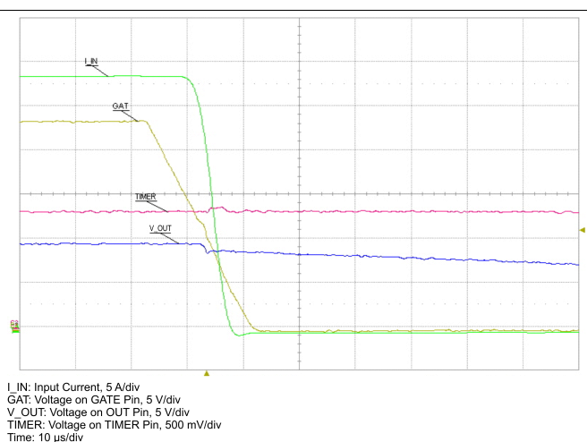
Figure 32. Current Limit During Output-Load Short-Circuit Condition (Onset)
