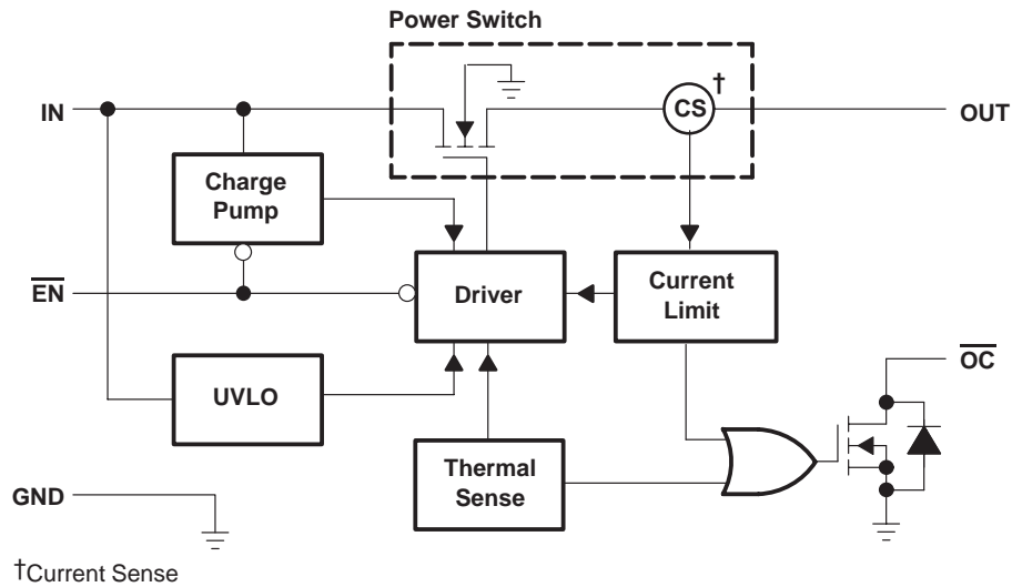
TPS2045 functional block diagram
