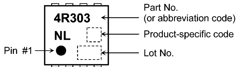
Fig. 7.1 Marking
