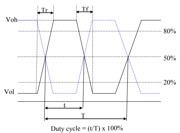
Test waveform
