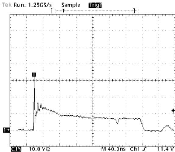
Figure 5. Positive 8kV contact per IEC 61000-4-2
