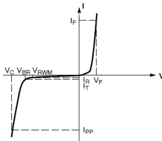
Uni-Directional TVS
