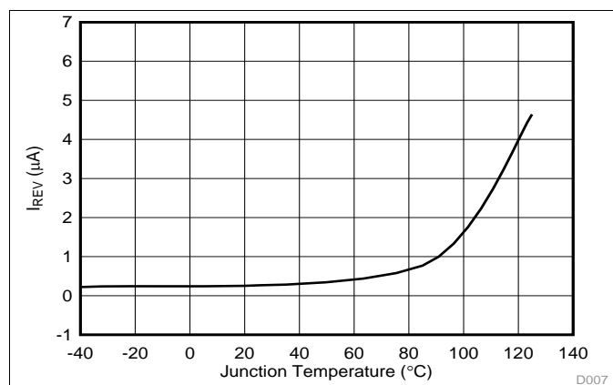
Figure 5. Reverse Leakage Current ( I_{REV} ) vs Temperature
