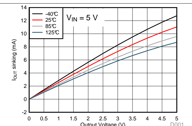
Figure 6. Output Discharge Current vs Output Voltage
