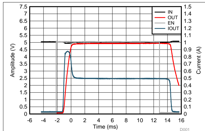
Figure 1. Turn ON into 10 \Omega
