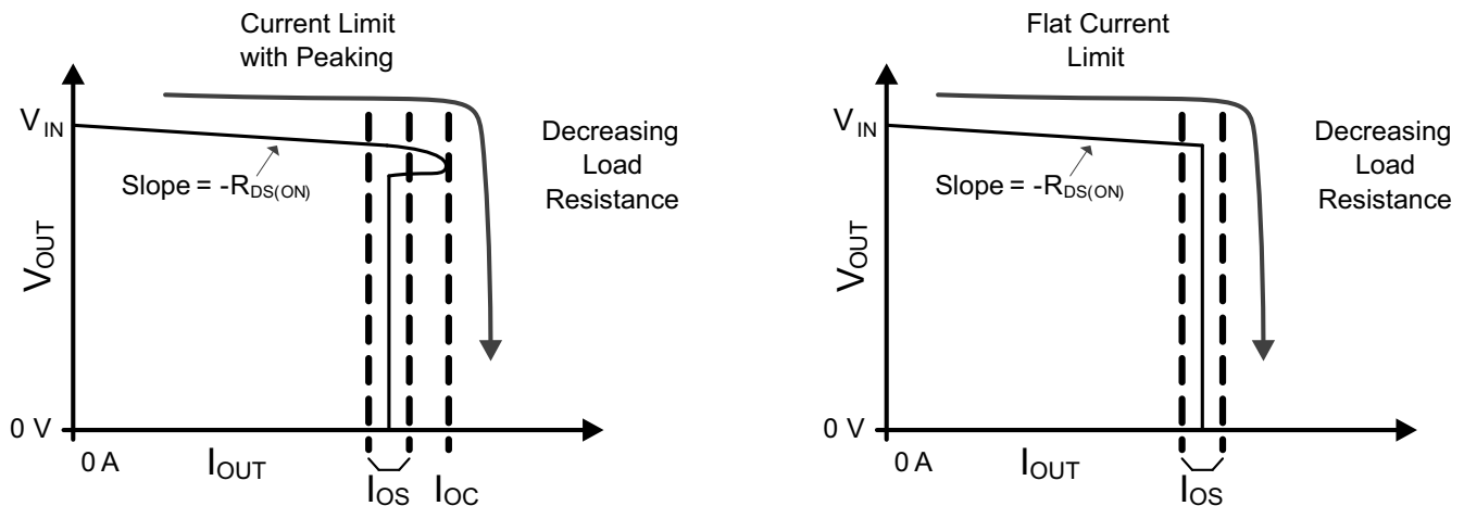
Figure 25. Current Limit Profiles
