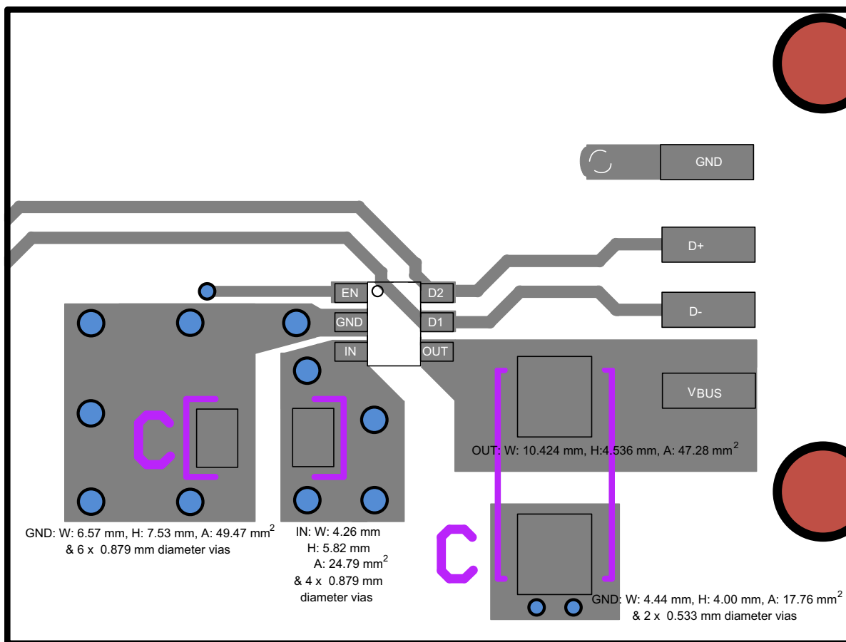
Figure 32. PCB Layout Example
