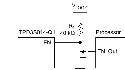
Figure 27. Implementing Active Low Logic for EN Pin
