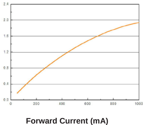
Luminous Flux vs. Forward Current
