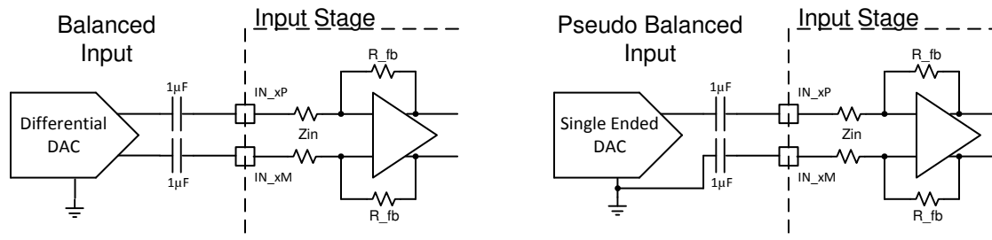
Figure 7-1. Differential Analog Input Connections
