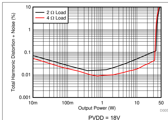
Figure 9-3. THD vs Output Power
