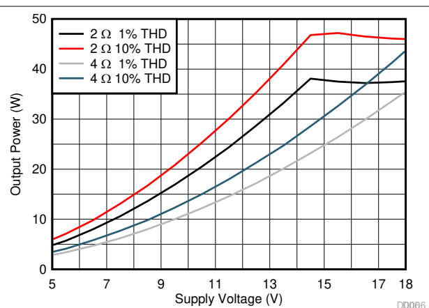
Figure 9-4. Output Power vs Supply Voltage
