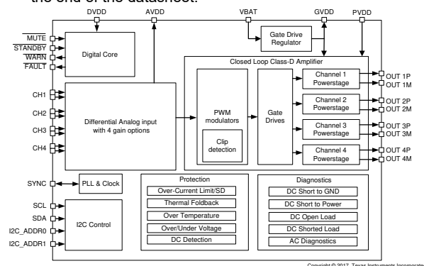
Block Diagram
