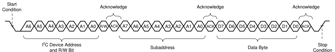
Figure 7-9. Random Write Transfer
