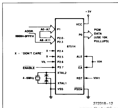
Figure 6. Program Verification
