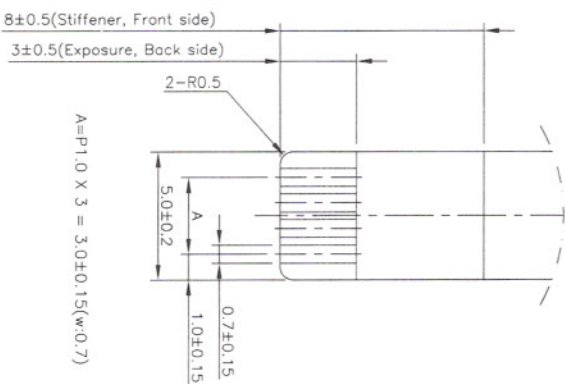
Detail AA (Scale=5/1)
