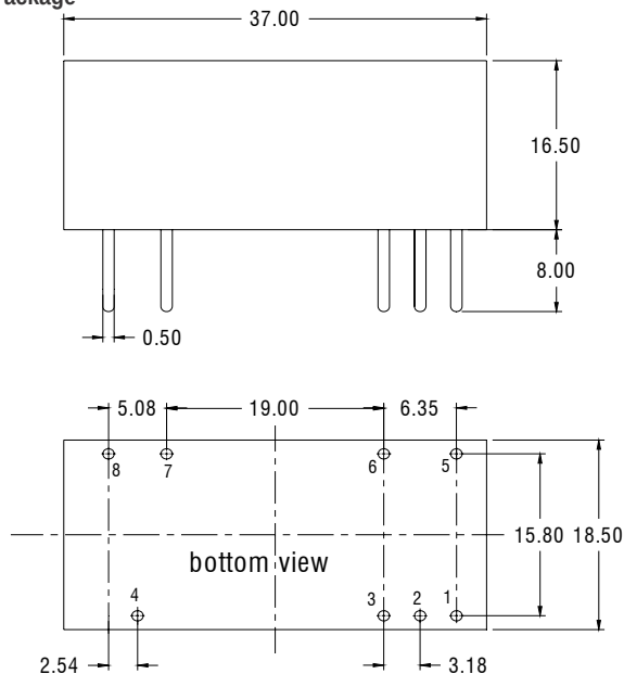
DIP Package
