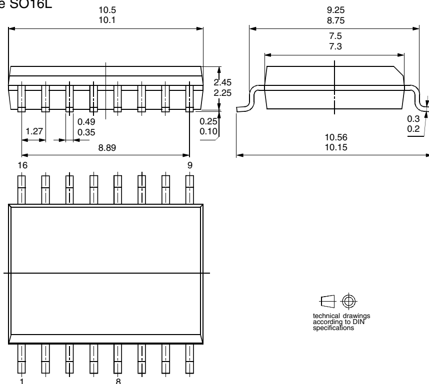
Package SO16L
