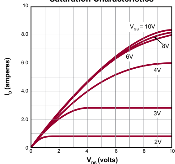
Saturation Characteristics
