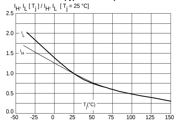
Figure 6: Relative variation of holding and latching current versus junction temperature (typical values)
