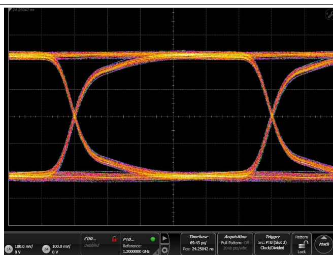
T_A = 25^\circ\text{C} Bias = 1.5 V 50 \Omega Termination Figure 24. Eye Pattern: 2.4 Gbps Through Path
