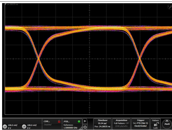
T_A = 25^\circ\text{C} Bias = 1.5 V 50 \Omega Termination Figure 26. Eye Pattern: 3 Gbps Through Path
