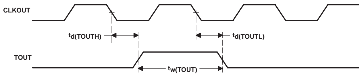
Figure 4–19. TOUT Timing
