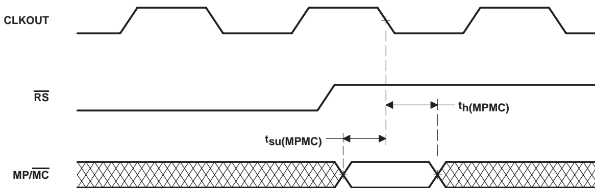
Figure 4-16. \overline{\text{MP/MC}} Timing
