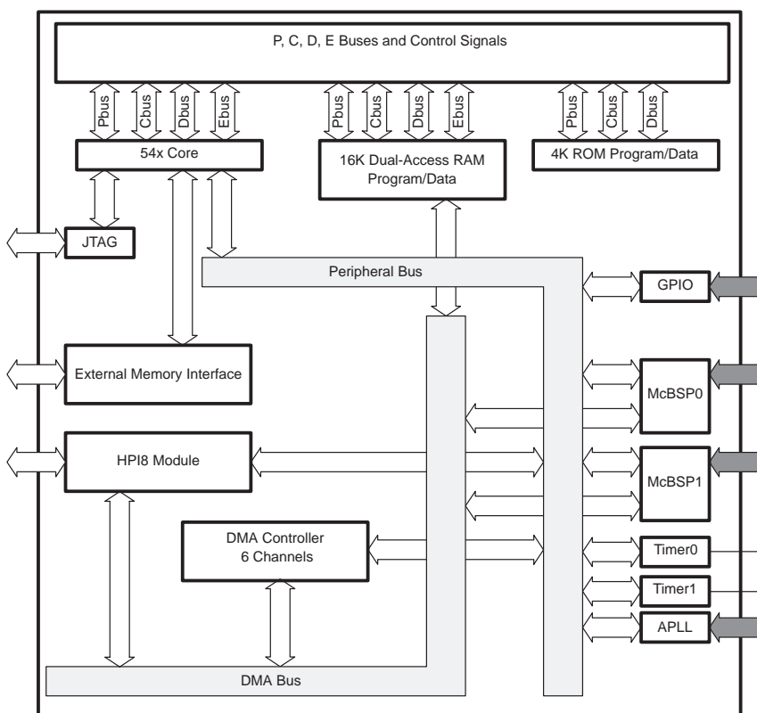
Figure 2–1. Block Diagram of the TMS320UC5402
