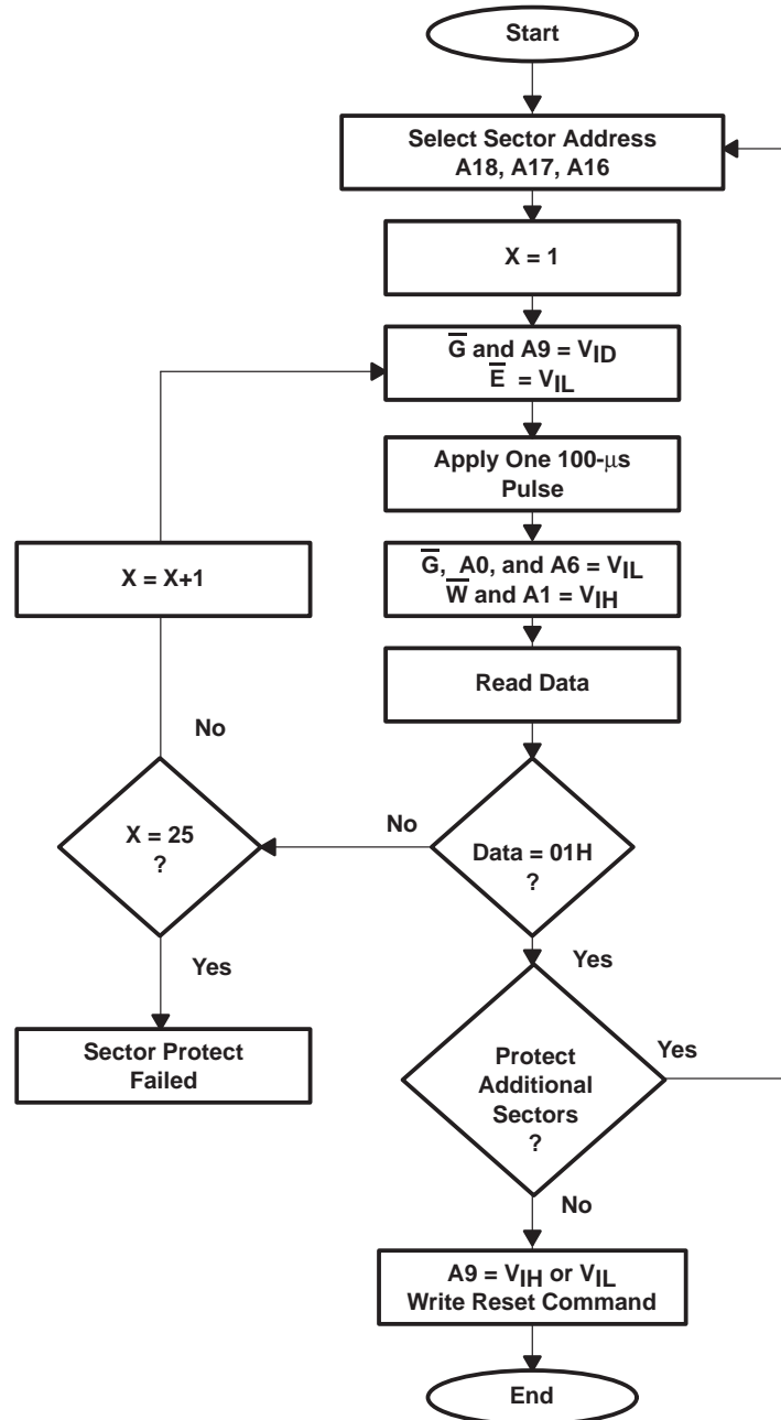
Figure 14. Sector-Protect Algorithm
