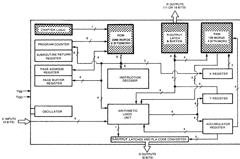
FIGURE 7 – TMS 1100/1300 LOGIC BLOCKS
