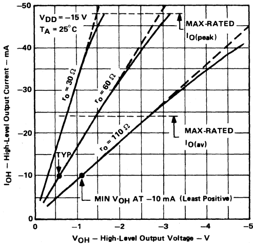
HIGH-LEVEL OUTPUT CURRENT vs HIGH-LEVEL OUTPUT VOLTAGE
