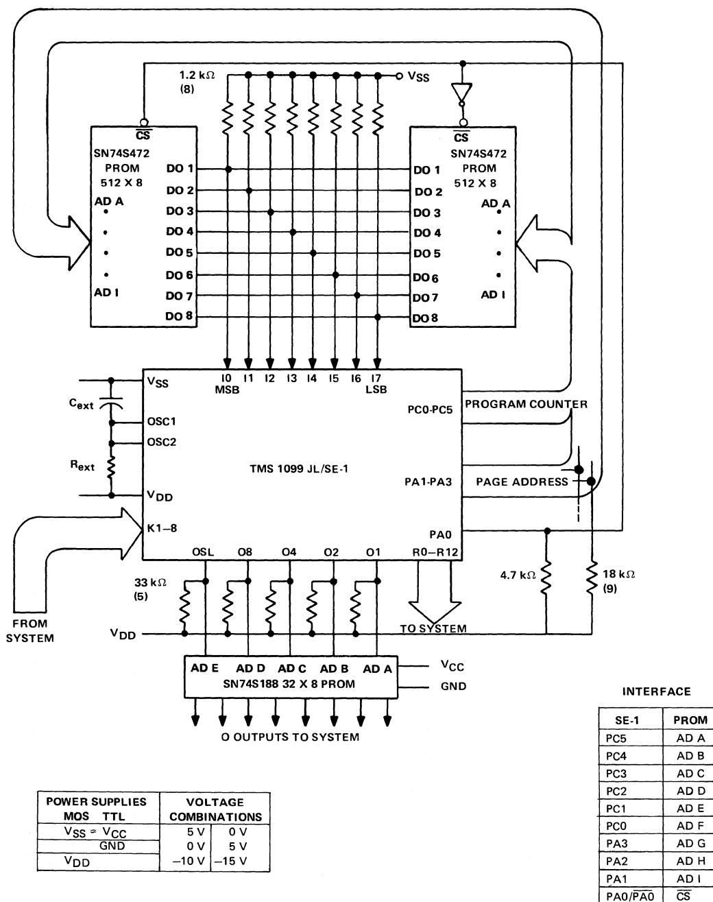
FIGURE 10- BLOCK DIAGRAM OF TYPICAL APPLICATION – PROTOTYPING SYSTEM WITH SE-1
