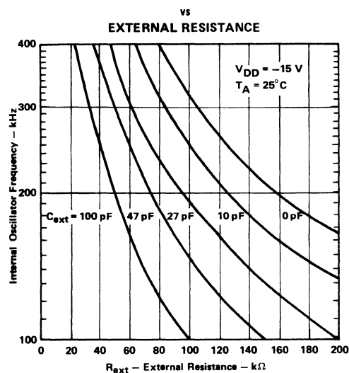
TYPICAL INTERNAL OSCILLATOR FREQUENCY
