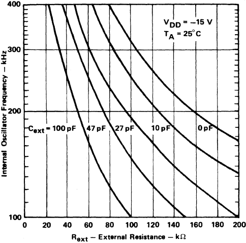
TYPICAL INTERNAL OSCILLATOR FREQUENCY vs EXTERNAL RESISTANCE
