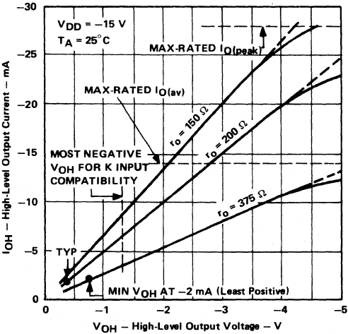
HIGH-LEVEL OUTPUT CURRENT vs HIGH-LEVEL OUTPUT VOLTAGE
