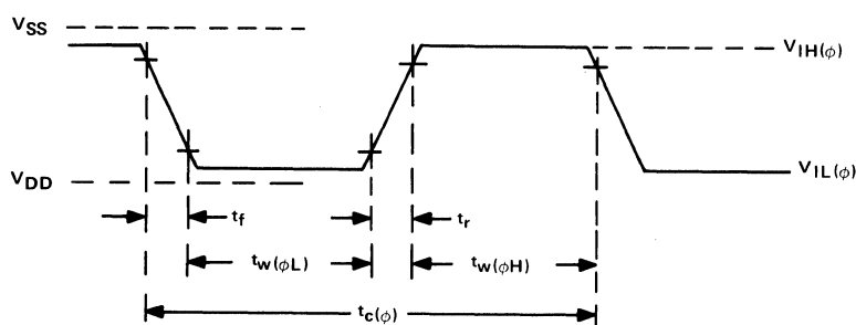
FIGURE 11 – EXTERNALLY DRIVEN CLOCK INPUT WAVEFORM
