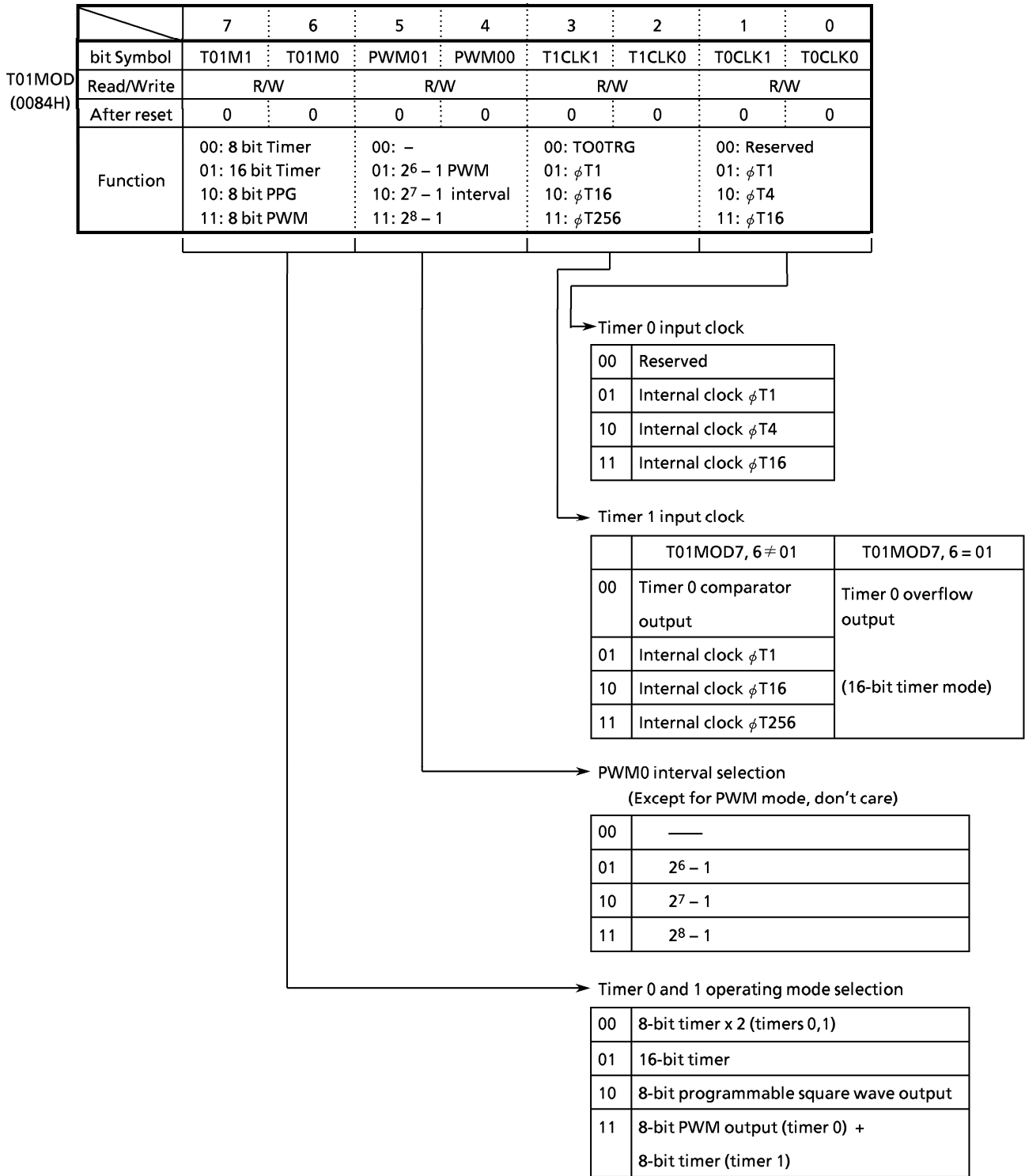
Figure 3.8 (4) Timer 0/1 Mode Register (T01MOD)
