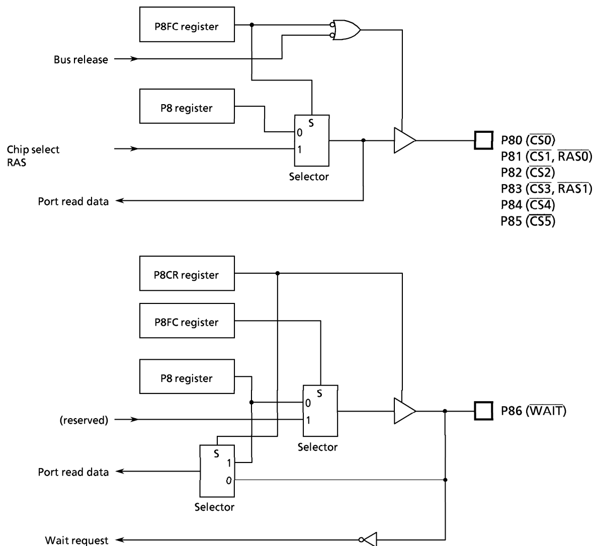
Figure 3.5 (7) Port 8
