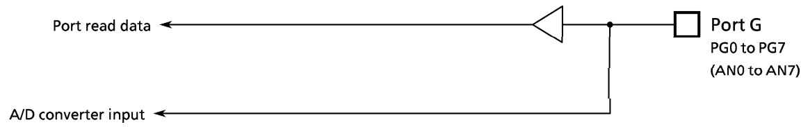
Figure 3.5 (14) Port G
