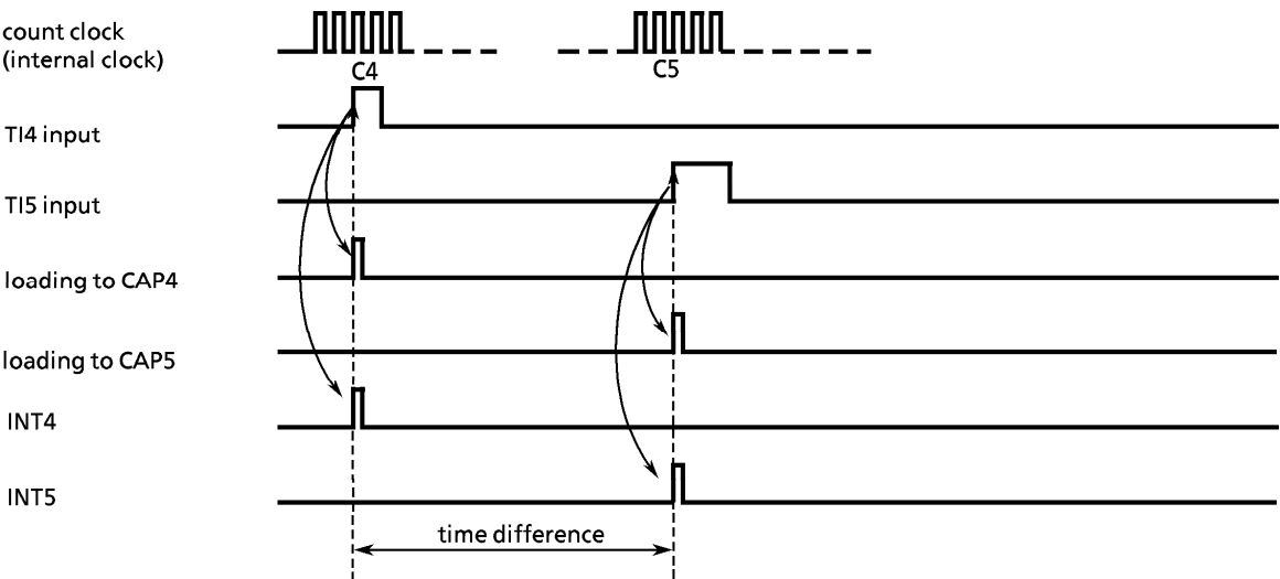
Figure 3.9 (26) Time Differential Measurement
