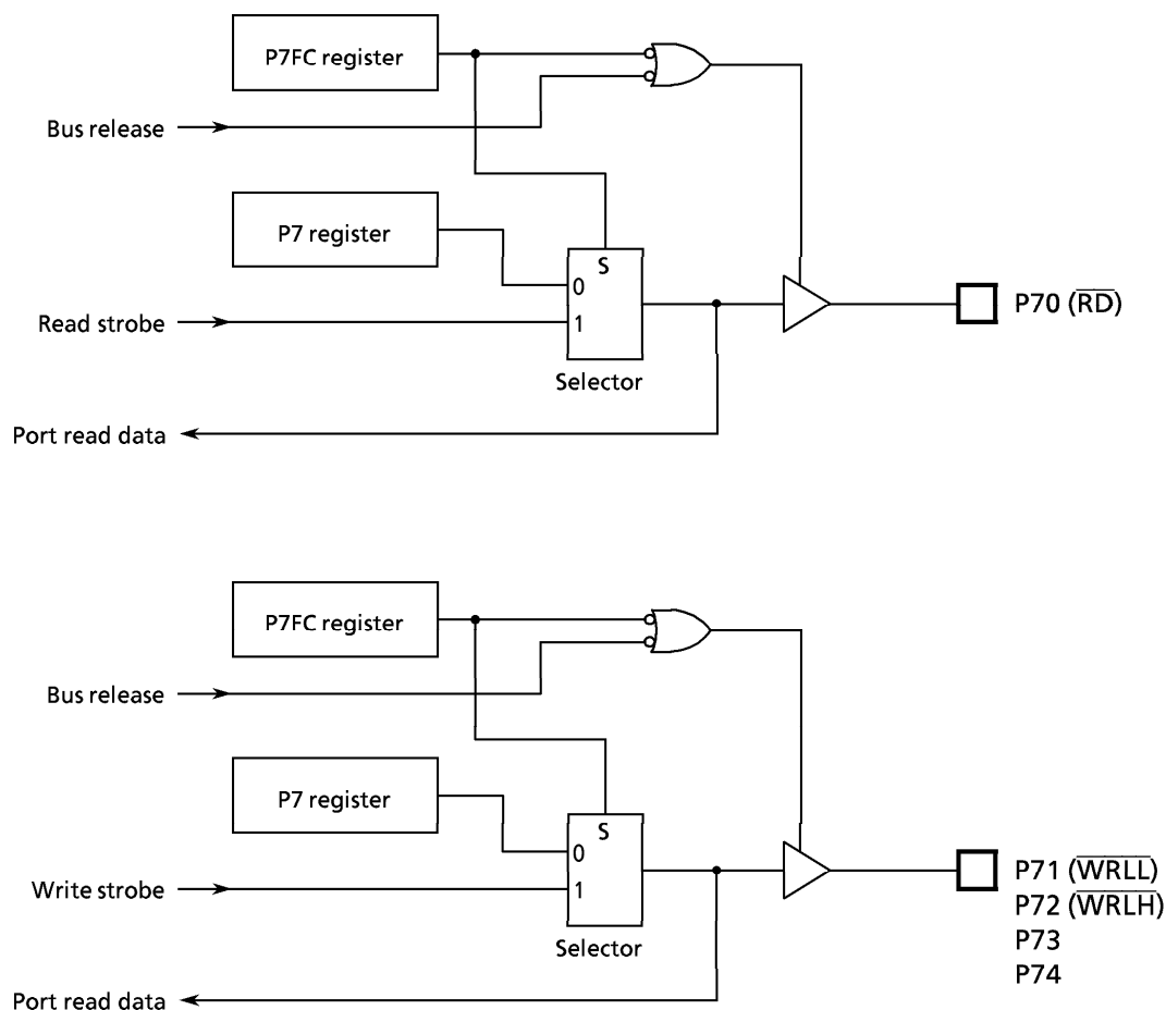
Figure 3.5 (6-1) Port 7 (P70 to P74)
