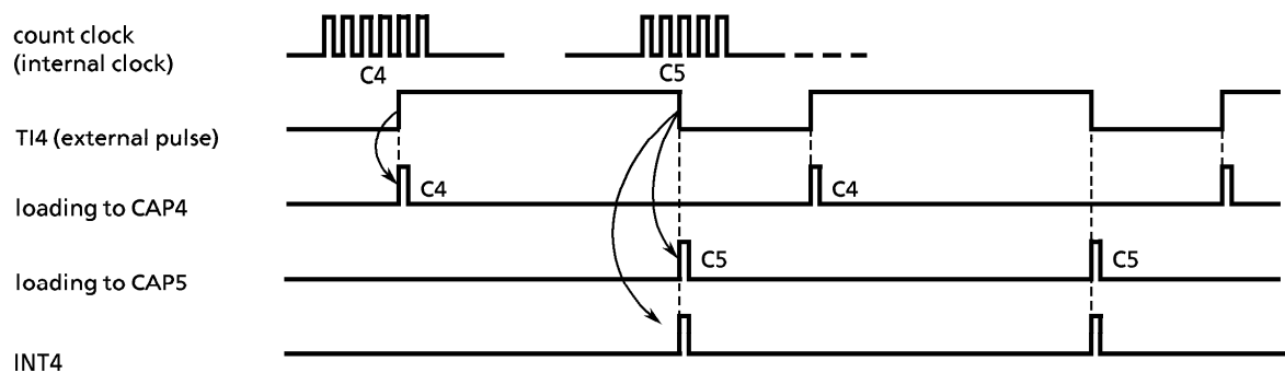
Figure 3.9 (25) Pulse Width Measurement
