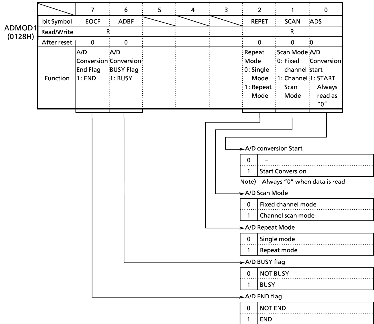
Figure 3.11 (2-1) A/D Control Register
