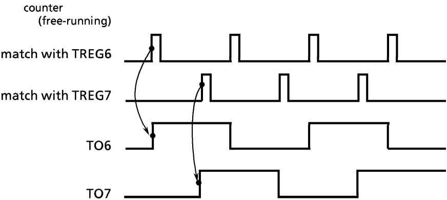
Figure 3.9 (27) Phase Output
