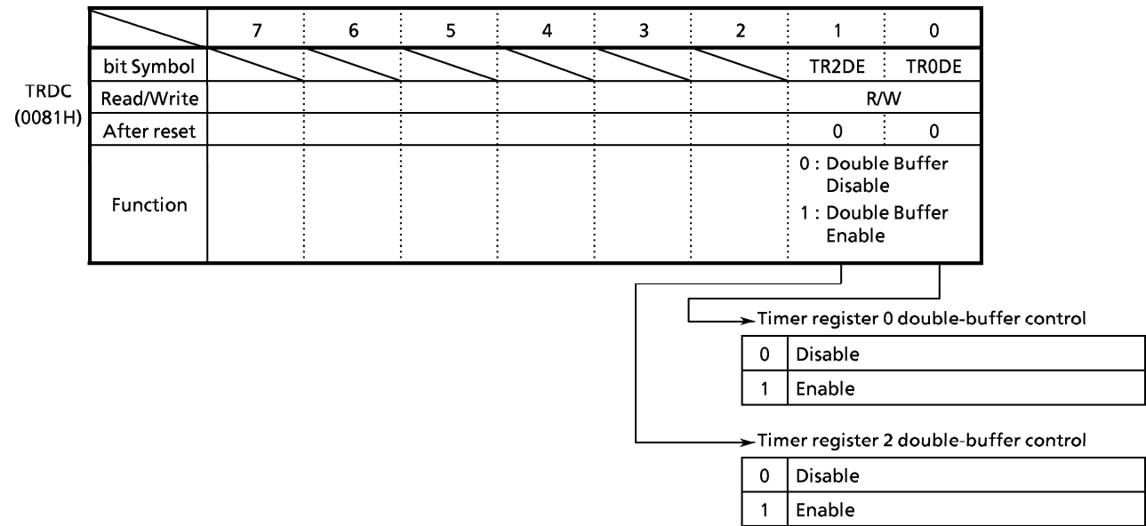
Figure 3.8 (8) Timer Register Double-Buffer Control Register (TRDC)
