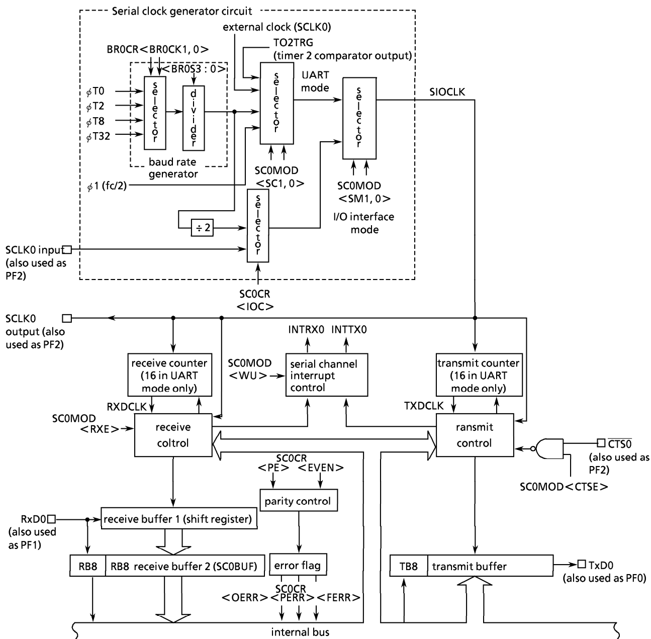
Figure 3.10 (11) Serial Channel 0 Block Diagram
