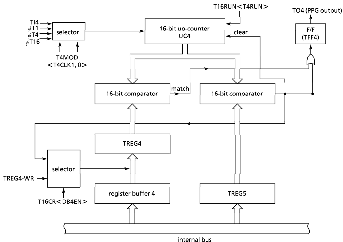
Figure 3.9 (21) 16-Bit PPG Mode Block Diagram
