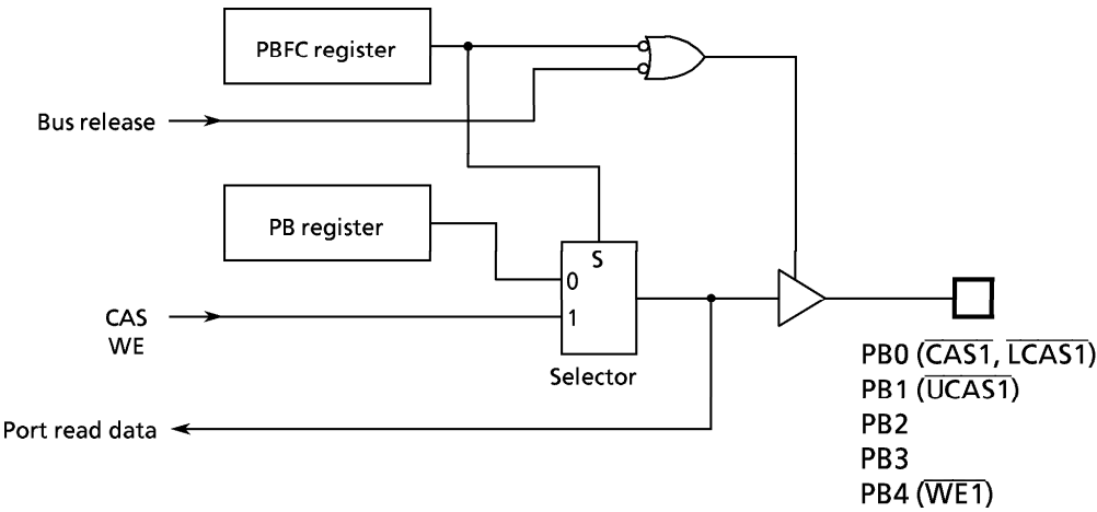
Figure 3.5 (9) Port B
