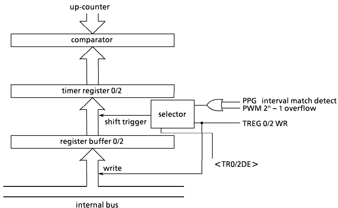
Figure 3.8 (3) Timer Register 0/2/4/6 Configuration
