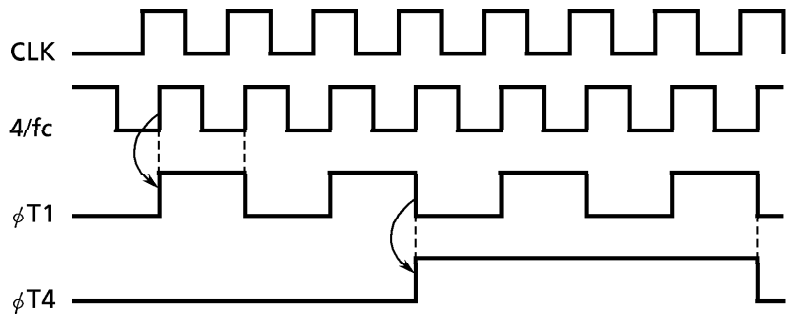
Figure 3.8 (2) Prescaler
