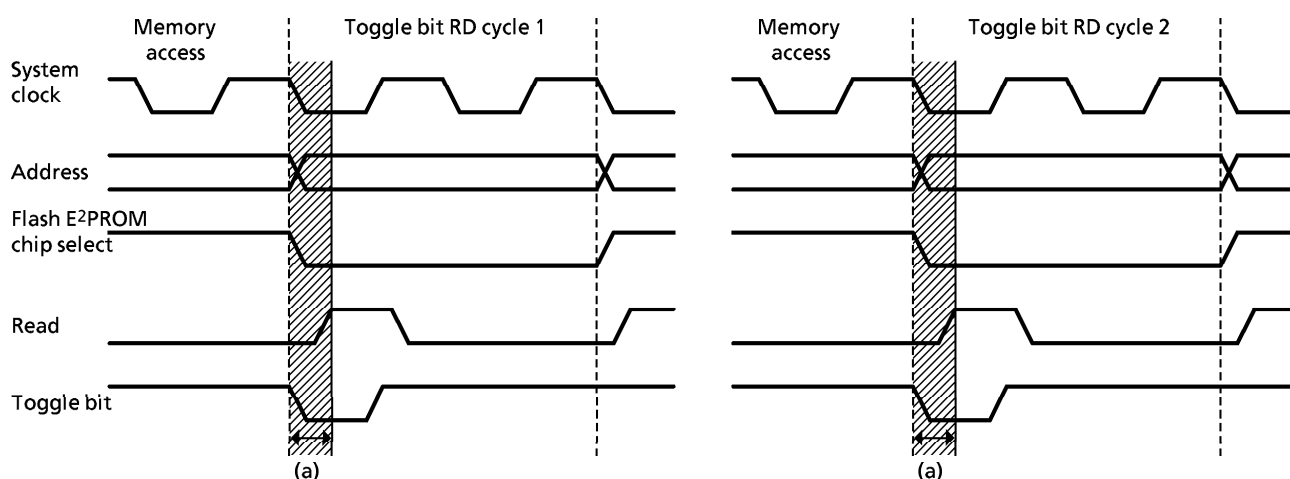
Figure 3.6 Flash E 2 PROM Toggle Bit Read Cycle
