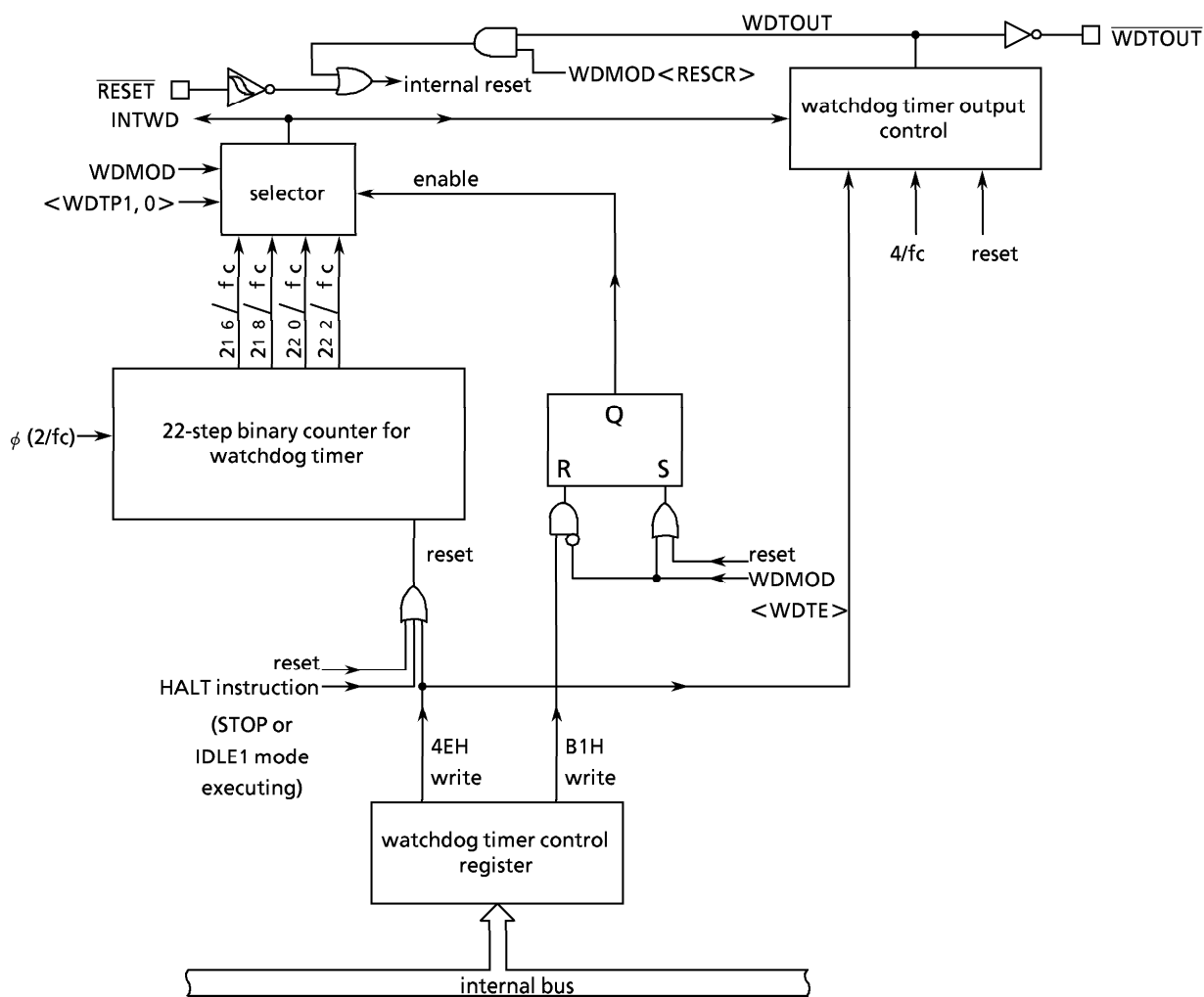
Figure 3.13 (1) Watchdog Timer Block Diagram
