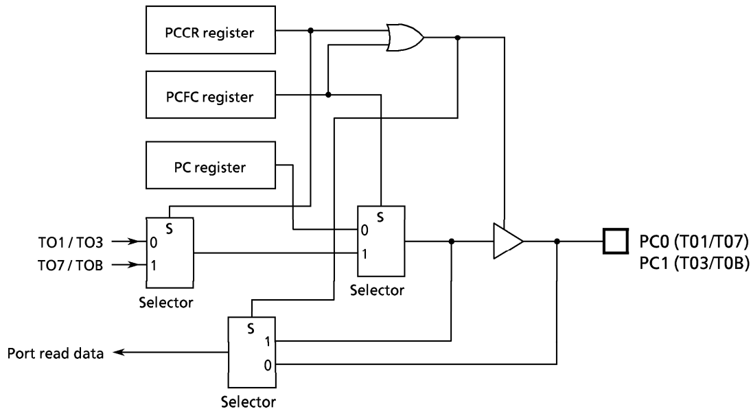
Figure 3.5 (10) Port C
