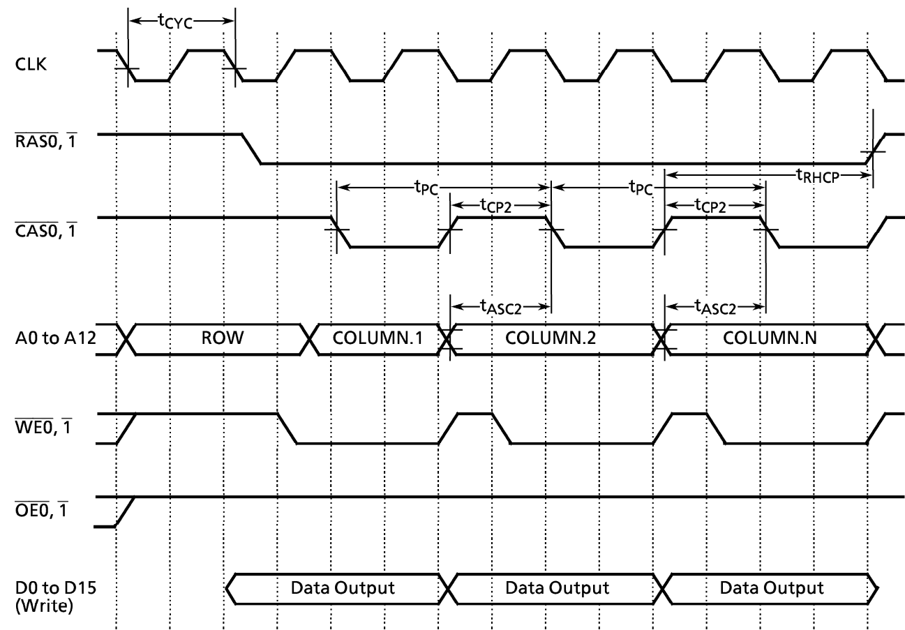
(6) DRAM Page mode write cycle (3-2-2-2 mode)
