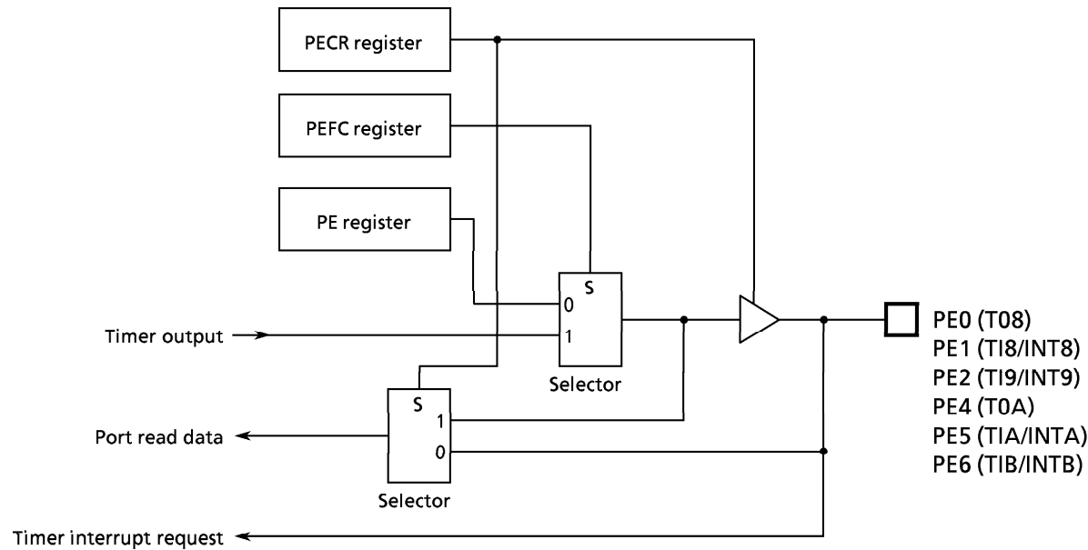
Figure 3.5 (12) Port E
