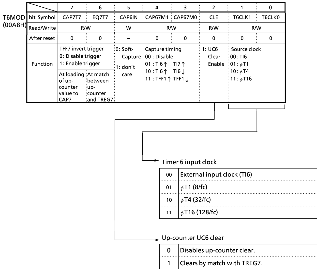
Figure 3.9 (8) 16-Bit Timer Mode Control Register (T6MOD) (1/2)
