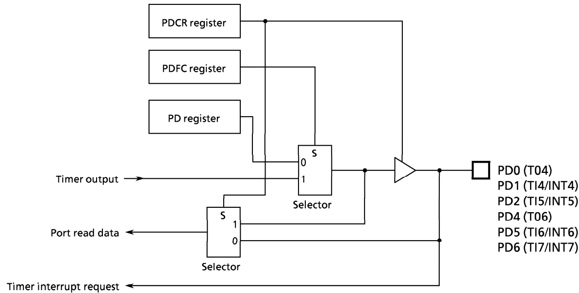
Figure 3.5 (11) Port D
