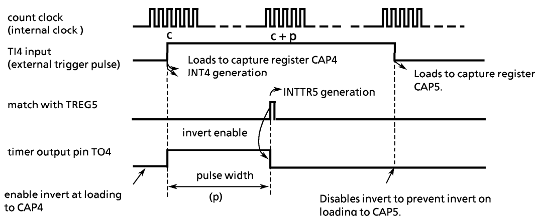
Figure 3.9 (23) One-Shot Pulse Output (No Delay)
