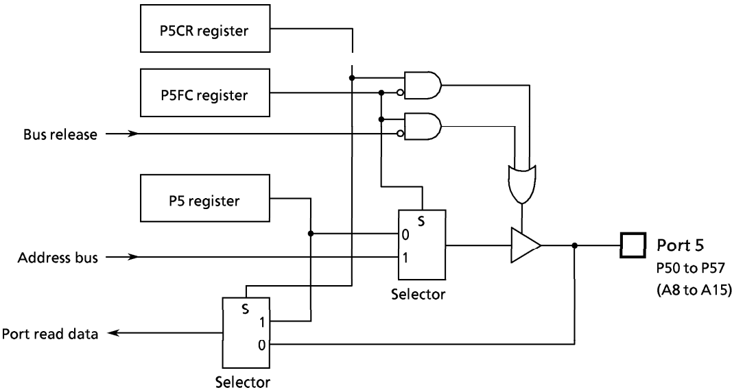
5Figure 3.5 (4) Port 5
