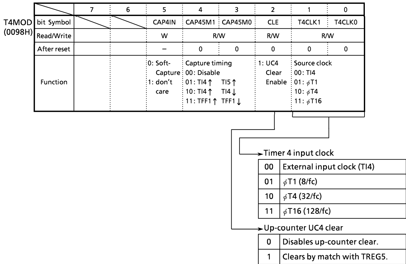
Figure 3.9 (5) 16-Bit Timer Mode Control Register (T4MOD) (1/2)
