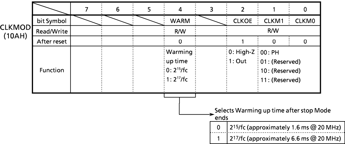
Figure 3.13 (6) CLOCK Mode Register
