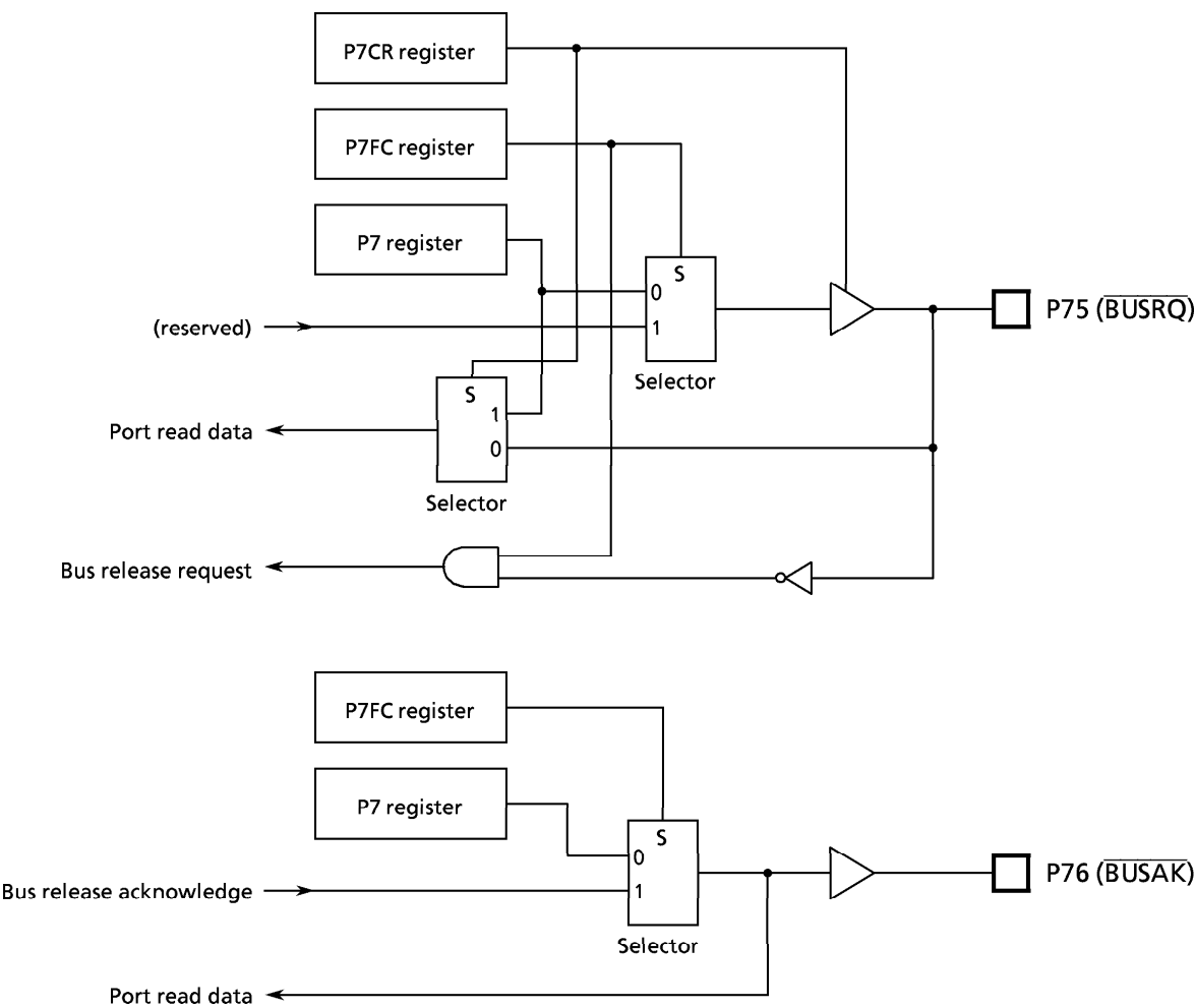
Figure 3.5 (6-2) Port 7 (P75, P76)
