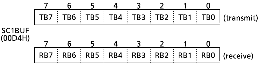
Figure 3.10 (9) Serial Transmit/Receive Buffer Register (SC1BUF, Channel 1)
