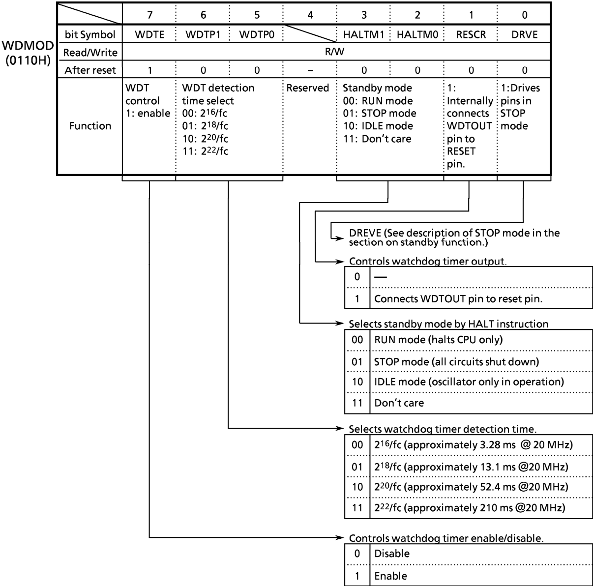
Figure 3.13 (4) Watchdog Timer Mode Register
