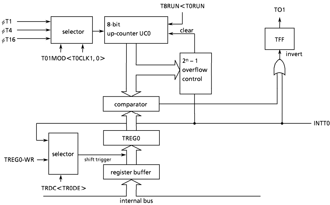
Figure 3.8 (14) 8-Bit PWM Output Mode Block Diagram
