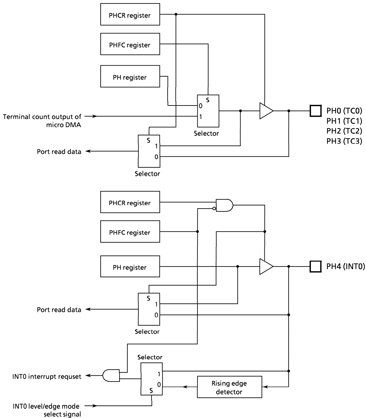
Figure 3.5 (15) Port H
