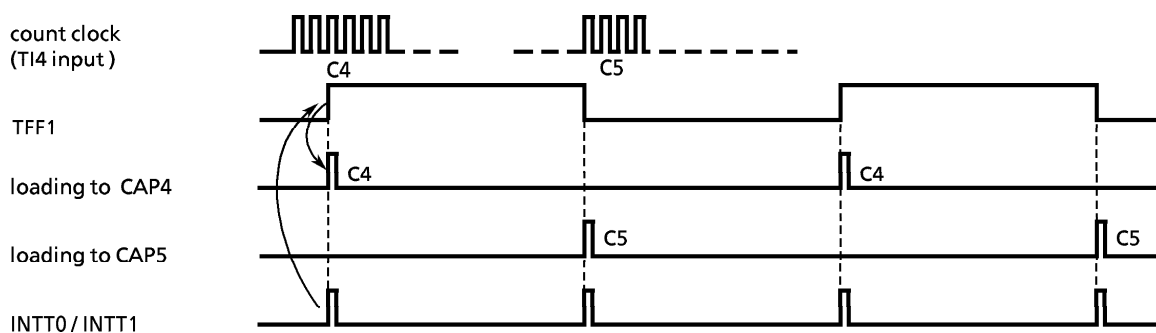
Figure 3.9 (24) Frequency Measurement
