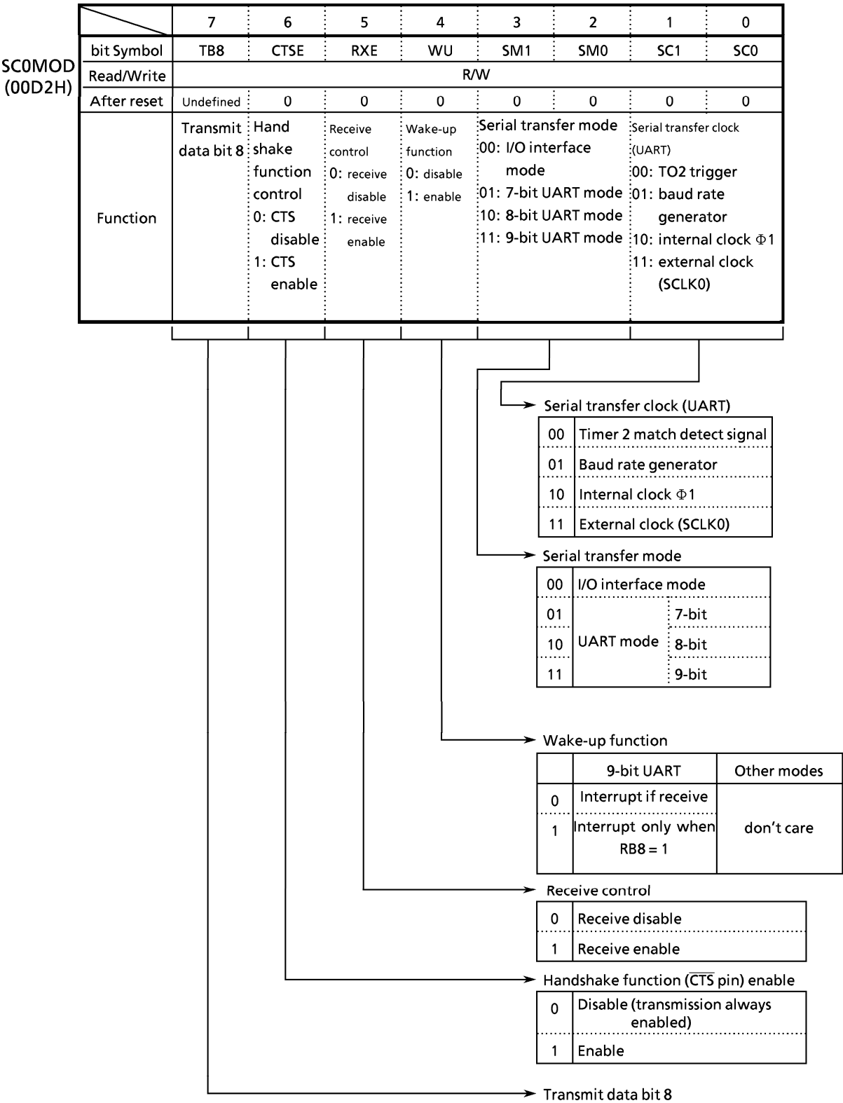
Figure 3.10 (2) Serial Mode Control Register (SC0MOD, Channel 0)
