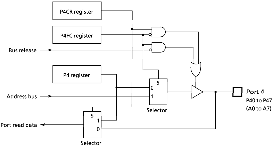
Figure 3.5 (3) Port 4
