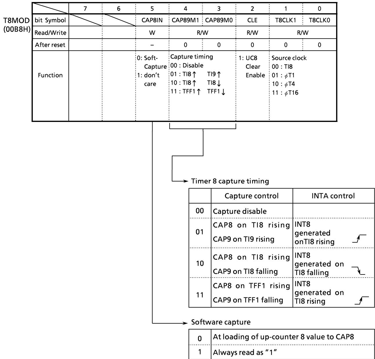
Figure 3.9 (12) 16-Bit Timer Control Register (T8MOD) (2/2)
