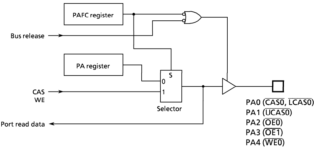
Figure 3.5 (8) Port A
