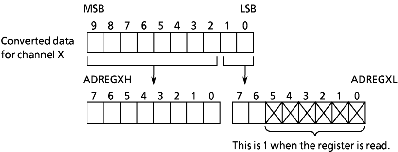
Figure 3.11 (3-2) A/D Conversion Result Register (ADREG26, 37)
