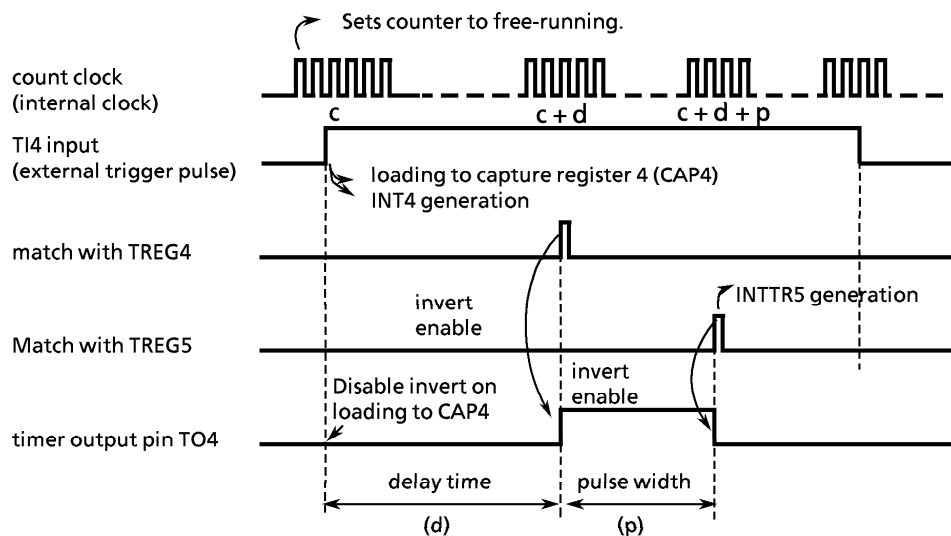
Figure 3.9 (22) One-Shot Pulse Output (With Delay)
