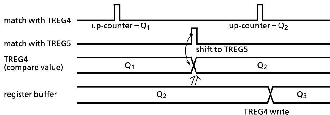
Figure 3.9 (20) Register Buffer Operation
