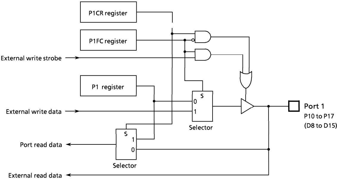
Figure 3.5 (2) Port 1
