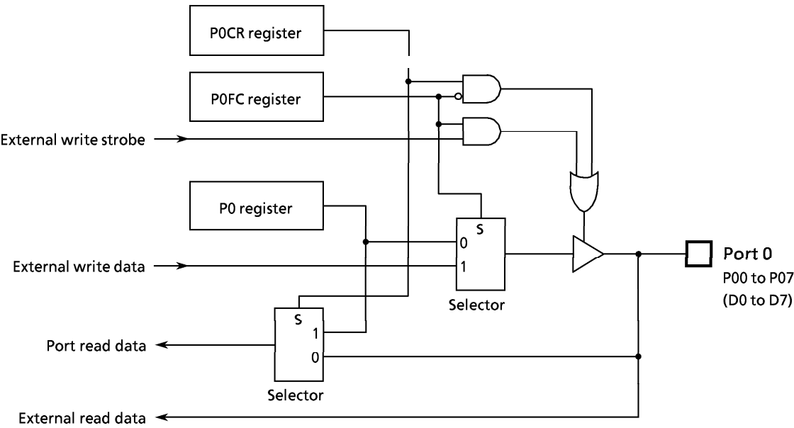
Figure 3.5 (1) Port 0
