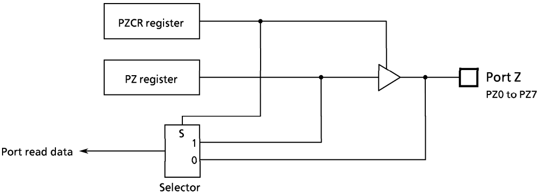
Figure 3.5 (16) Port Z
