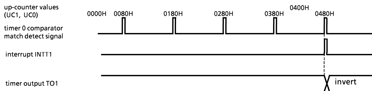
Figure 3.8 (12) Timer Output for 16-Bit Timer Mode
