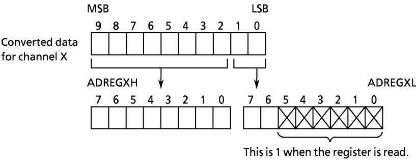
Figure 3.11 (3-1) A/D Conversion Result Register (ADREG04, 15)
