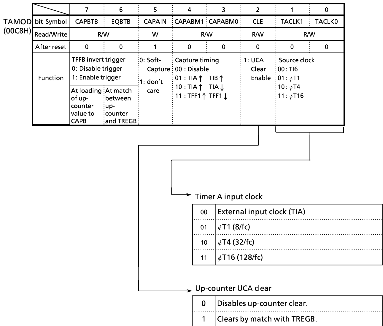
Figure 3.9 (14) 16-Bit Timer Mode Control Register (TAMOD) (1/2)
