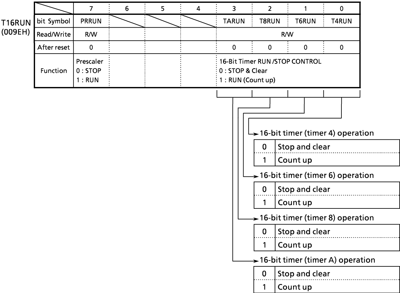
Figure 3.9 (17) 16-Bit Timer Operation Control Register (T16RUN)
