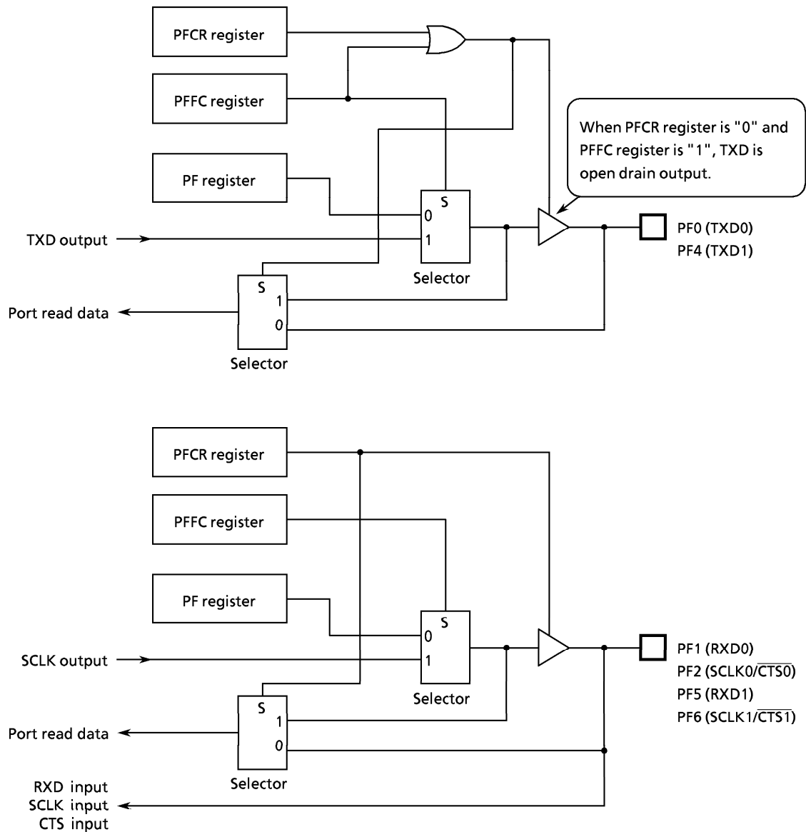
Figure 3.5 (13) Port F
