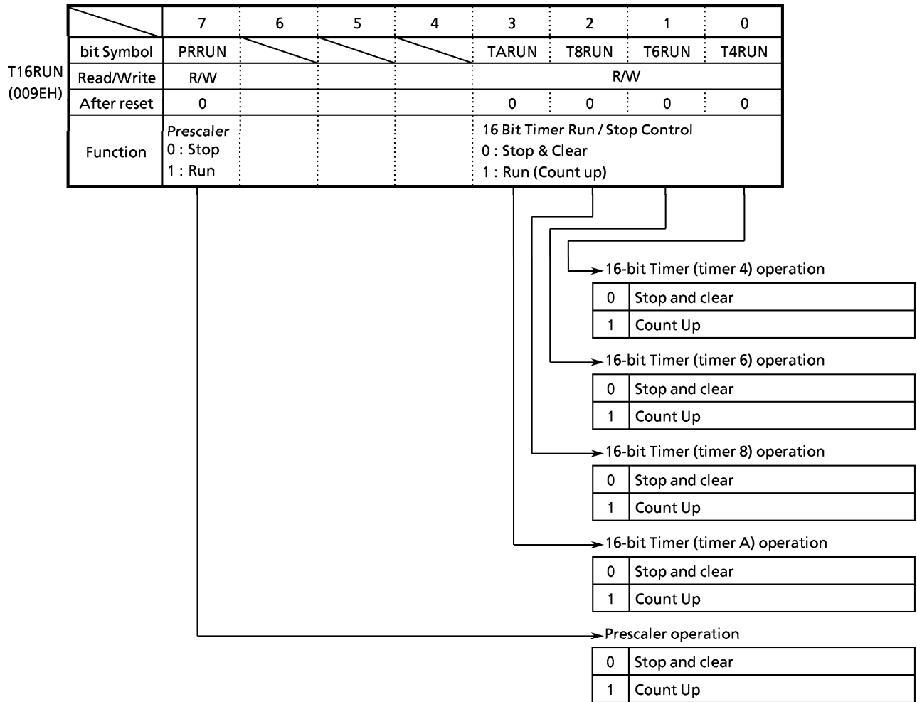
Figure 3.8 (9) 16-Bit Timer Operation Control Register (T16RUN)
