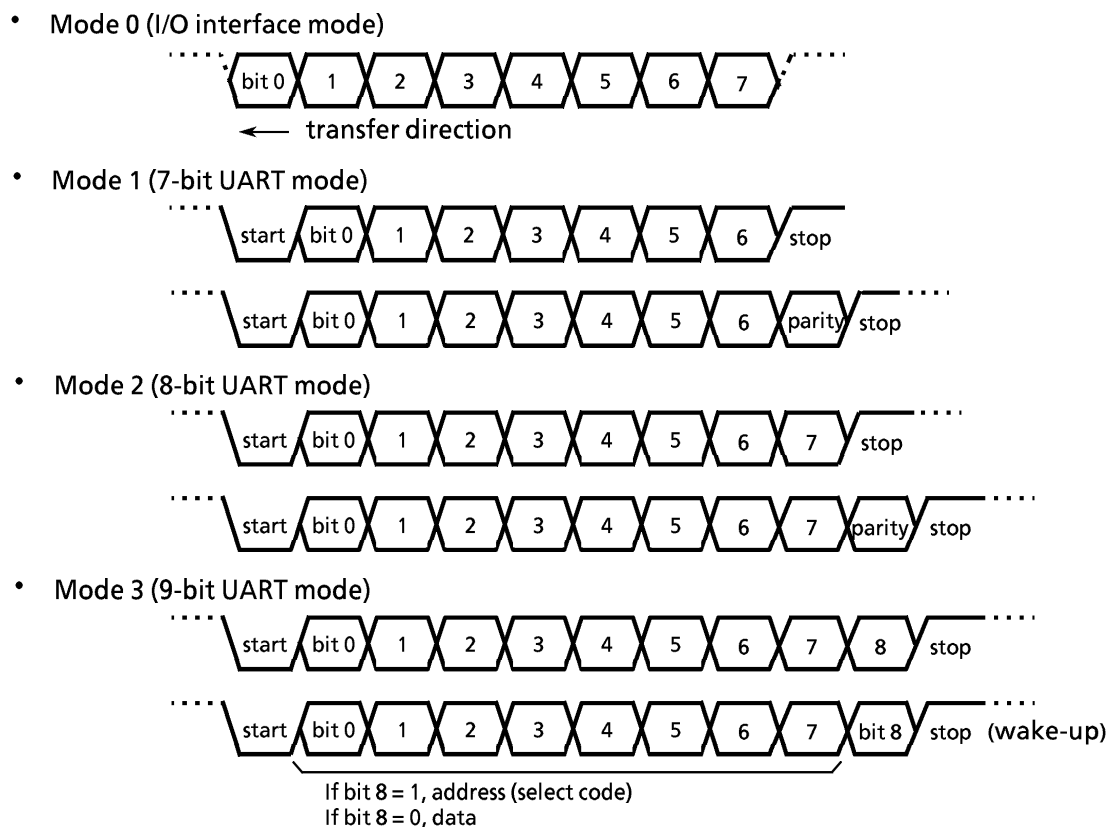
Figure 3.10 (1) Data Formats
