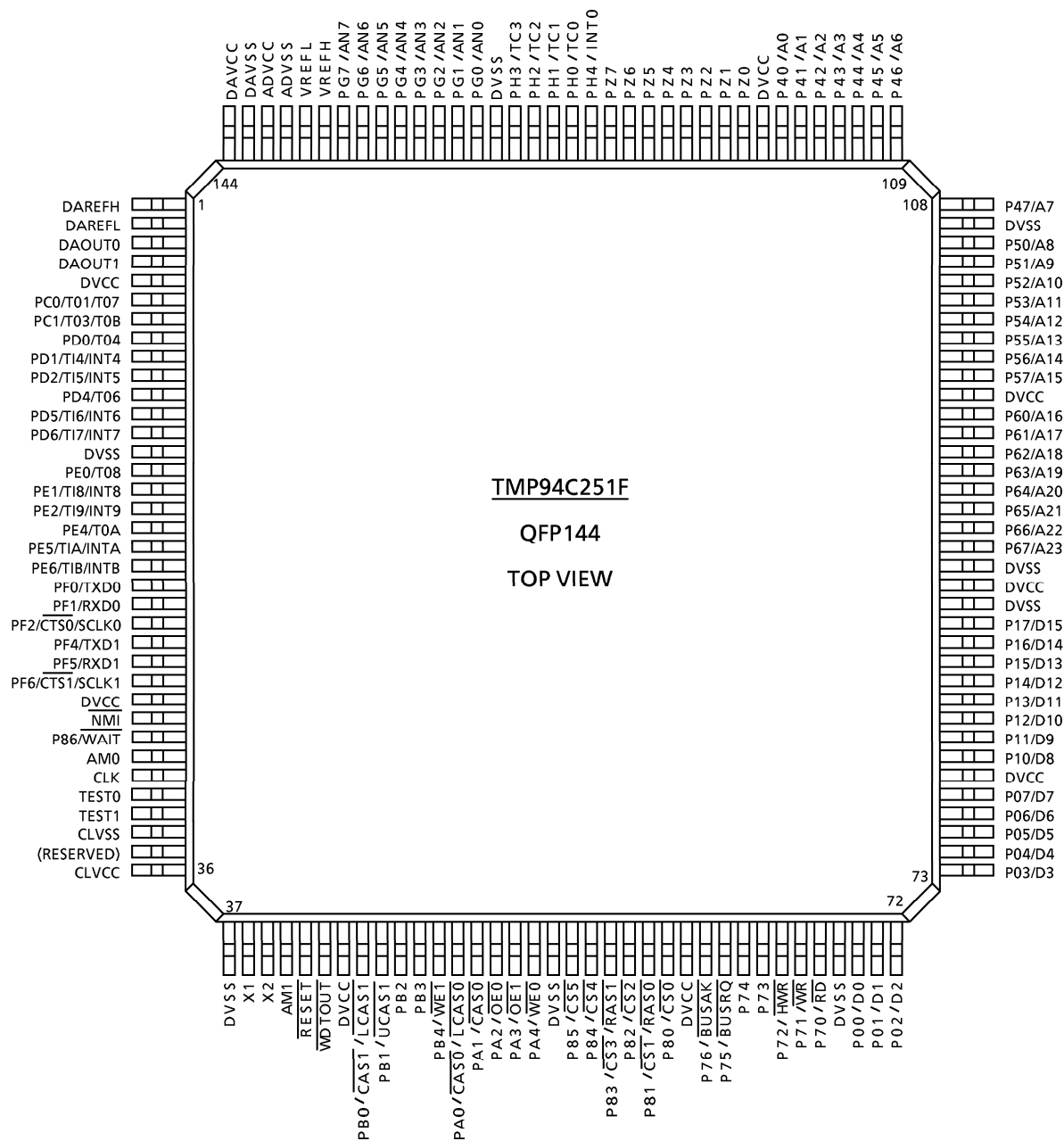
Figure 2.1 Pin Assignment
