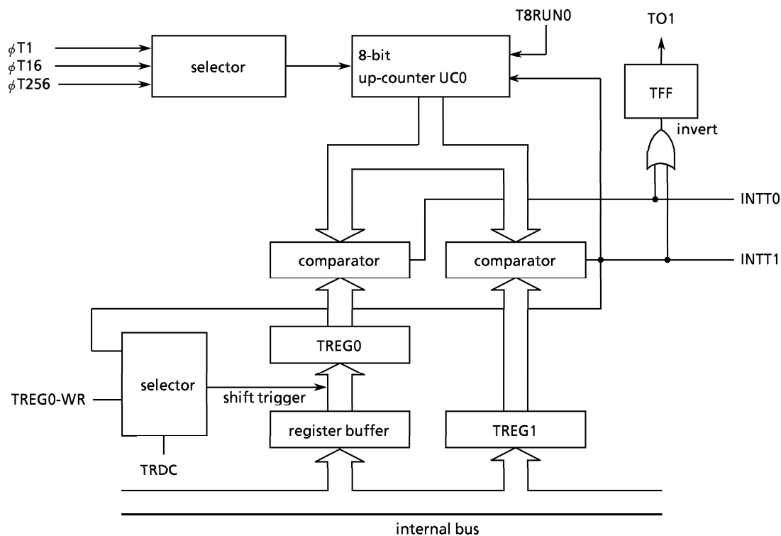
Figure 3.8 (13) 8-Bit PPG Output Mode Block Diagram
