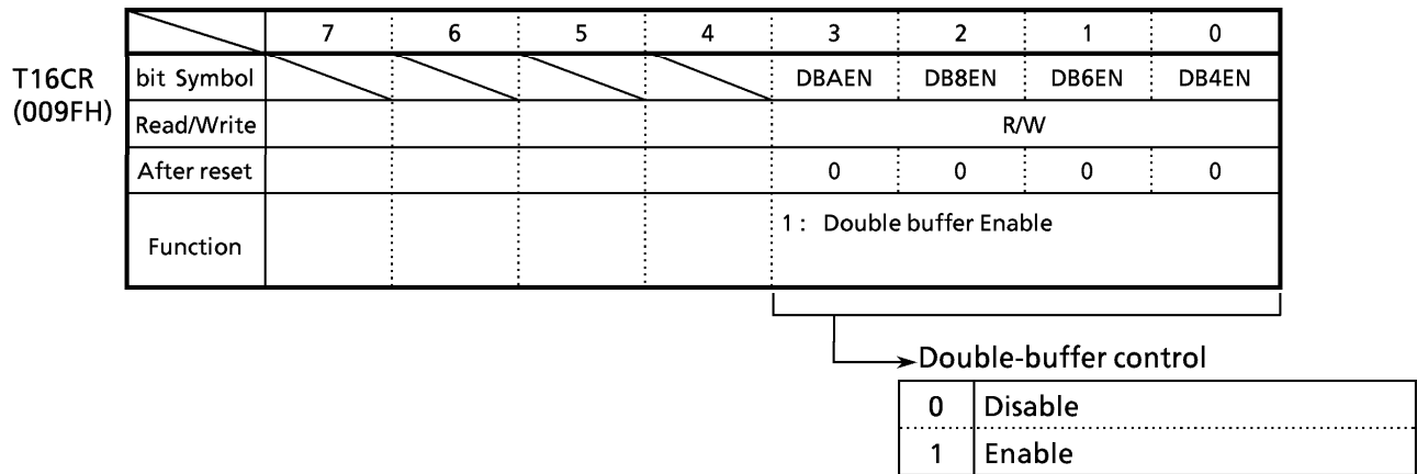
Figure 3.9 (18) 16-Bit Timer (4, 6, 8, A) Control Register (T16CR)
