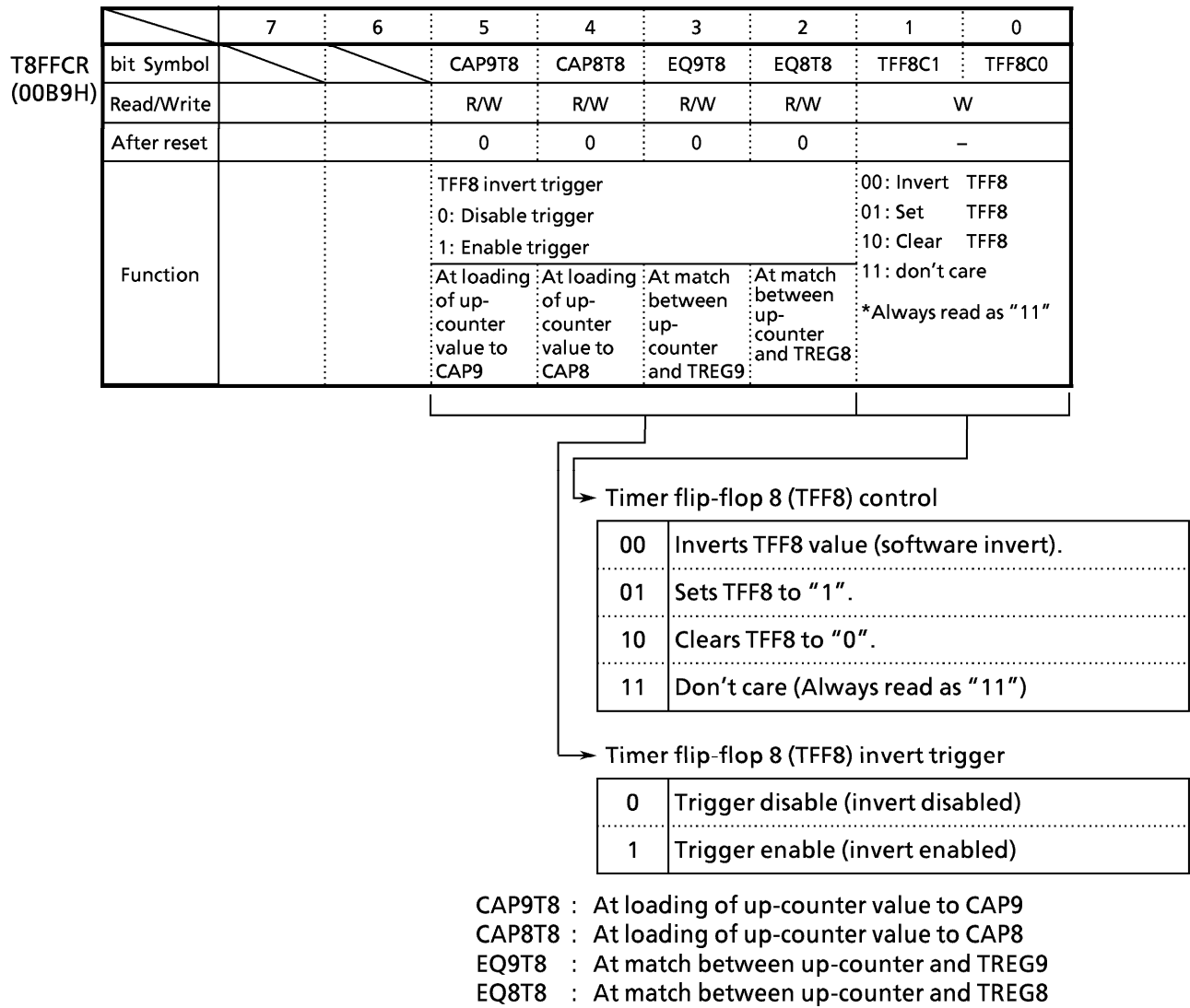
Figure 3.9 (13) 16-Bit Timer 8 F/F Control (T8FFCR)
