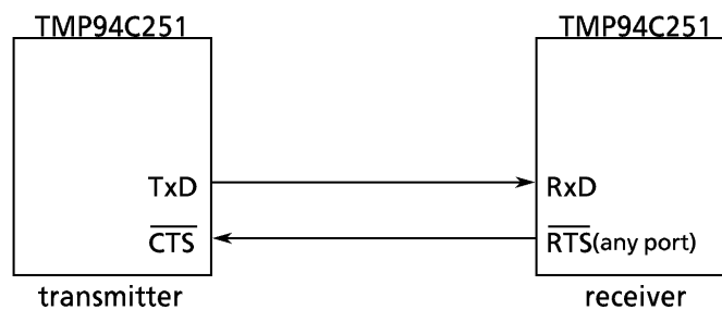
Figure 3.10 (13) Handshake Function
