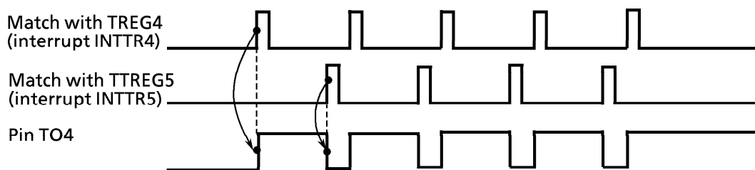
Figure 3.9 (19) Programmable Pulse Generation (PPG) Output Waveform
