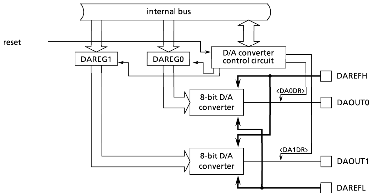
Figure 3.12 (1) D/A Converter Block Diagram
