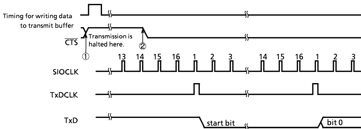
Figure 3.10 (13) Handshake Function
