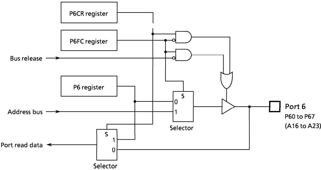
Figure 3.5 (5) Port 6
