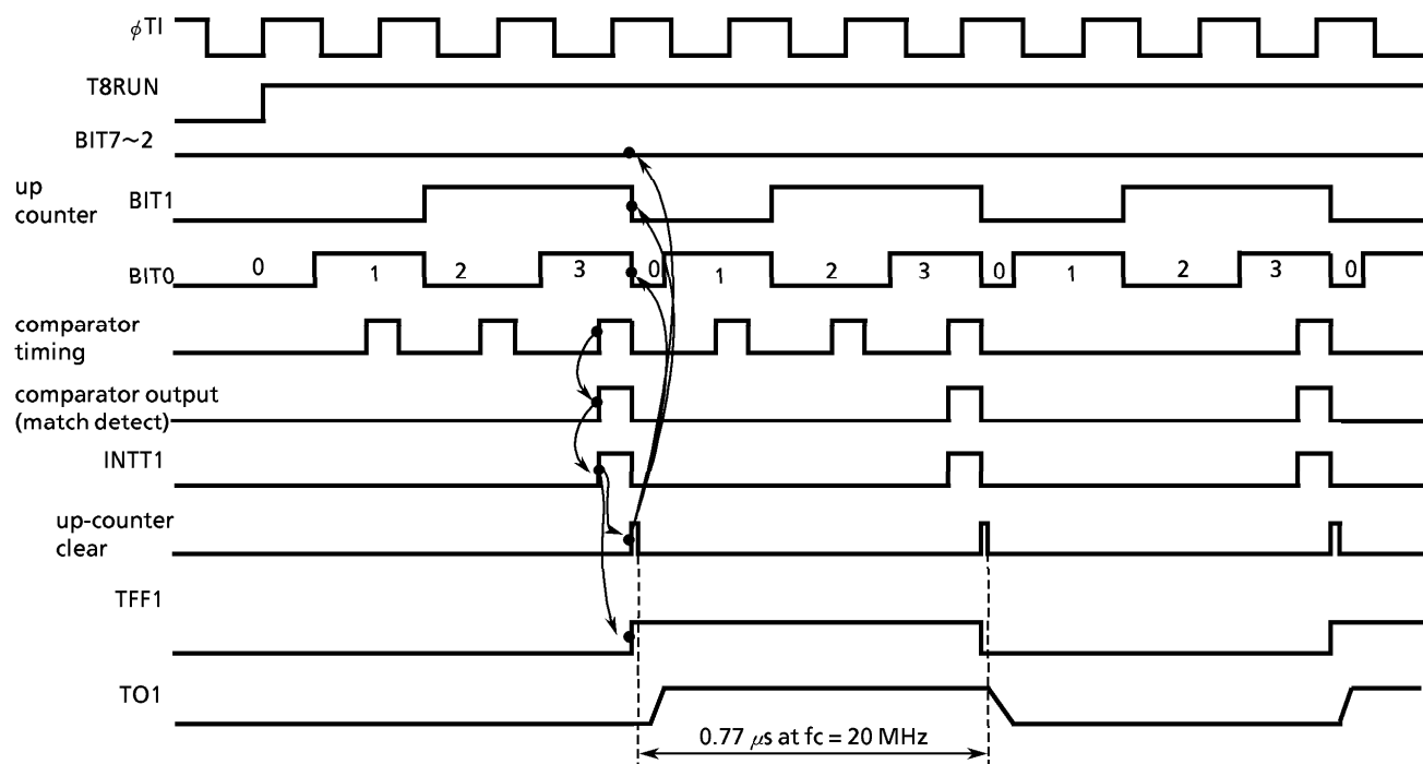
Figure 3.8 (10) Square Wave (50 % Duty) Output Timing Chart
