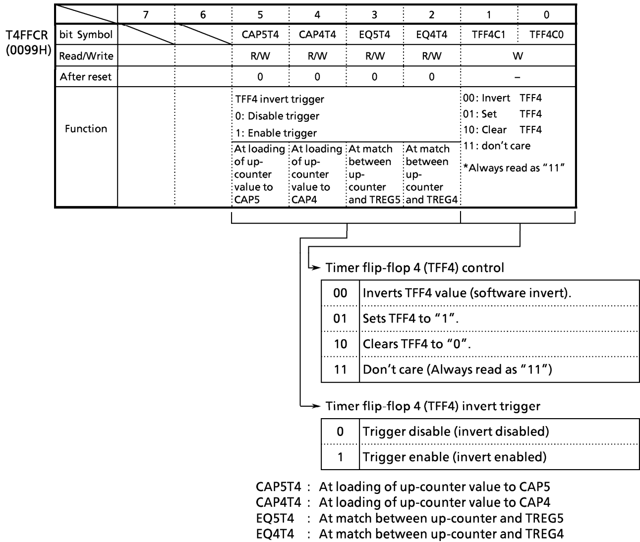
Figure 3.9 (7) 16-Bit Timer 4 F/F Control (T4FFCR)
