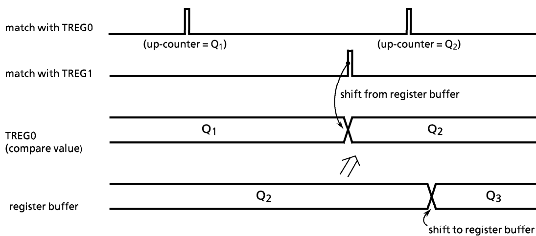
Register Buffer Operation
