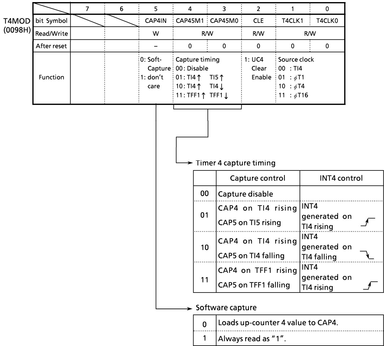
Figure 3.9 (6) 16-Bit Timer Control Register (T4MOD) (2/2)
