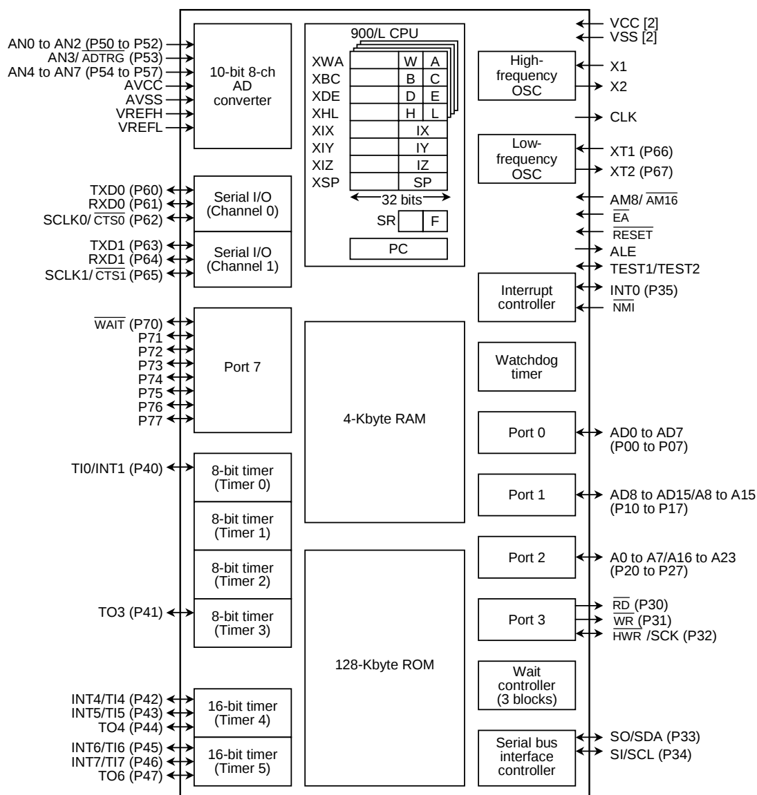
Figure 1.1 TMP93CW44 Block Diagram
