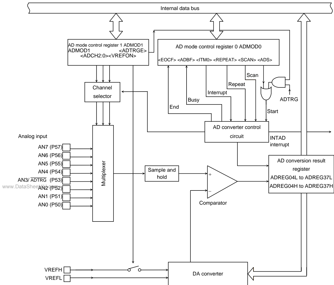
Figure 3.11.1 Block Diagram of AD Converter
