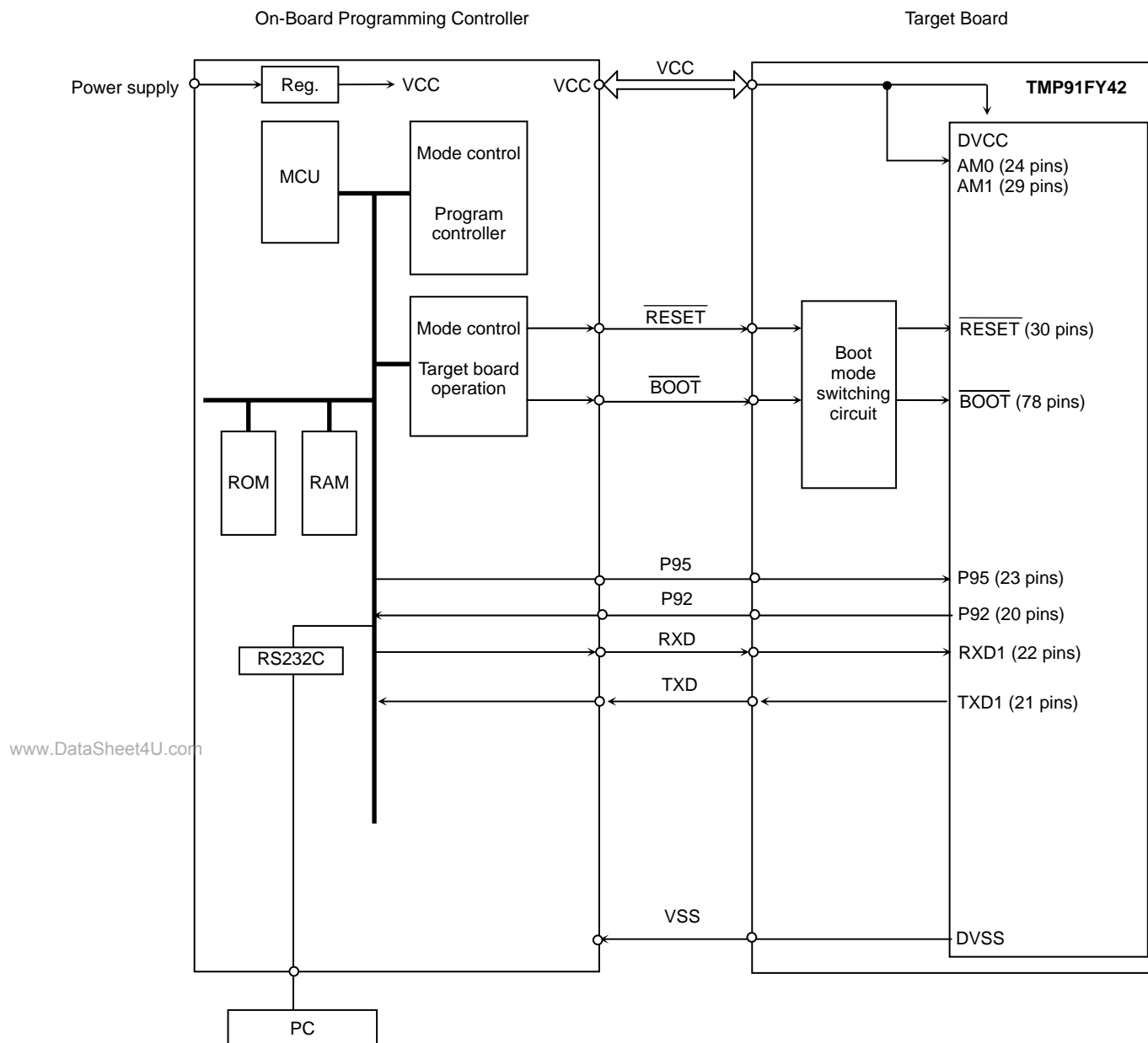
Figure 3.14.4 Example of Connection with an External Controller in Single Boot Mode
