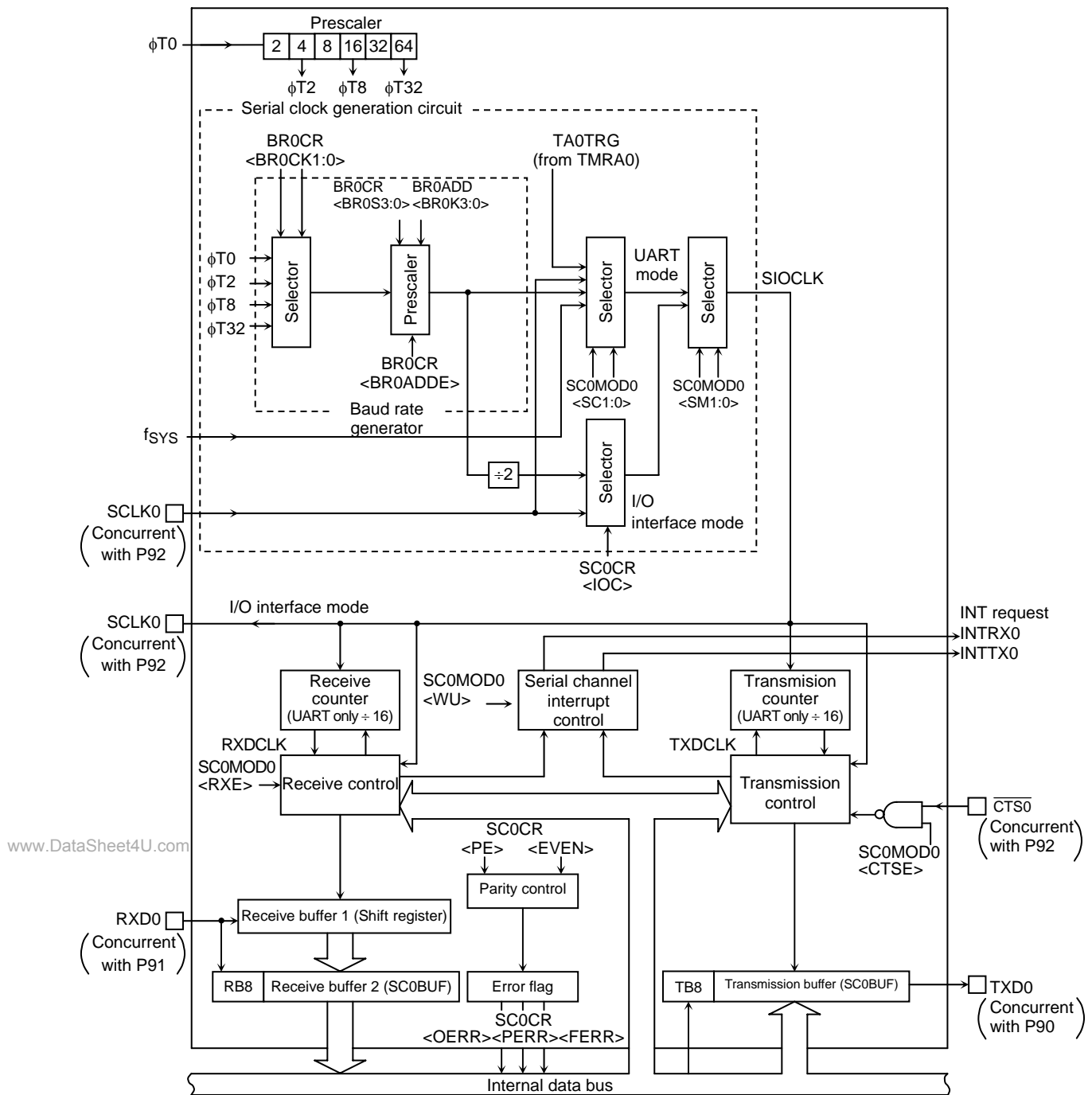
Figure 3.9.2 Block Diagram of the Serial Channel 0 (SIO0)
