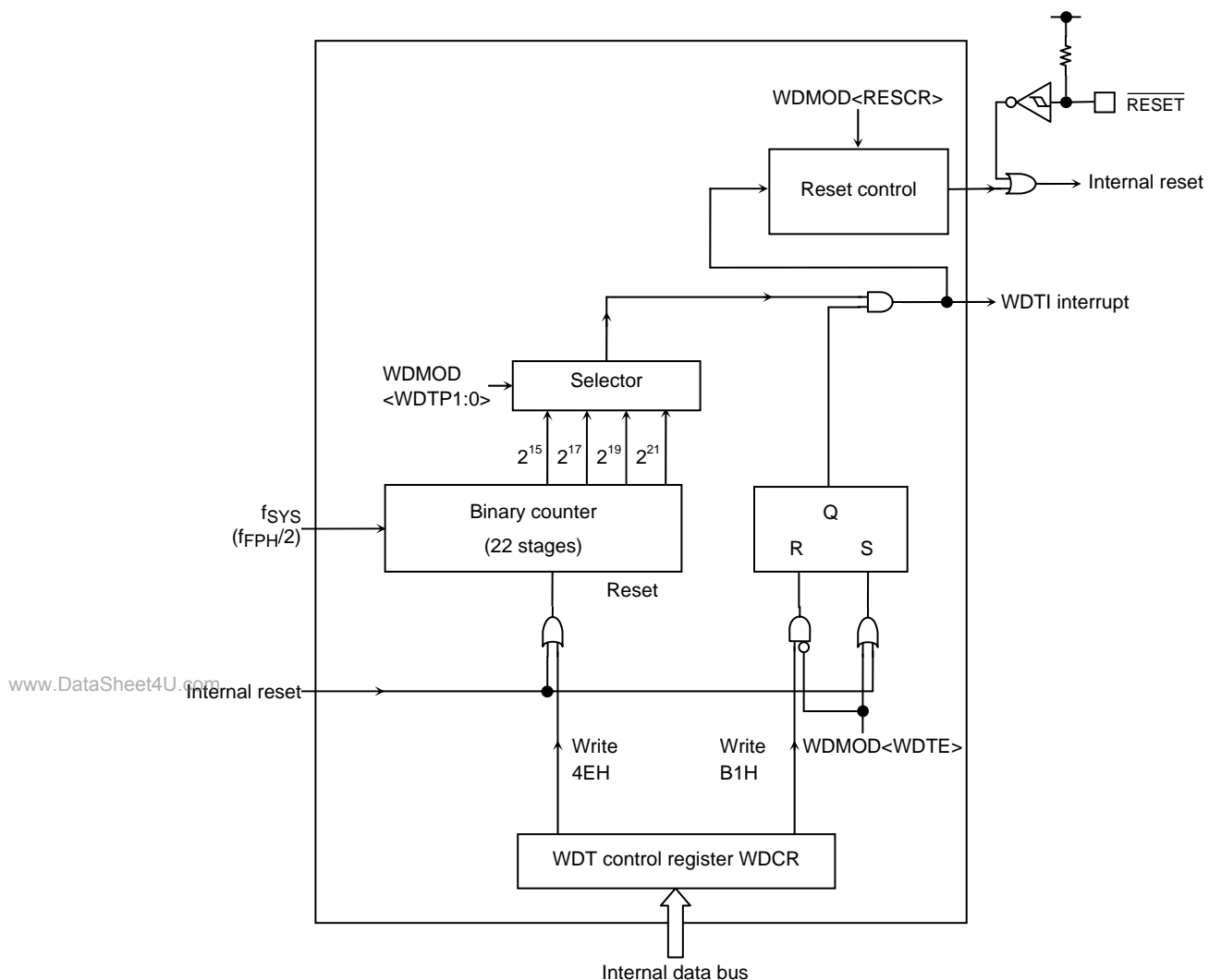
Figure 3.12.1 Block Diagram of Watchdog Timer
