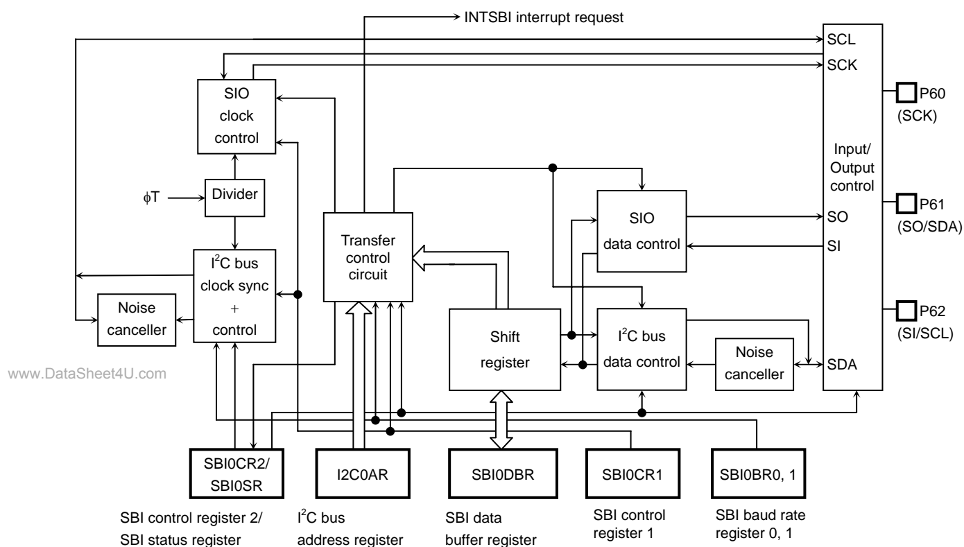
Figure 3.10.1 Serial Bus Interface (SBI)
