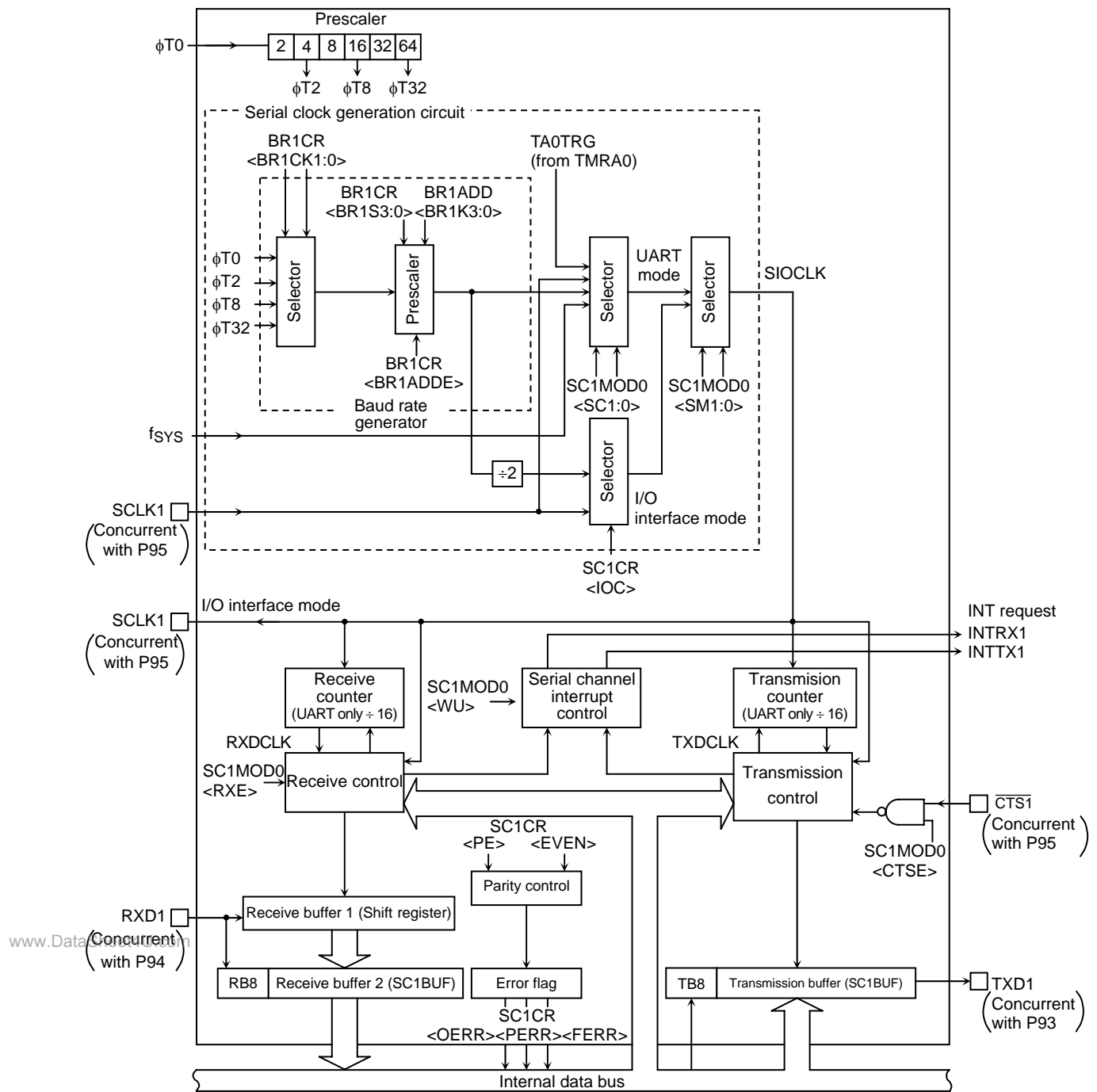
Figure 3.9.3 Block Diagram of the Serial Channel 1 (SIO1)
