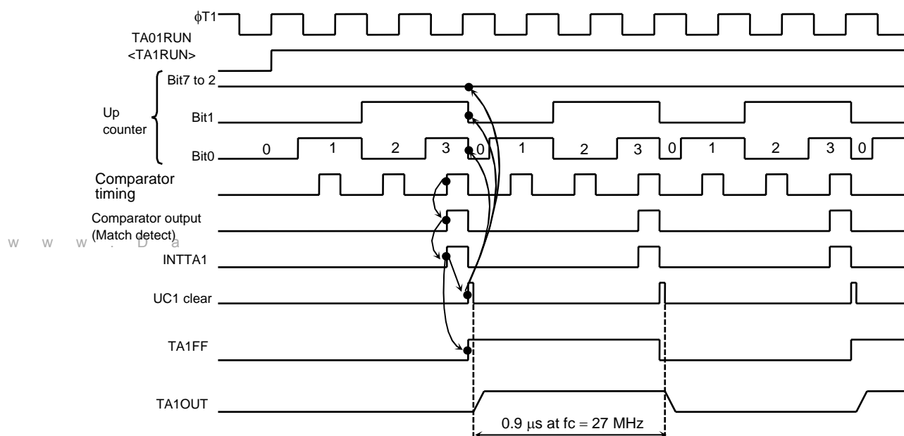
Figure 3.7.17 Square Wave Output Timing Chart (50% duty)
