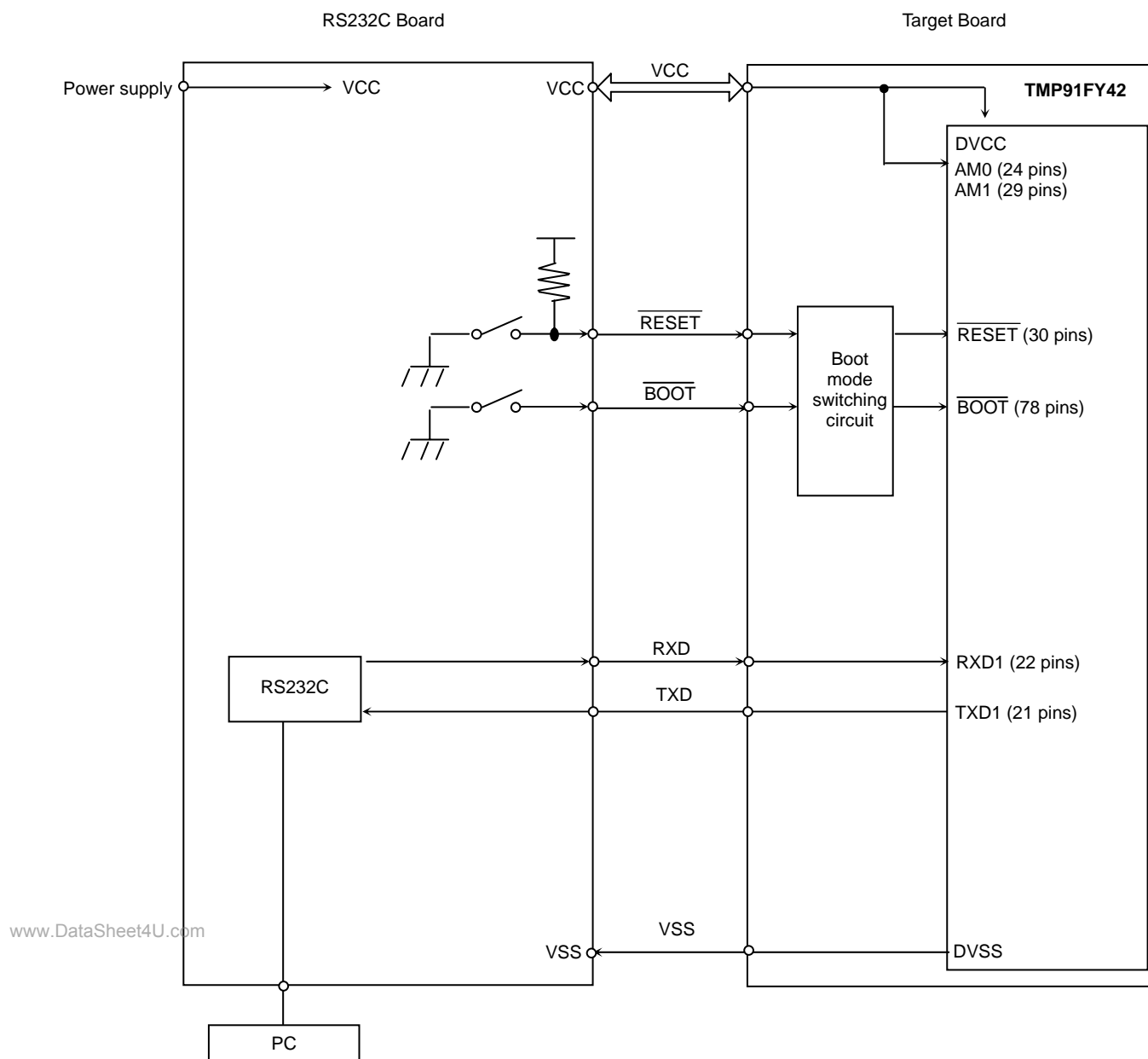
Figure 3.14.5 Example of Connection with an RS232C Board in Single Boot Mode
