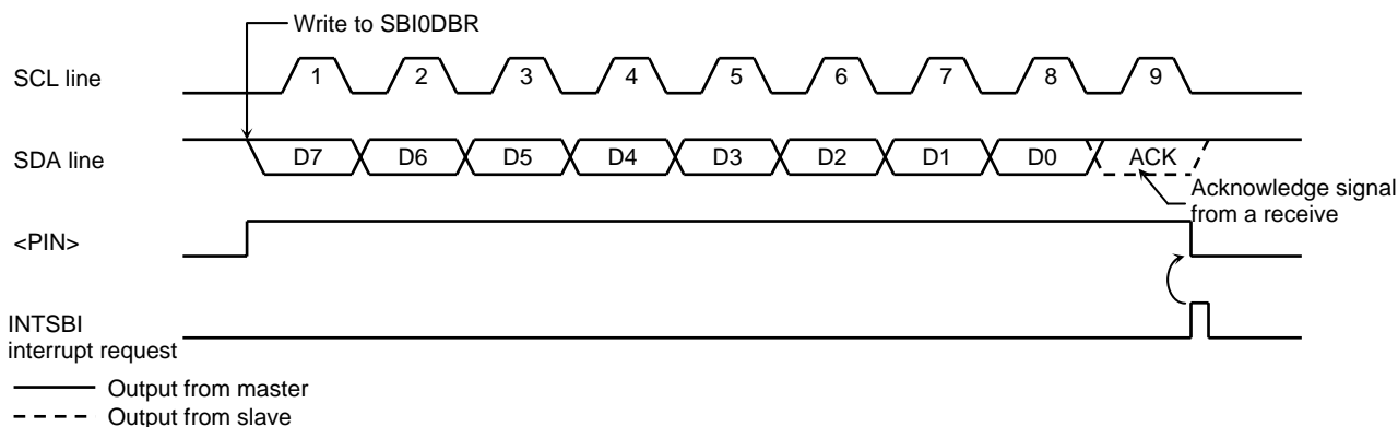
www.DataSheet4U.com Figure 3.10.14 Example in which BC<2:0> = 000 and <ACK> = 1 in Transmitter Mode
