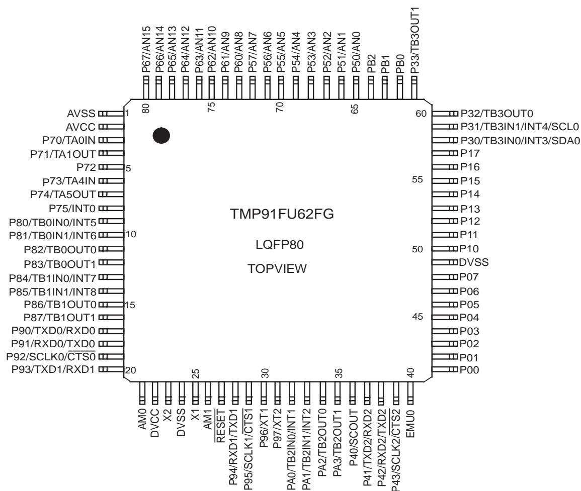
Figure 1-1 Pin Assignment(TMP91FU62FG)
