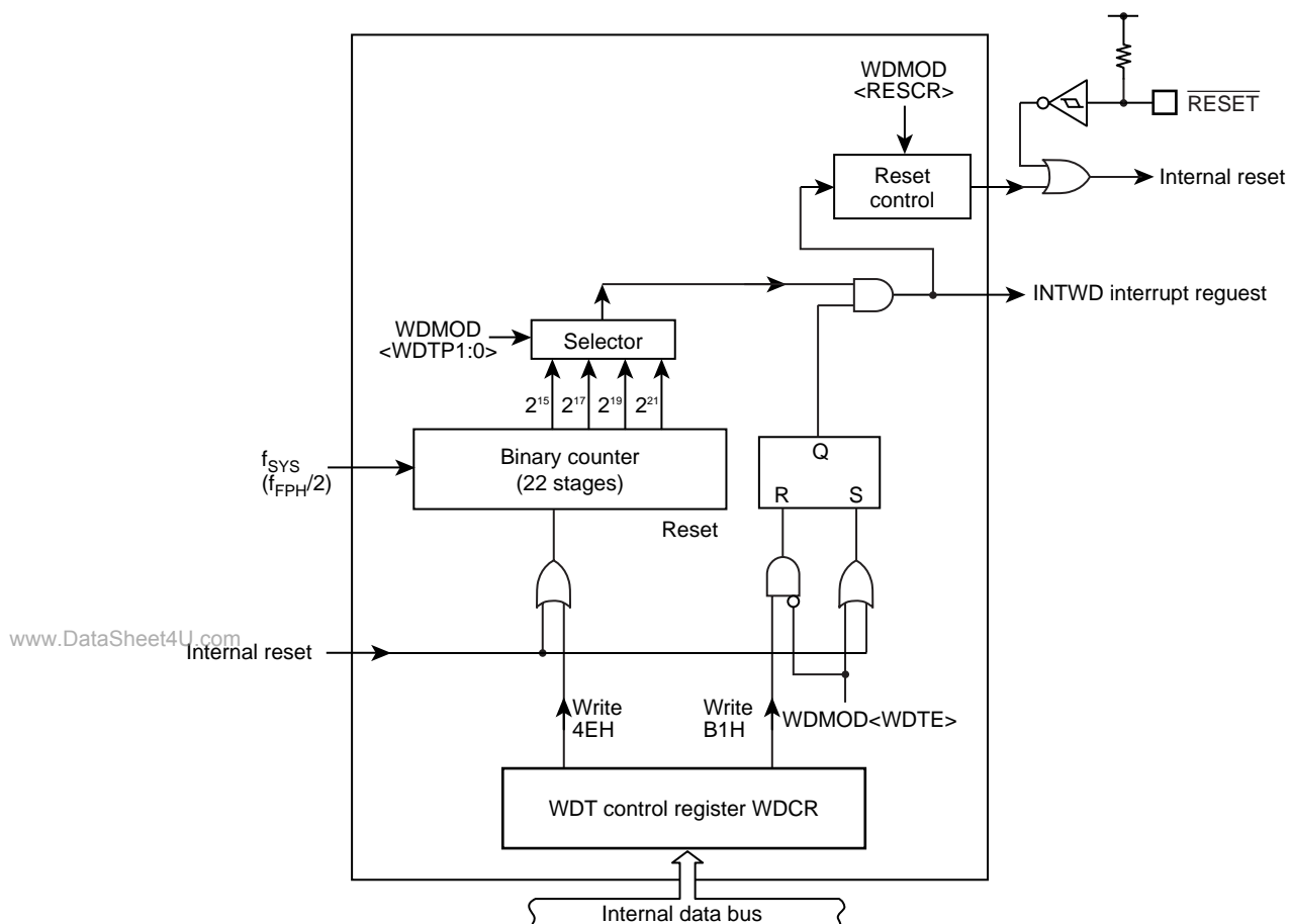
Figure 11-1 Block Diagram of Watchdog Timer
