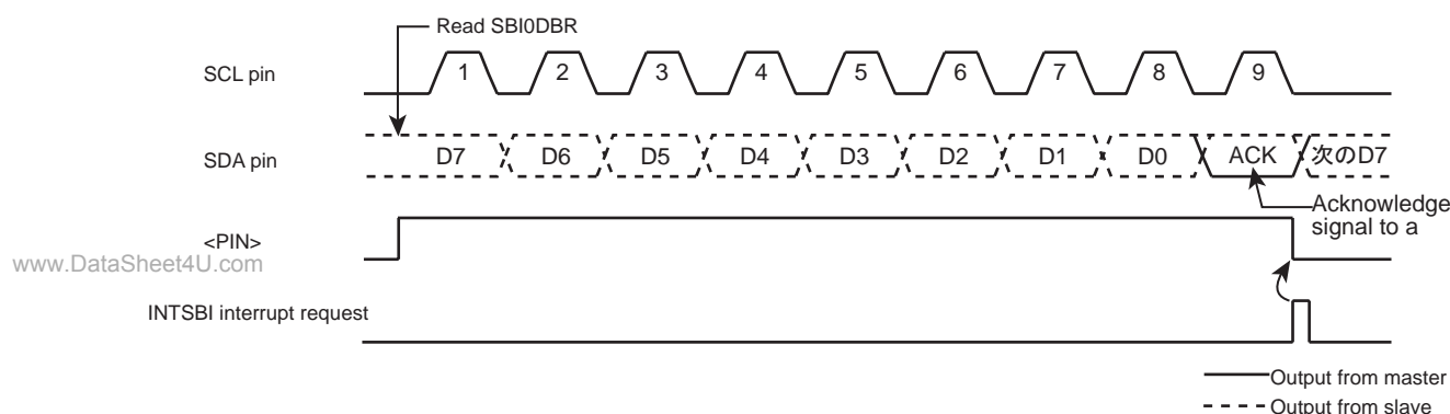
Figure 8-11 Example of when \langle BC2:0 \rangle = "000" , \langle ACK \rangle = "1" in Receiver Mode
