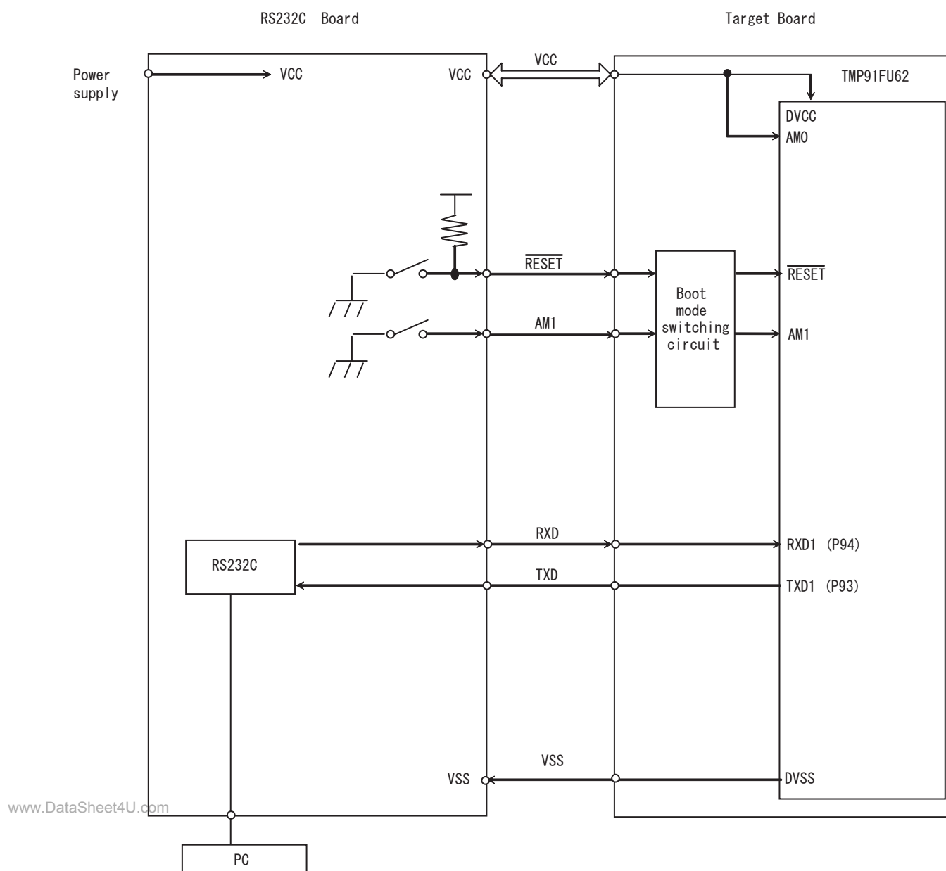
Figure 13-5 Example of Connection with an RS232C Board in Single Boot Mode
