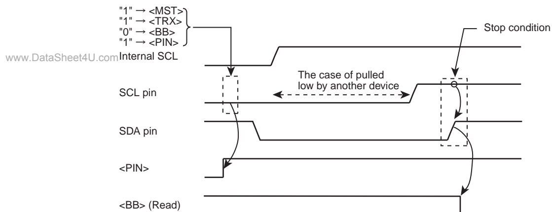
Figure 8-14 Condition Generation (Multi master)
