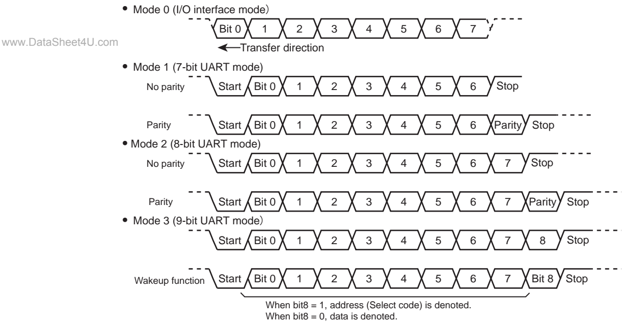
Figure 7-1 Data Formats
