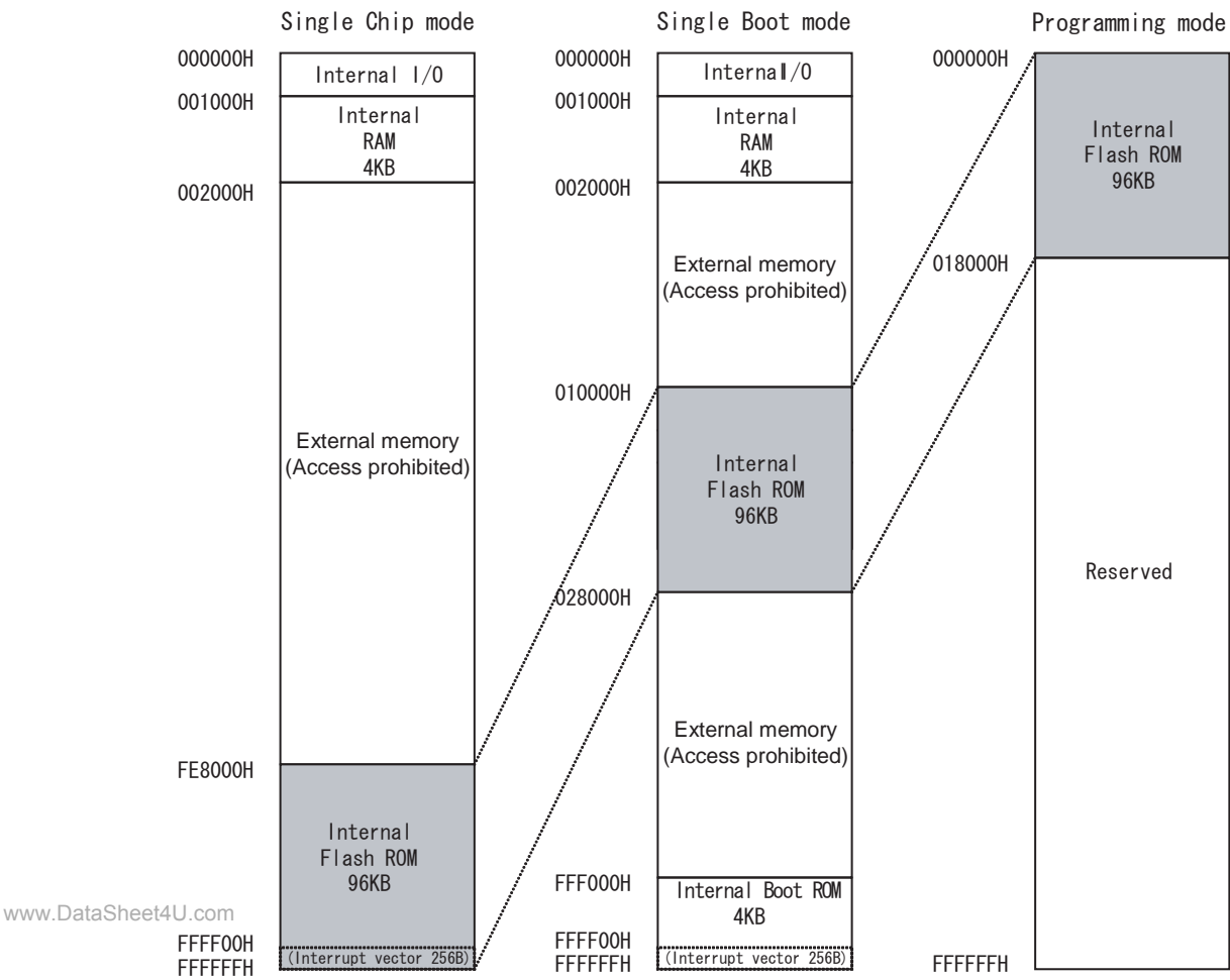
Figure 13-3 Memory Map for Each Operation Mode
