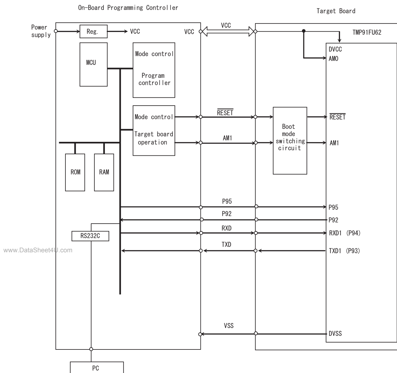
Figure 13-4 Example of Connection with an External Controller in Single Boot Mode
