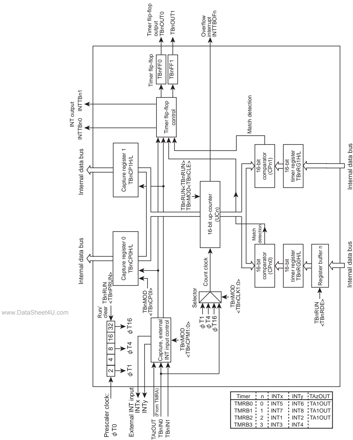
Figure 6-1 Block Diagrams of TMRB0 to TMRB3
