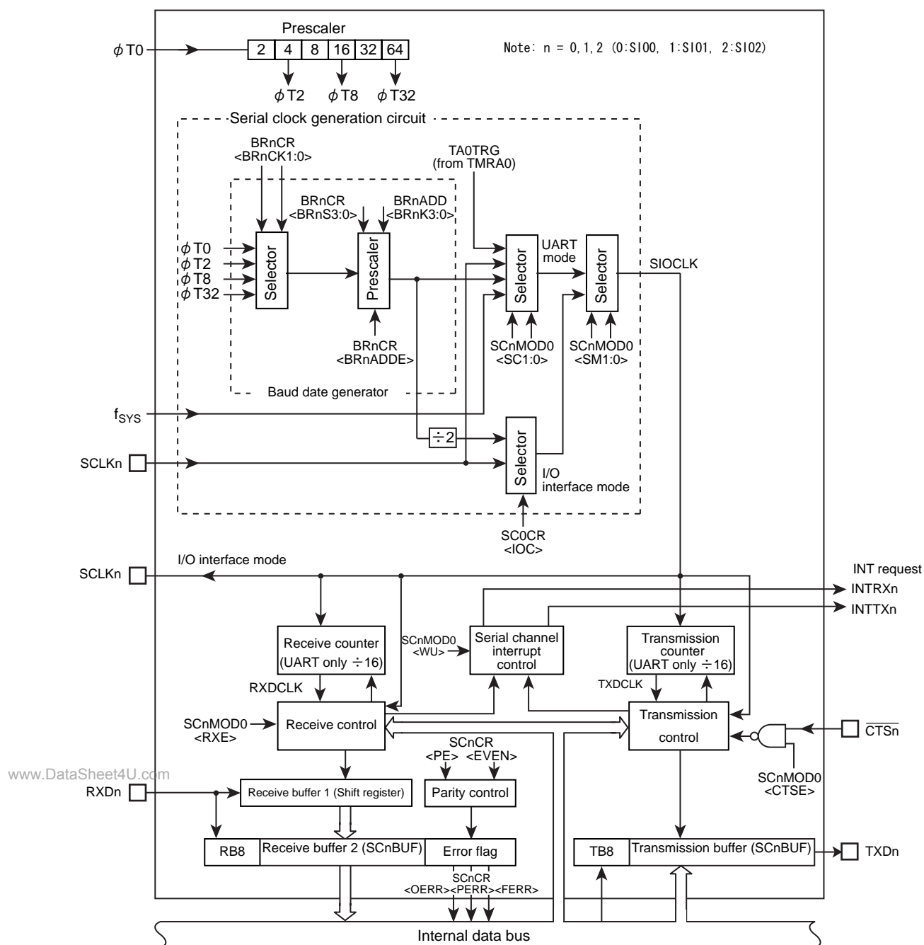
Figure 7-2 Block Diagram of the Serial Channel 0/1/2
