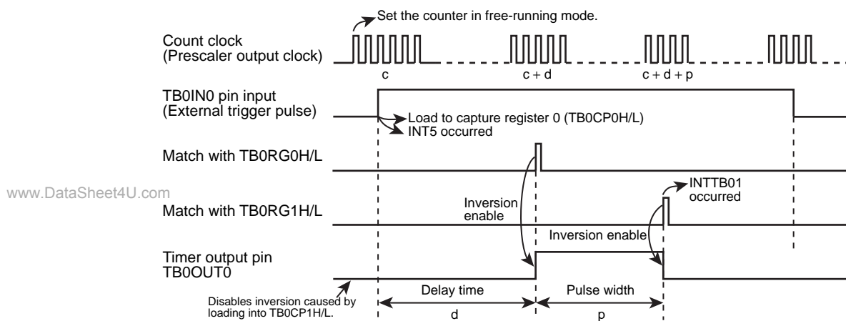
Figure 6-5 One-shot Pulse Output (with delay)
