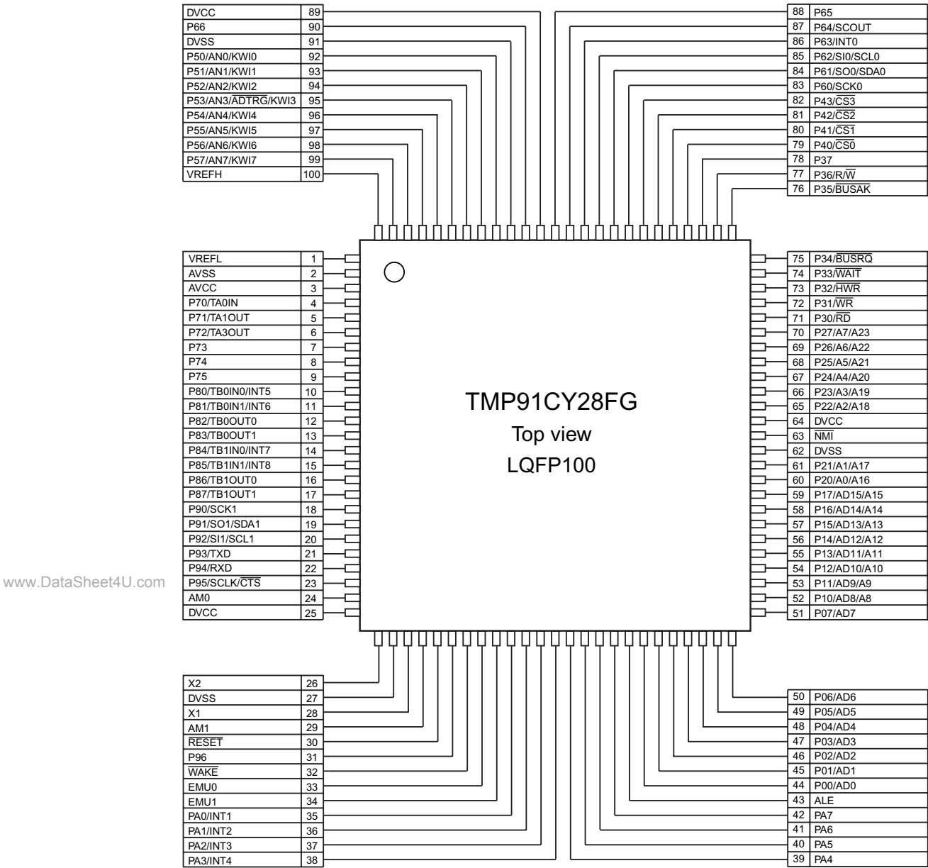
Figure 2.1.1 100-Pin LQFP Pin Assignment
