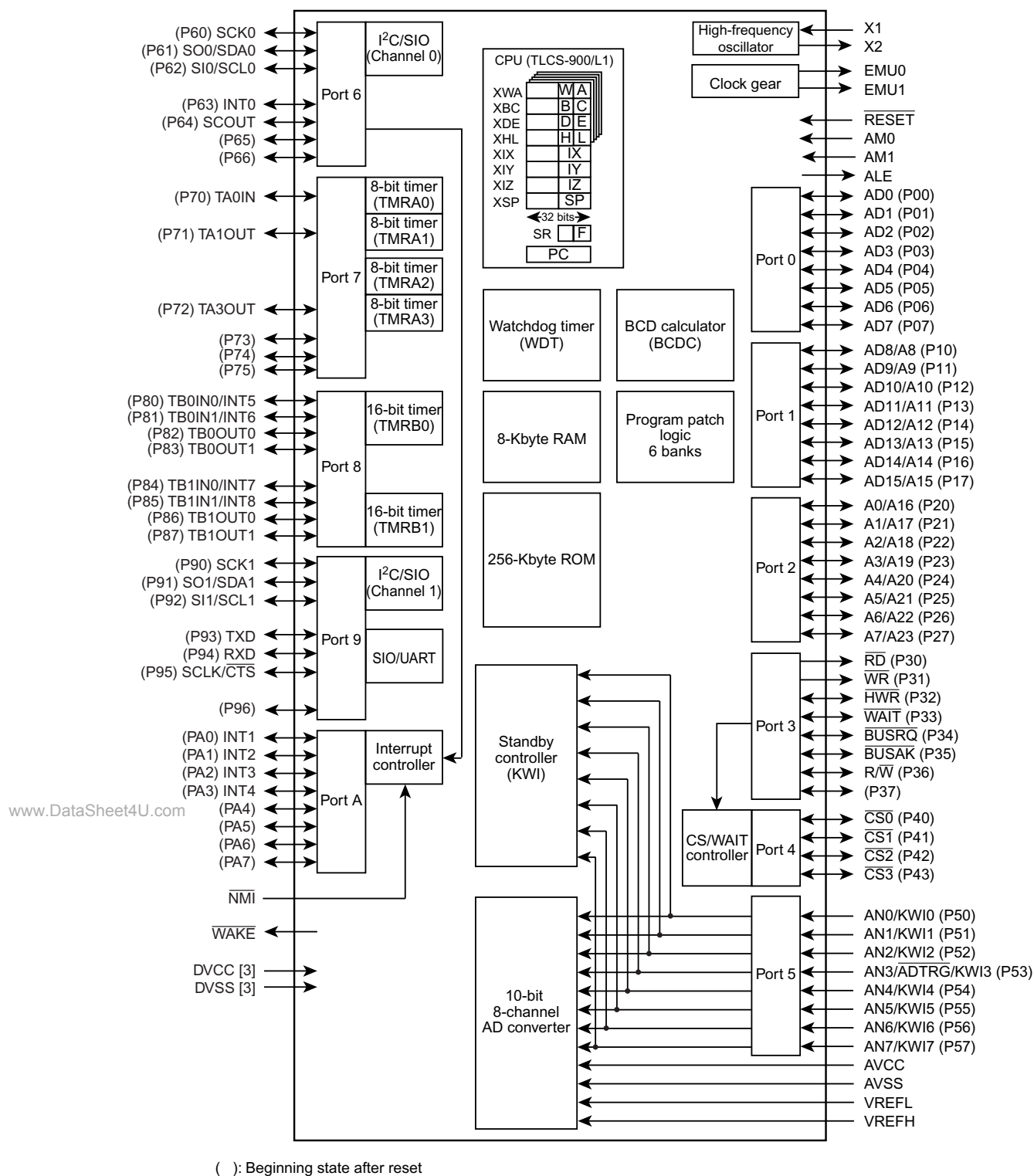
Figure 1.1 TMP91CY28 Block Diagram
