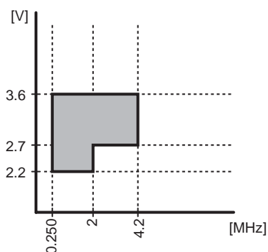
Gear clock(fcgck) frequency range
