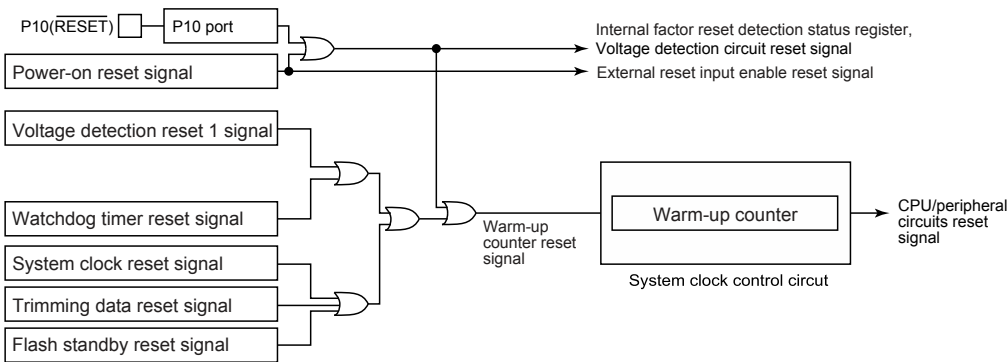
Figure 2-16 Reset Control Circuit
