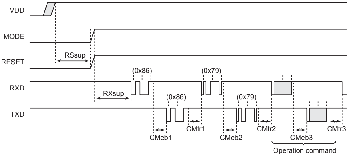
Figure 22-6 Reset Timing
