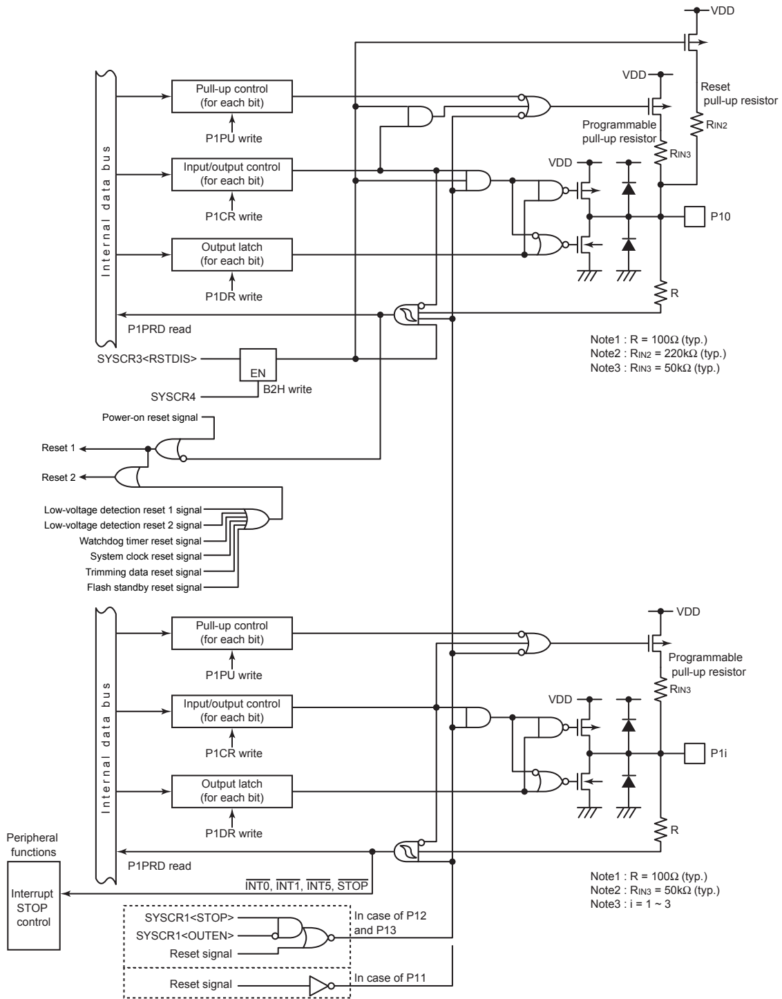
Figure 8-4 Port P1
