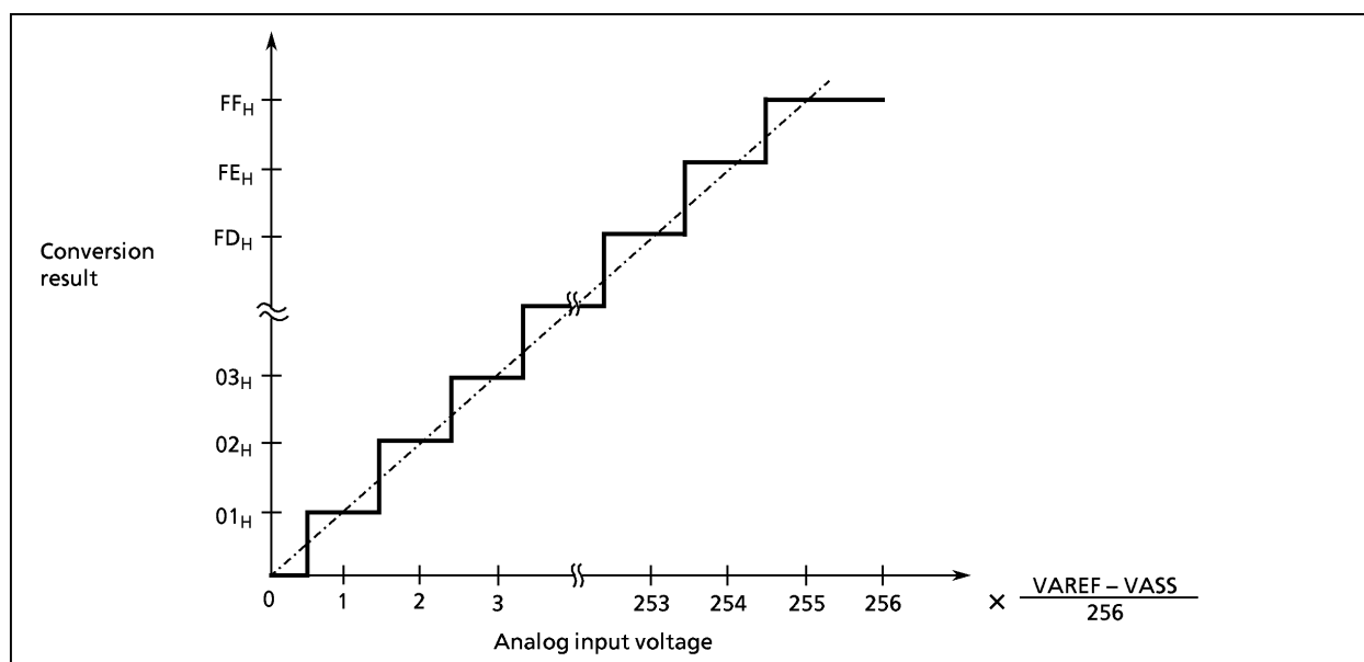
Figure2-79. Analog Input Voltage vs AD Conversion Result (typ.)
