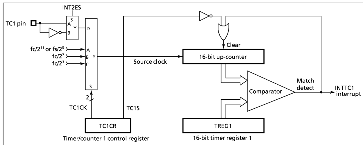
Figure 2-16. Timer/Couter 1
