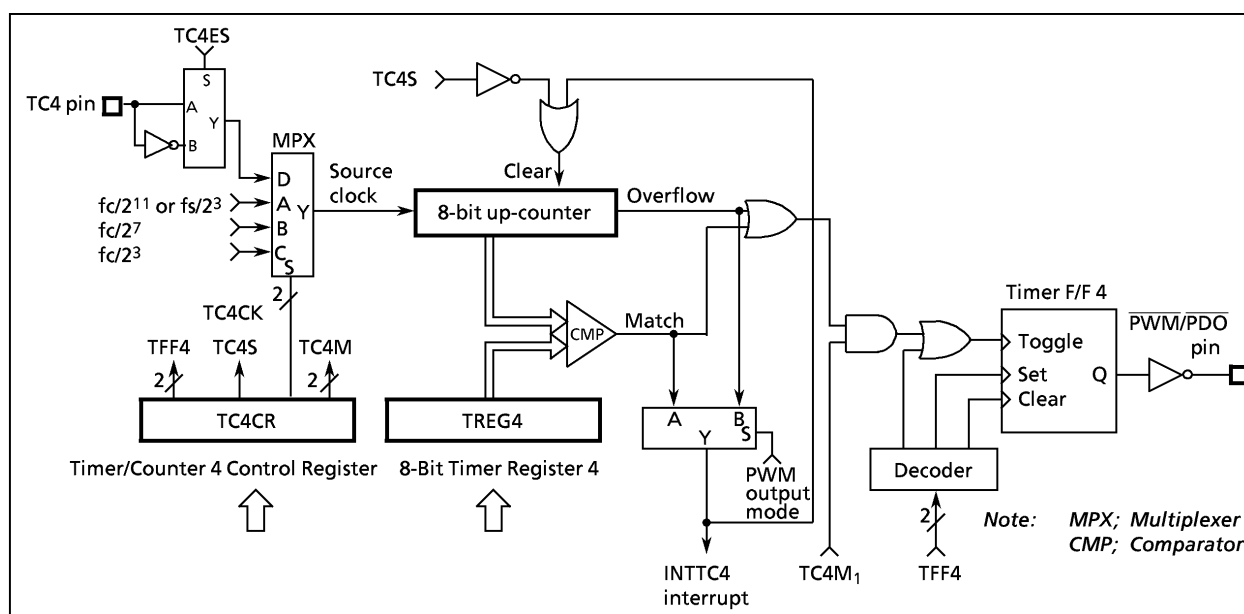
Figure 2-25. Timer/Counter 4
