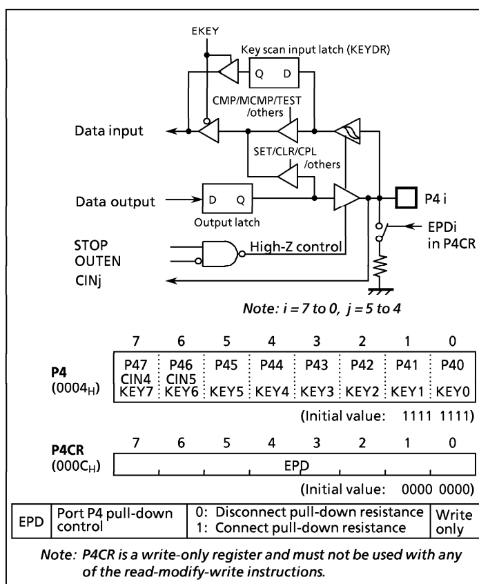
Figure 2-7. Port P4
