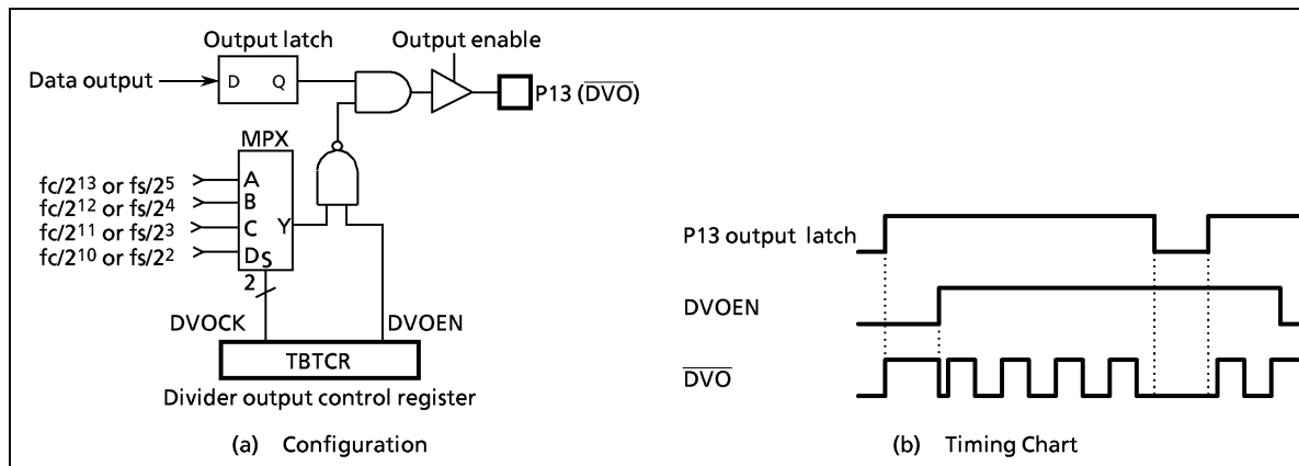
Figure 2-15. Divider Output
