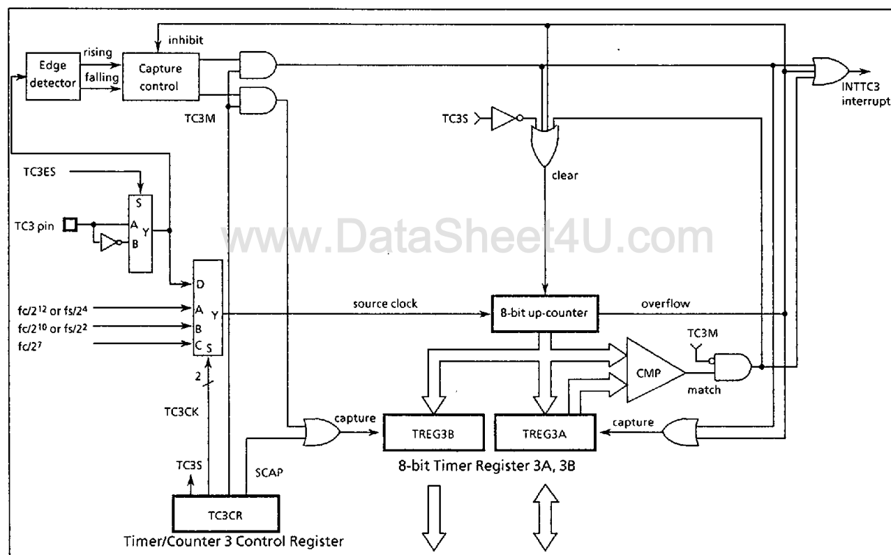
Figure 2-27. Timer / Counter 3
