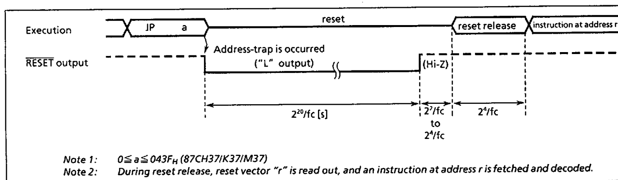
Figure 1-32. Address-Trap-Reset
