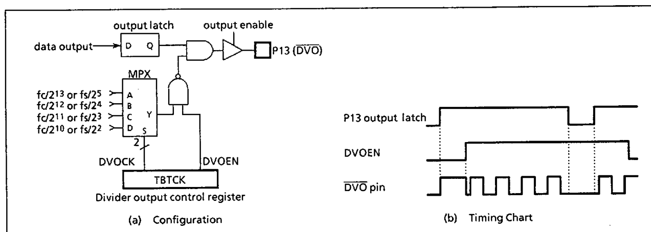
Figure 2-14. Divider Output
