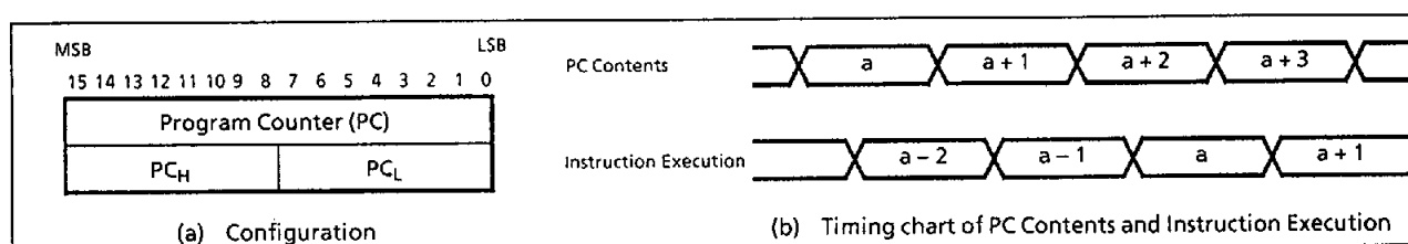
Figure 1-4. Program Counter
