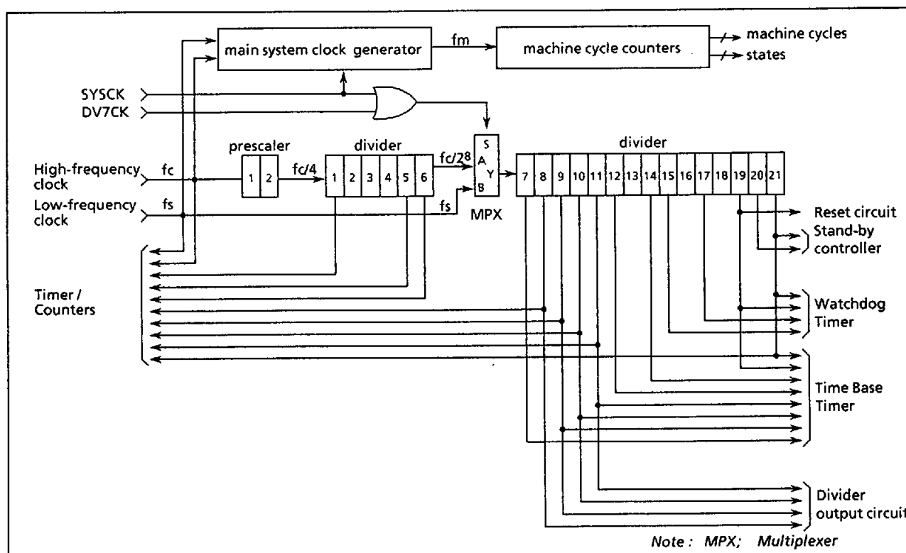
Figure 1-12. Configuration of Timing Generator
