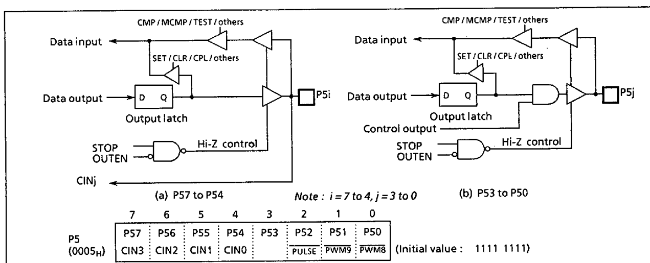
Figure 2-8. Port P5
