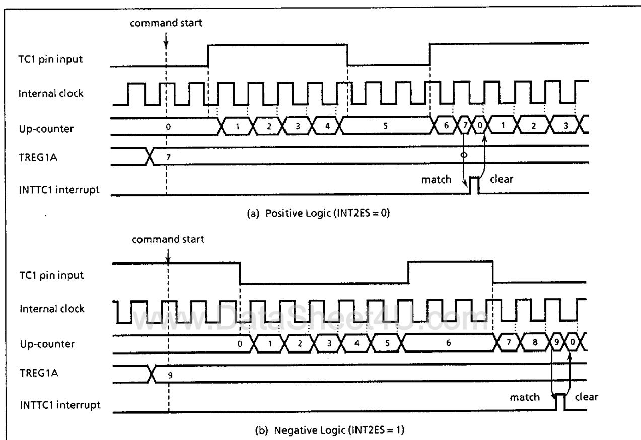
Figure 2-20. Window Mode Timing Chart
