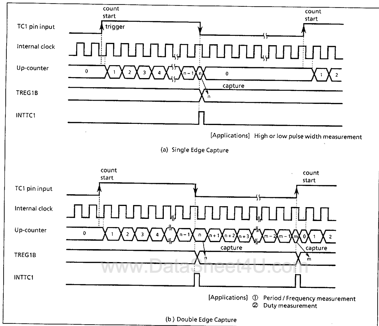
Figure 2-21. Pulse Width Measurement Mode Timing Chart
