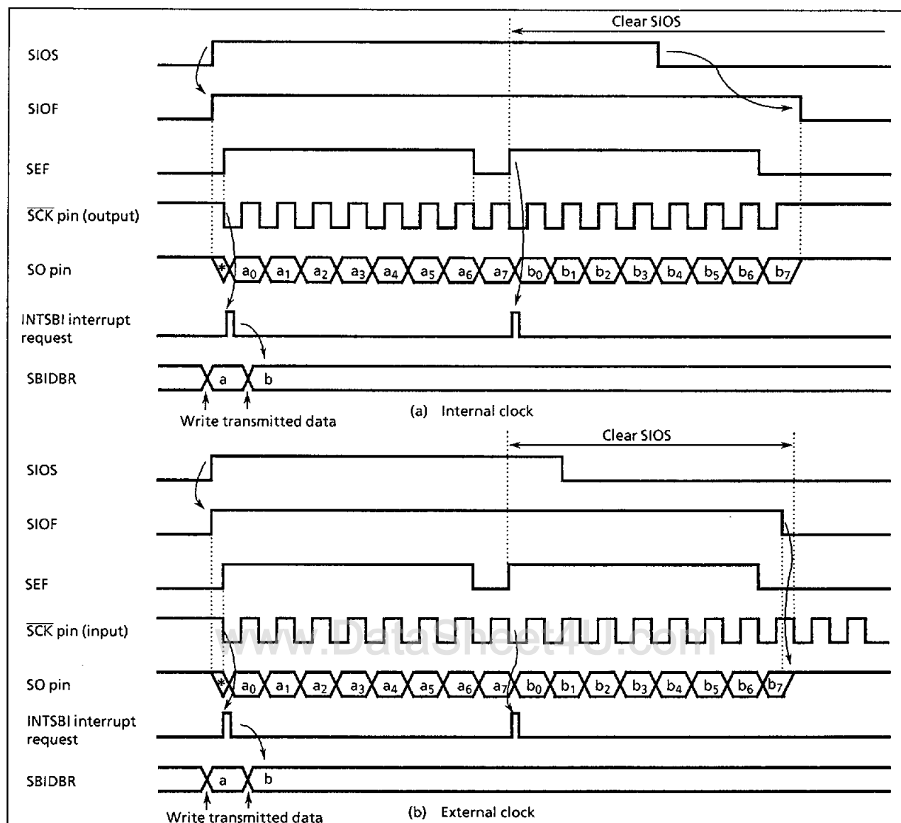
Figure 2-53. Transfer Mode
