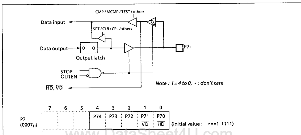
Figure 2-10. Port P7
