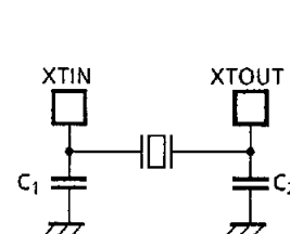
(3) Low-frequency Oscillation
