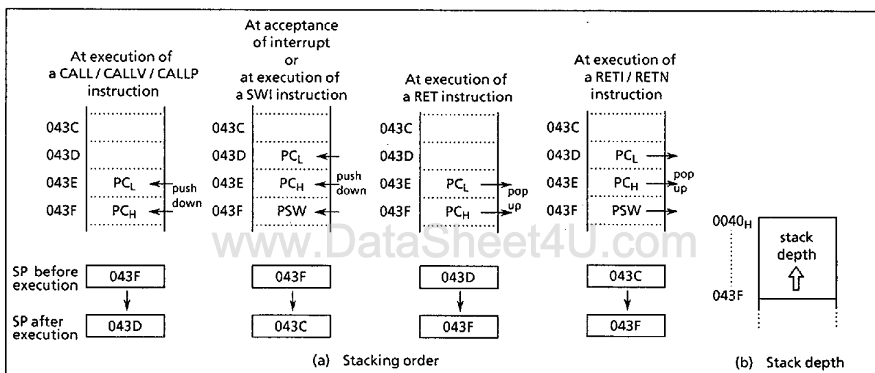
Figure 1-9. Stack
