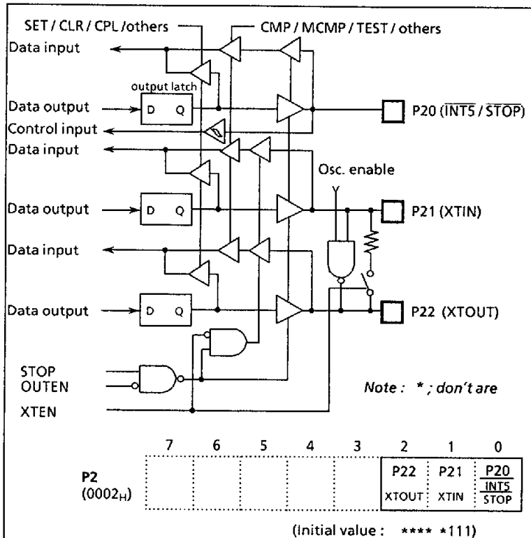
Figure 2-5. Port P2
