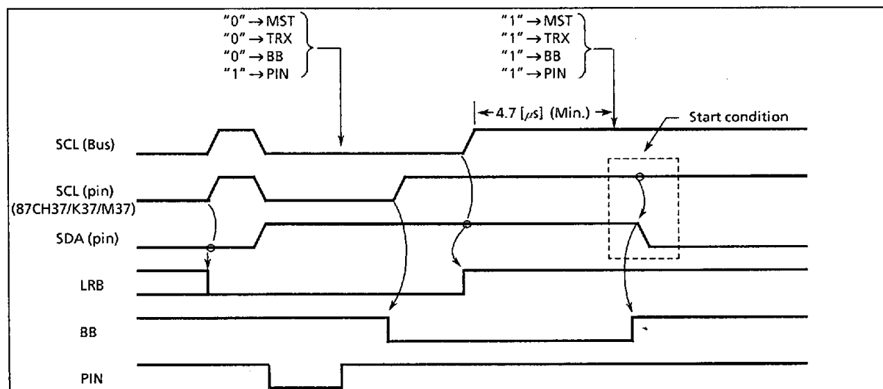
Figure 2-47. Timing Diagram when Restarting the 87CH37/K37/M37
