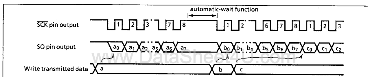
Figure 2-50. Automatic-wait Function
