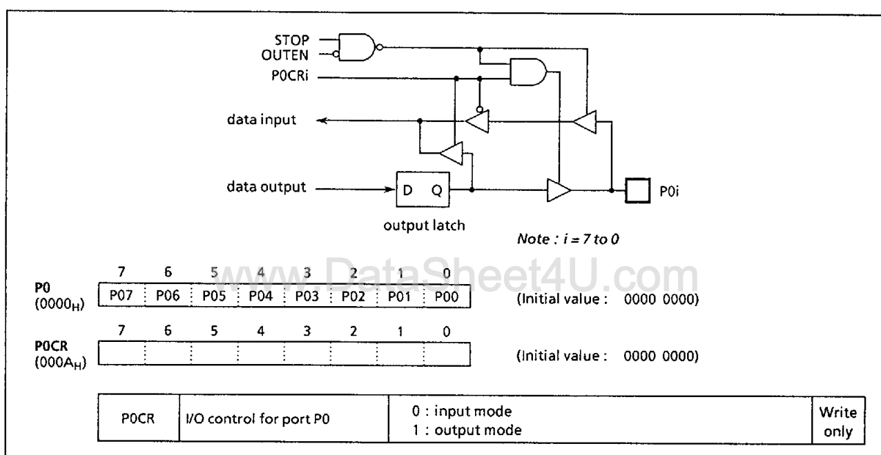
Figure 2-3. Port P0 and P0CR
