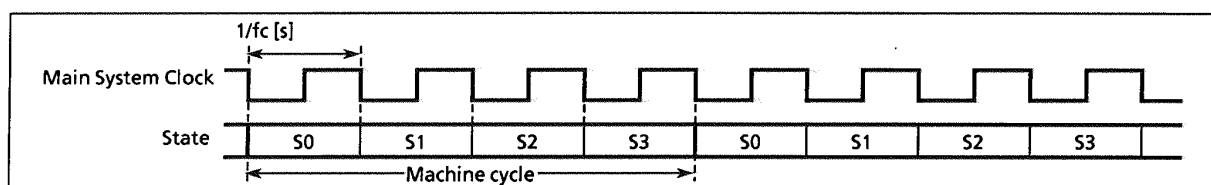
Figure 1-12. Machine cycle
