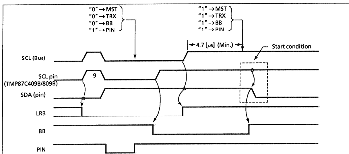
Figure 2-37. Timing diagram when restarting the TMP87C409B/809B
