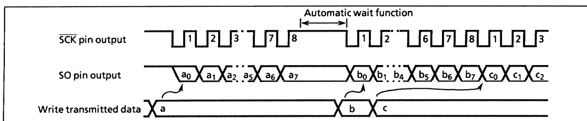
Figure 2-39. Automatic wait function
