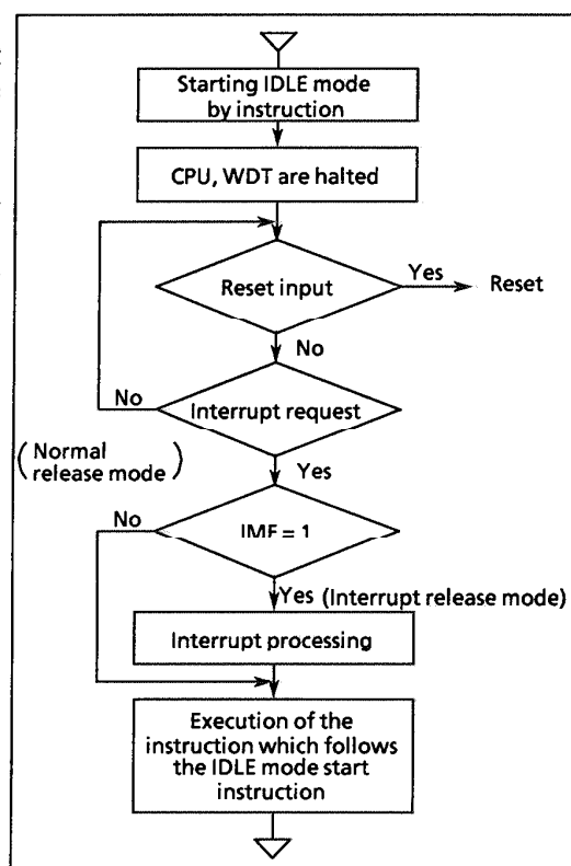
Figure 1-18. IDLE mode
