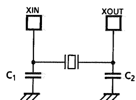
(1) High-frequency Oscillation
