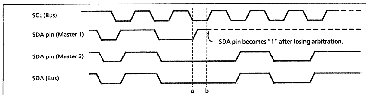
Figure 2-30. Arbitration lost
