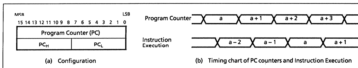
Figure 1-3. Program counter
