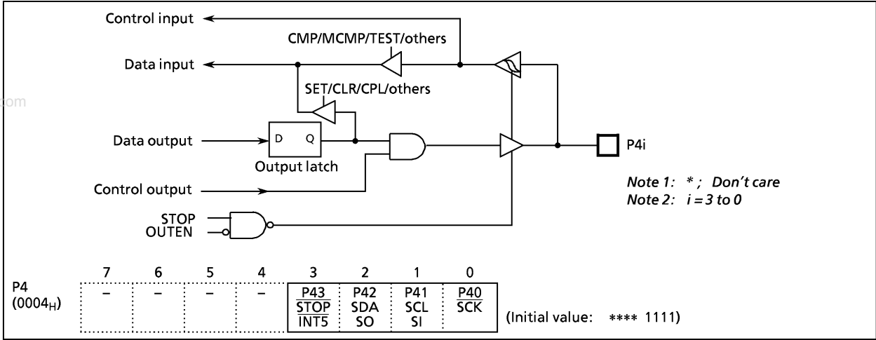
Figure 2-4. Port P4
