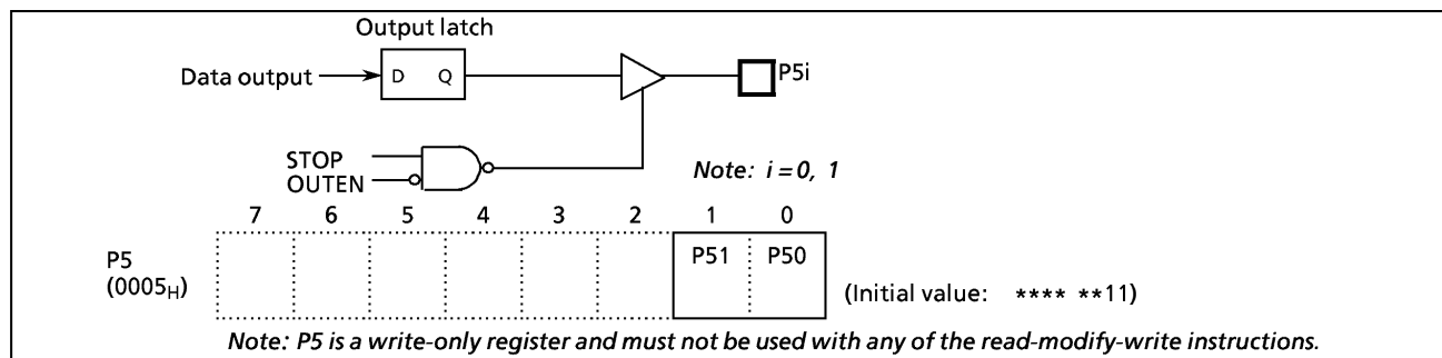
Figure 2-6. Port P5
