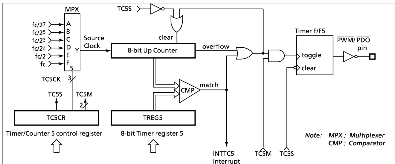
Figure 2-28. Timer/Counter 5 (TC5)
