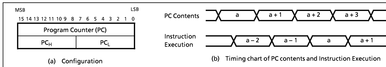
Figure 1-3. Program Counter
