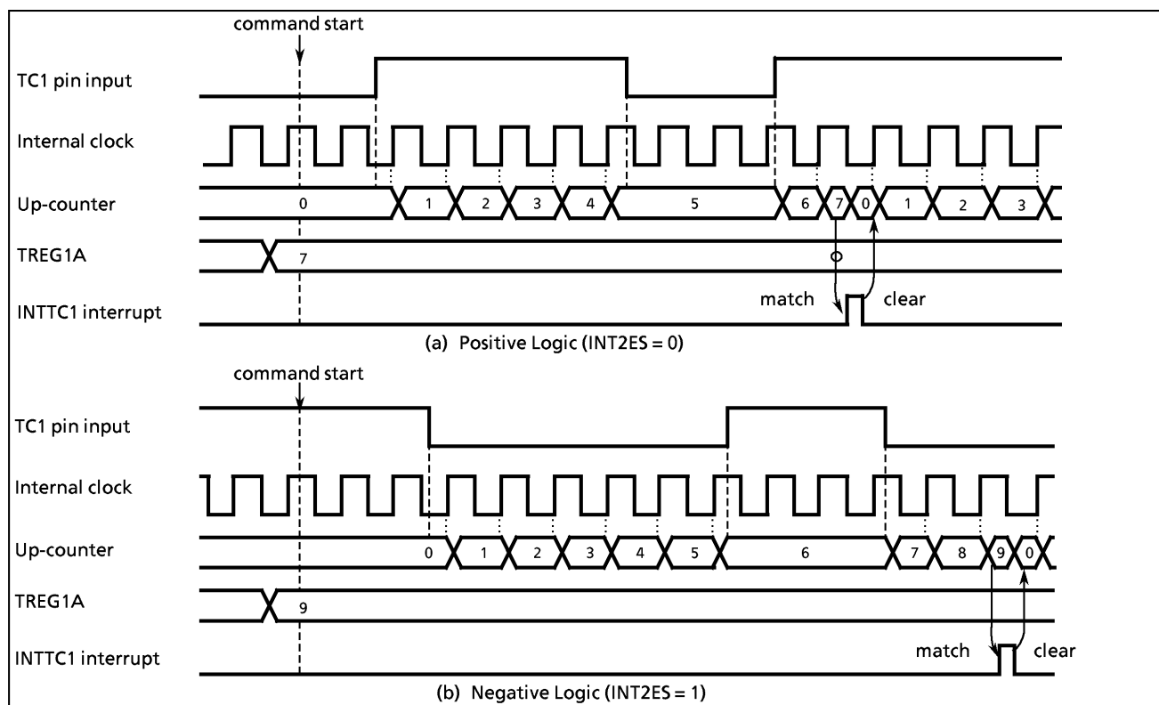
Figure 2-18. Window Mode Timing Chart
