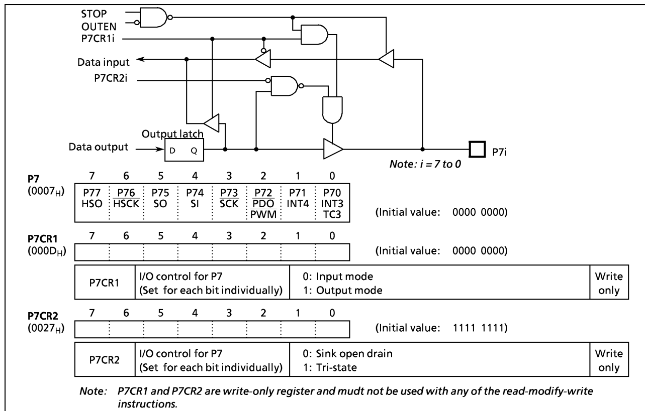
Figure 2-8. Port 7 and P7CR
