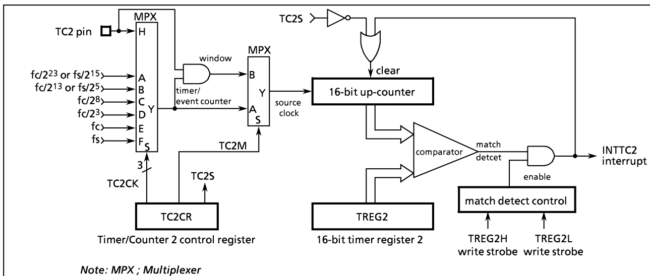
Figure 2-22. Timer/Counter 2 (TC2)
