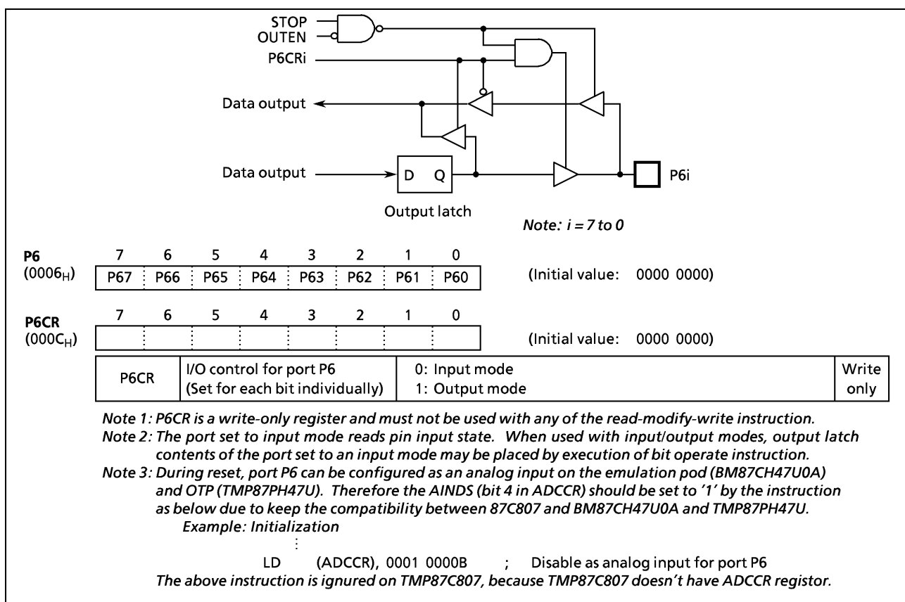
Figure 2-7. Port P6 and P6CR
