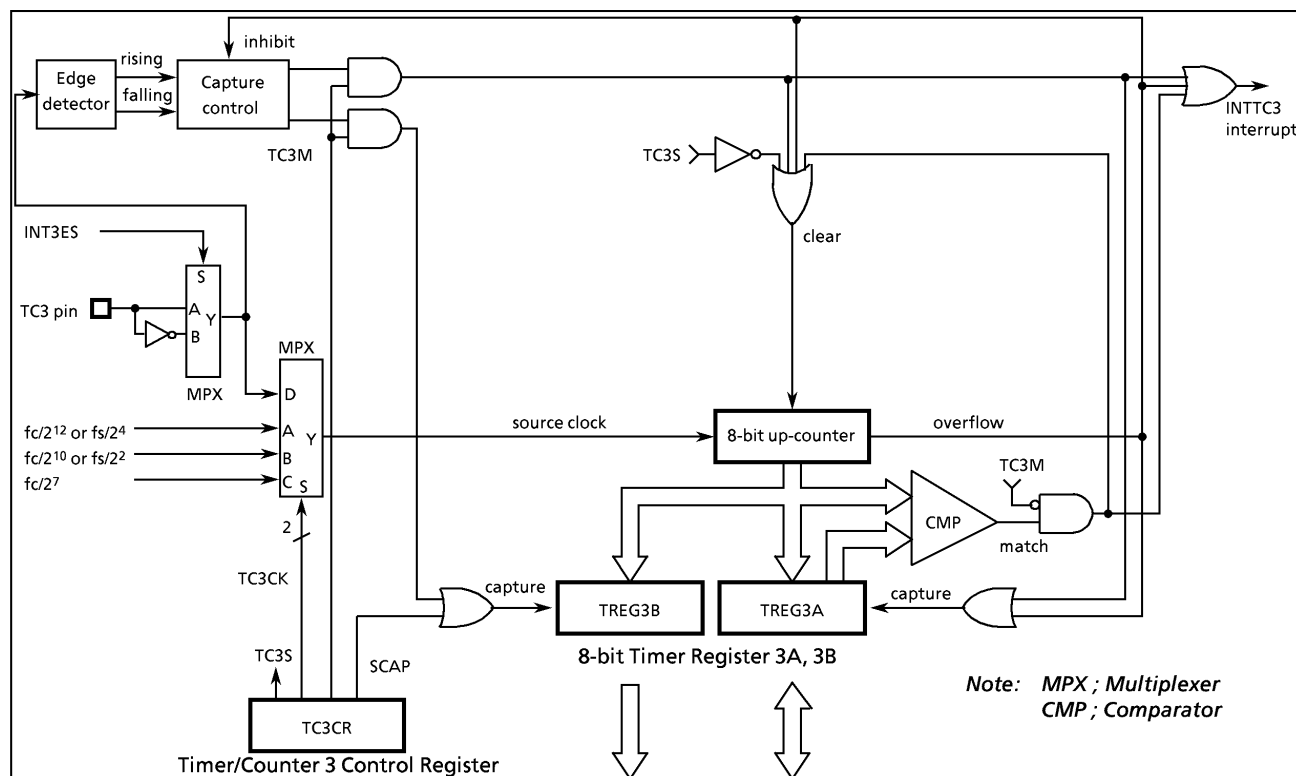
Figure 2-25. Timer/Counter 3 (TC3)
