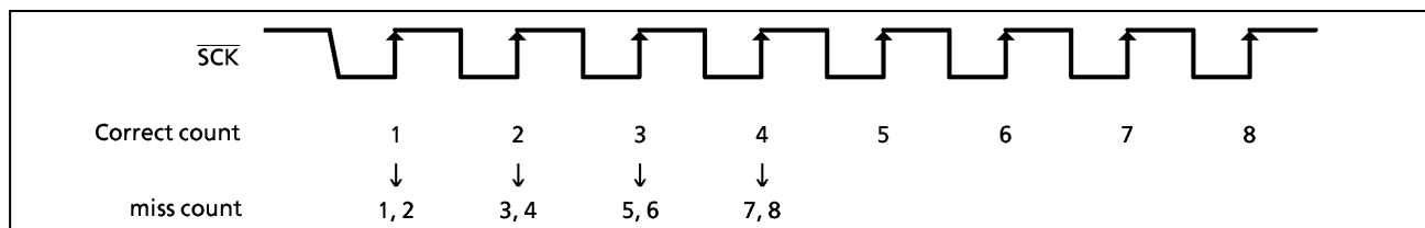
Figure 2-42. Example of miss count (at 8-bit receive mode)
