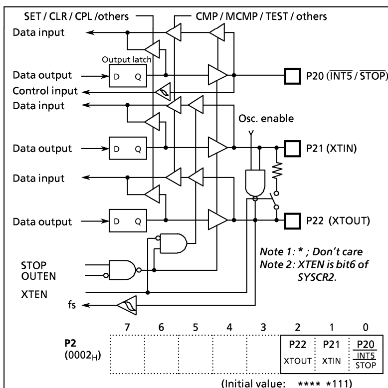
Figure 2-5. Port P2
